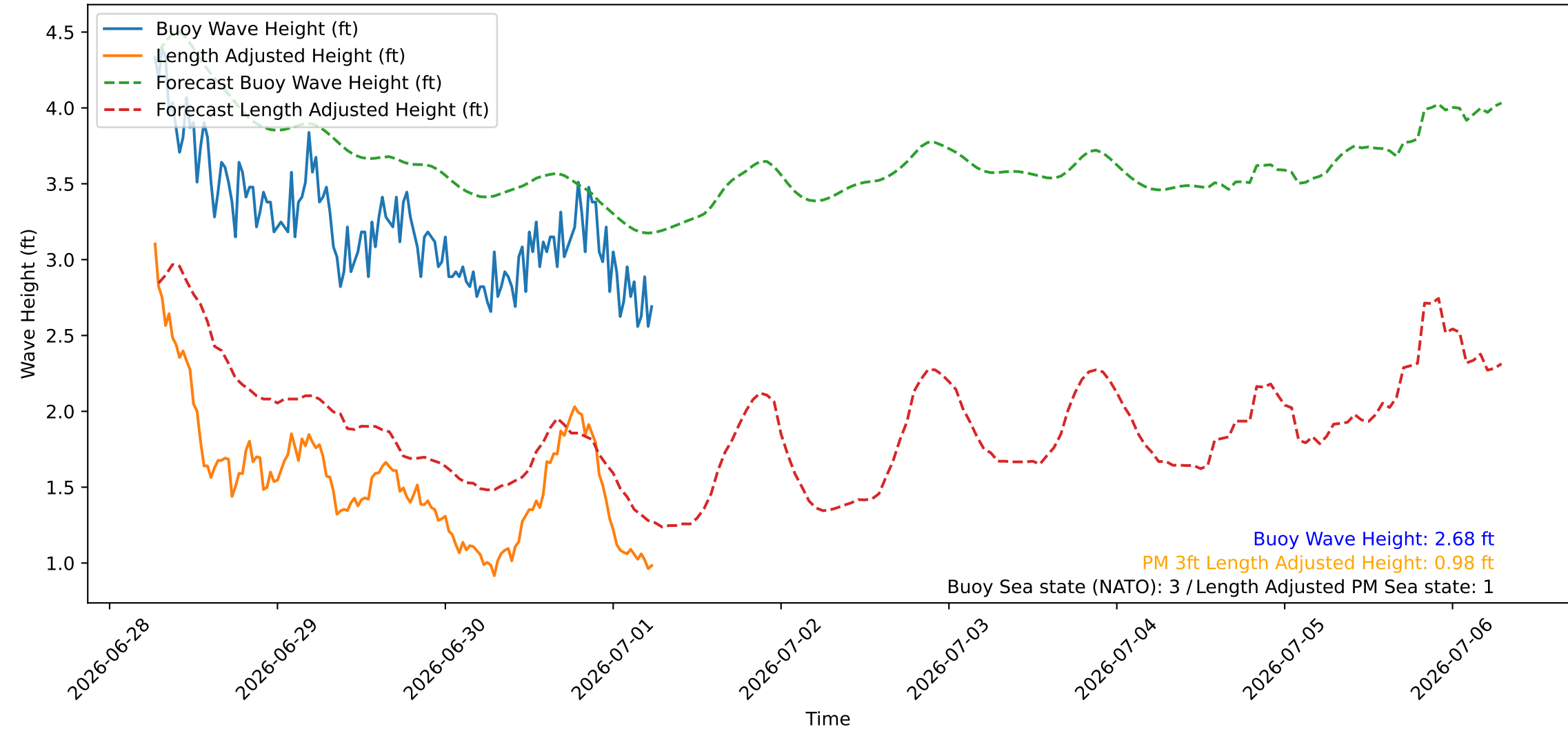
Wave Heights over Time for Green Beach at 2026-07-01 06:31:08
