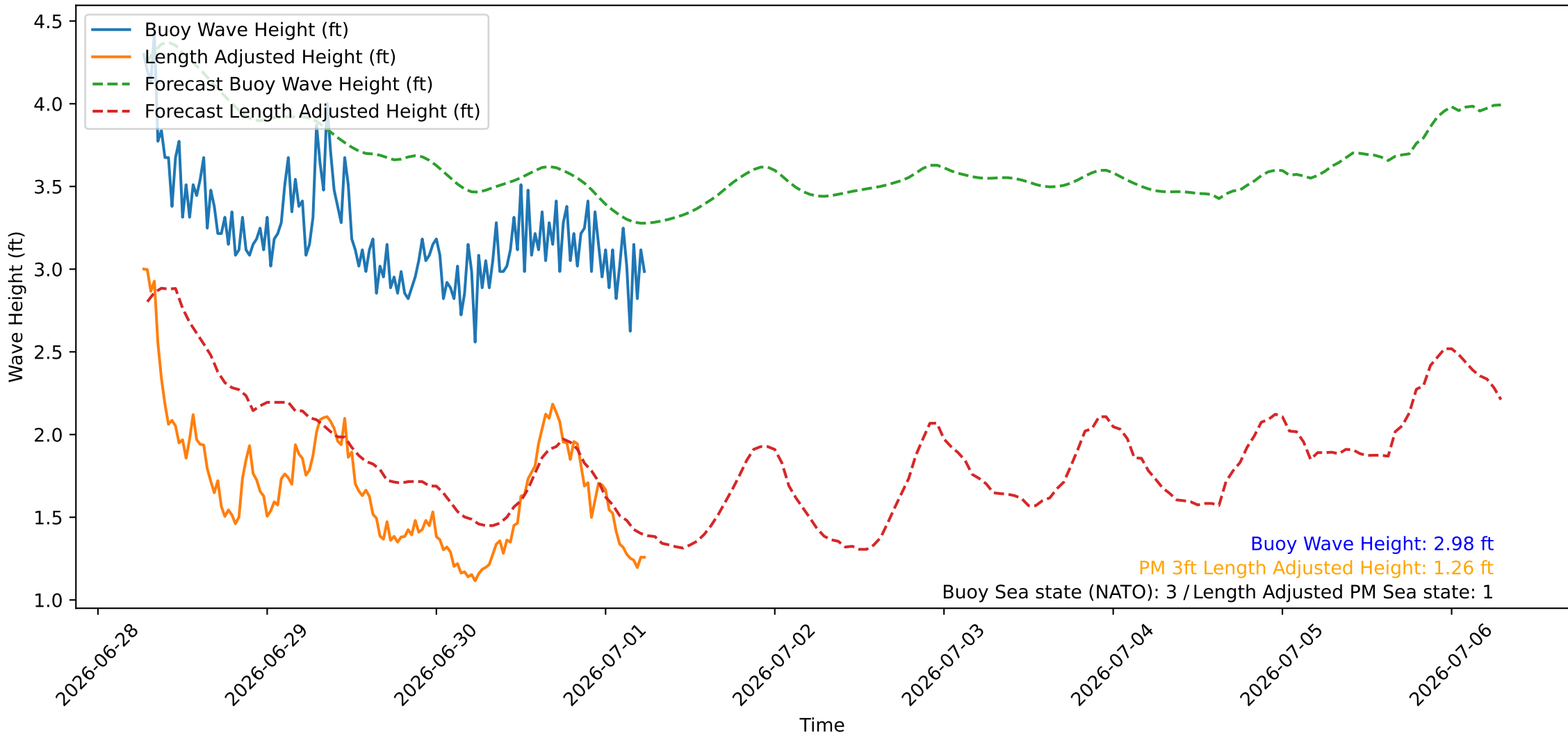
Wave Heights over Time for Oceanside Harbor at 2026-07-01 06:30:26
