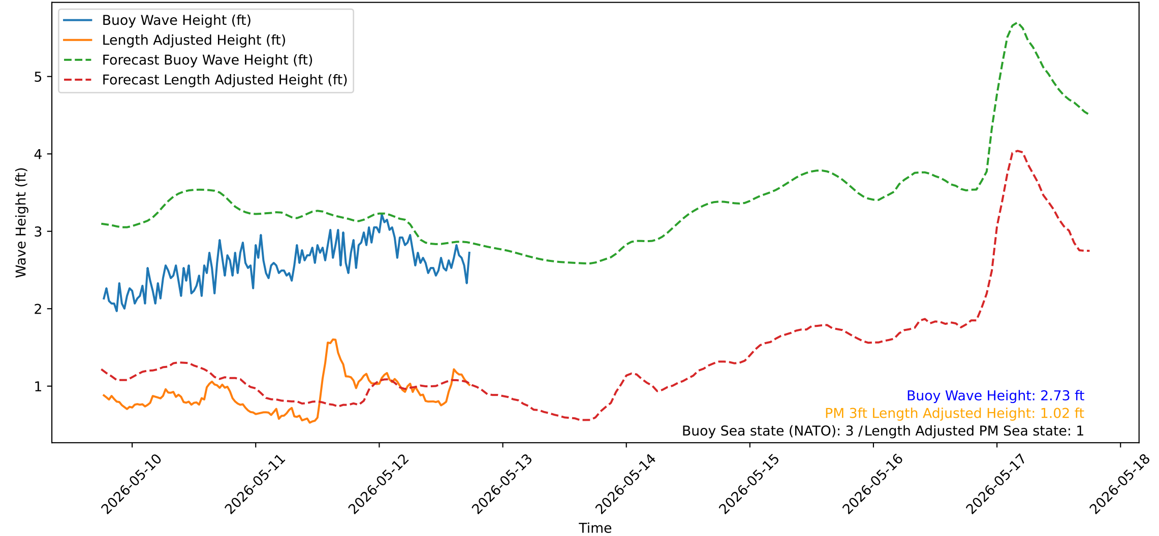
Wave Heights over Time for Red Beach at 2026-05-12 18:10:51
