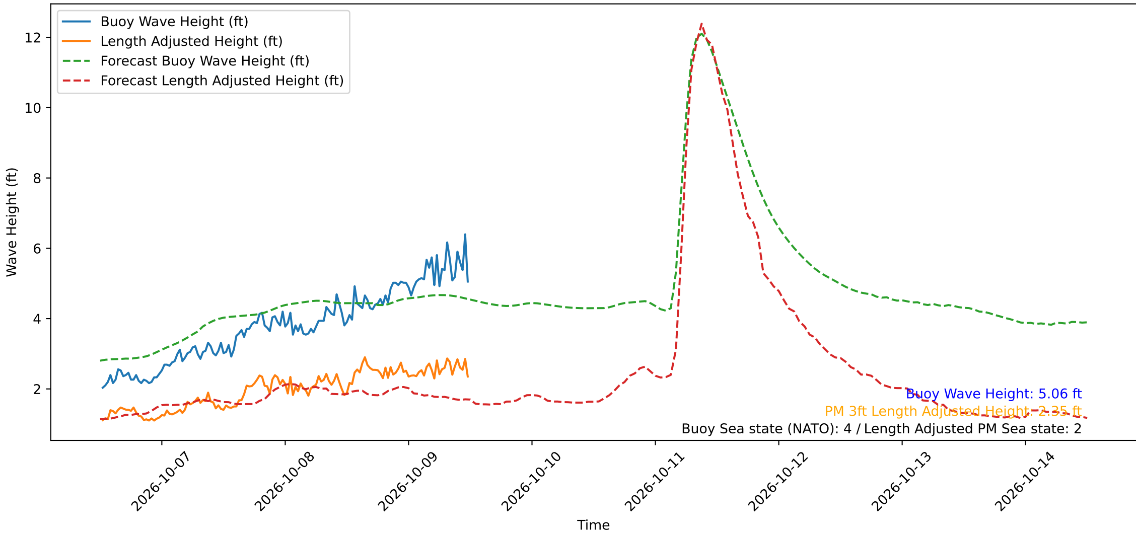
Wave Heights over Time for Oceanside Harbor at 2026-10-09 12:20:29
