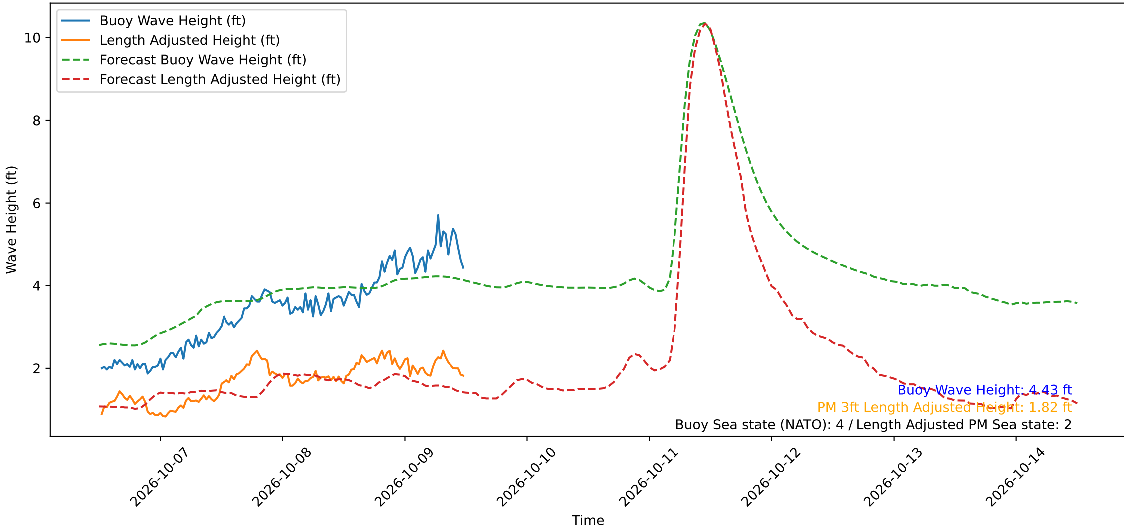
Wave Heights over Time for Red Beach at 2026-10-09 12:20:49
