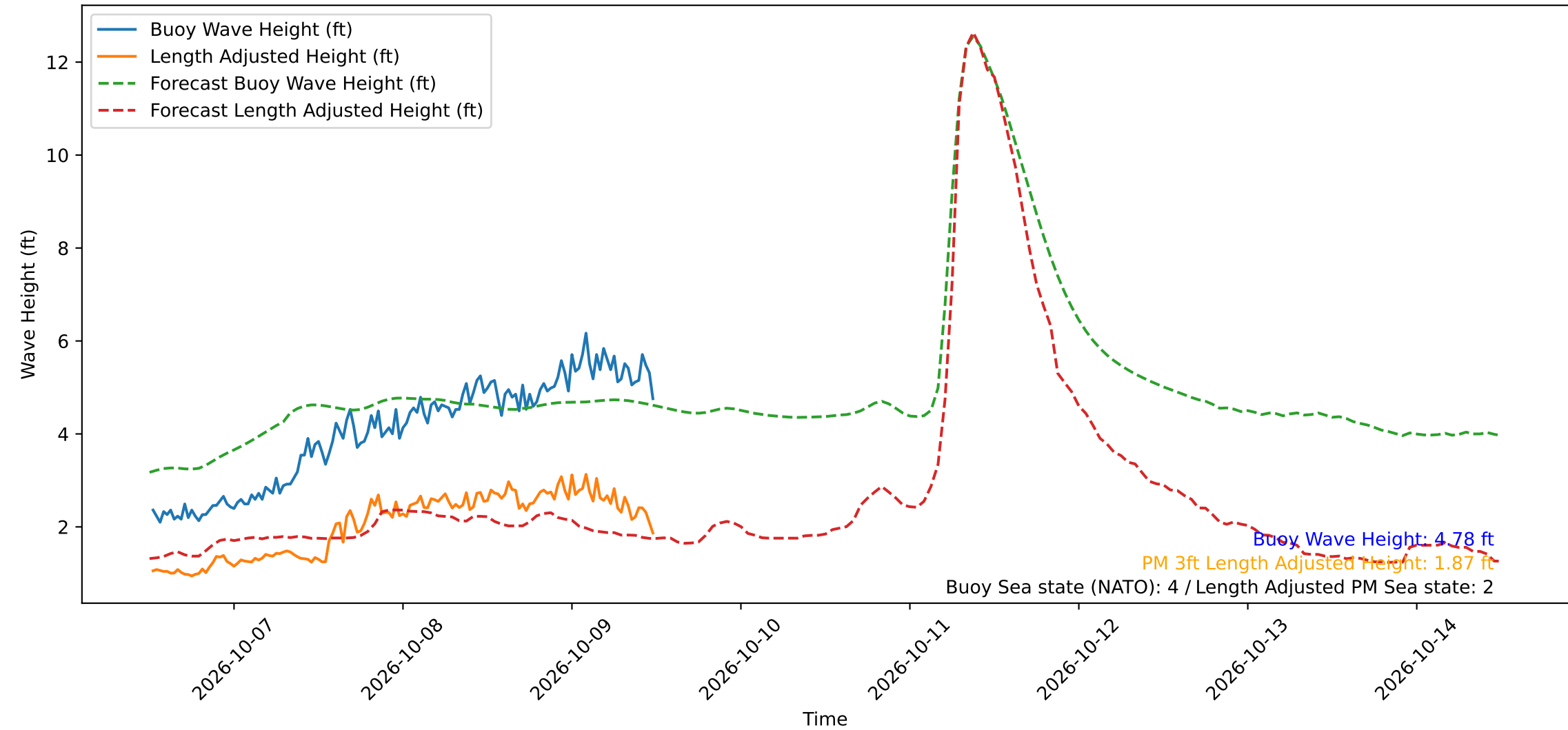
Wave Heights over Time for Green Beach at 2026-10-09 12:21:14
