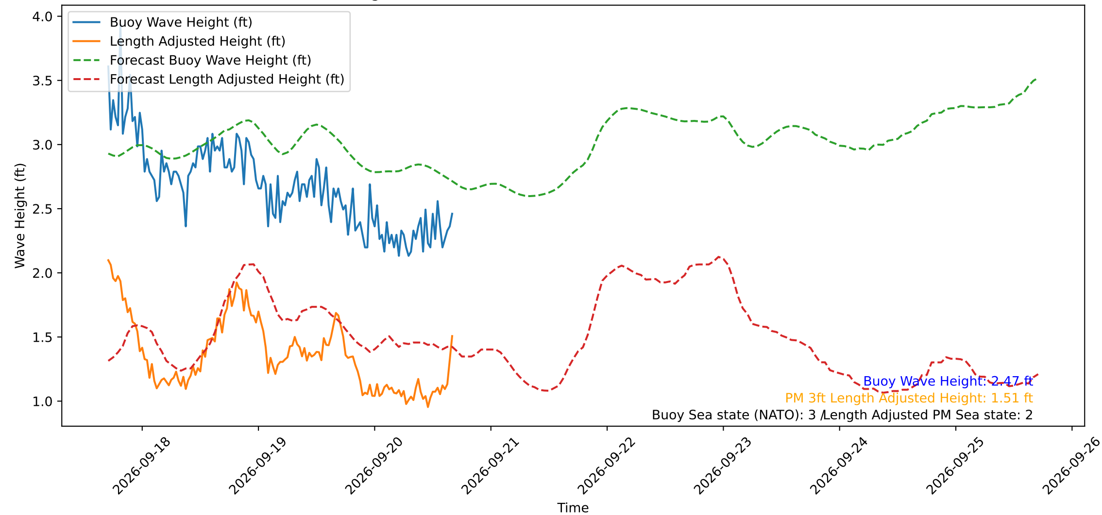
Wave Heights over Time for Oceanside Harbor at 2026-09-20 16:50:30
