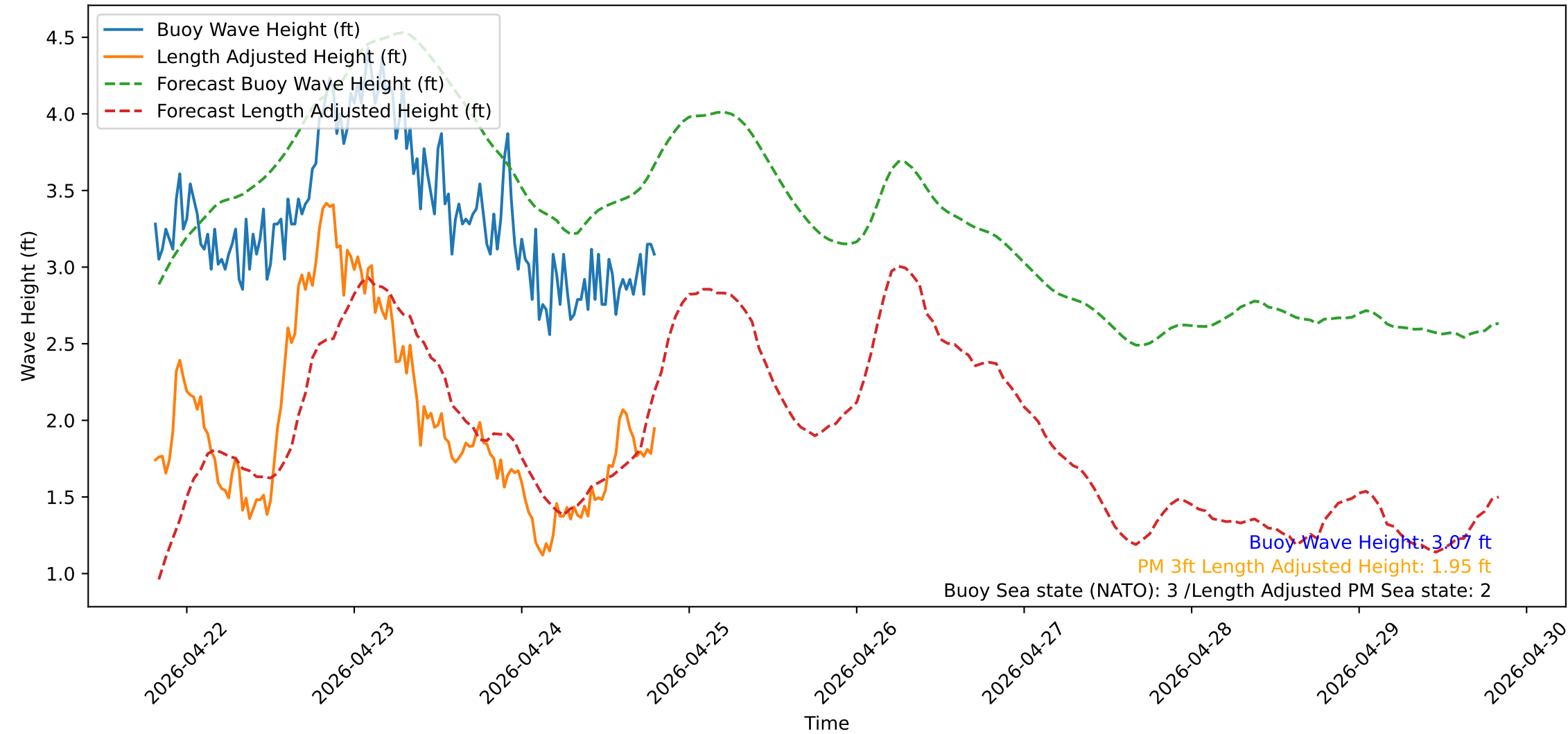
Wave Heights over Time for Oceanside Harbor at 2026-04-24 19:30:31
