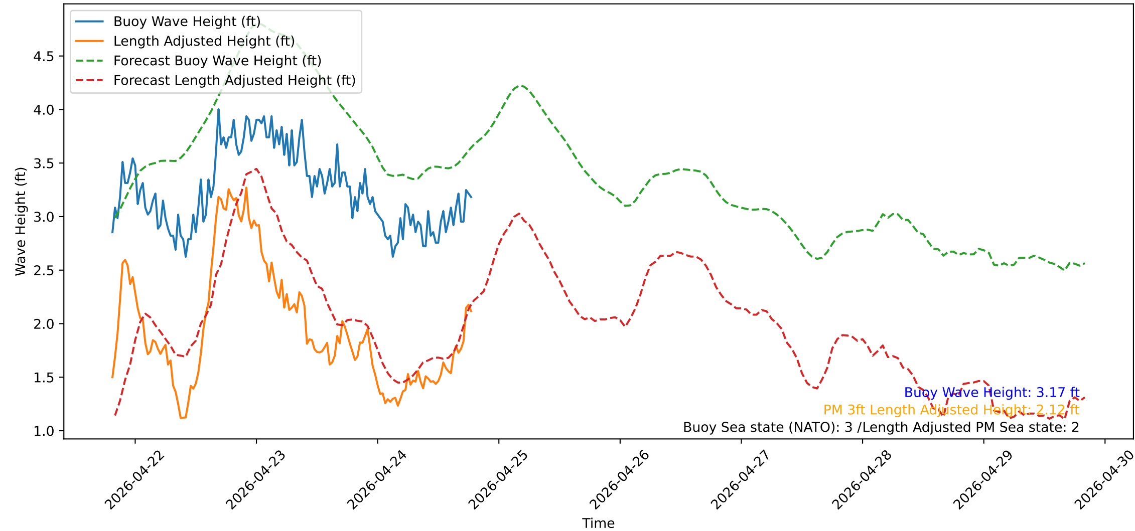
Wave Heights over Time for Green Beach at 2026-04-24 19:31:12
