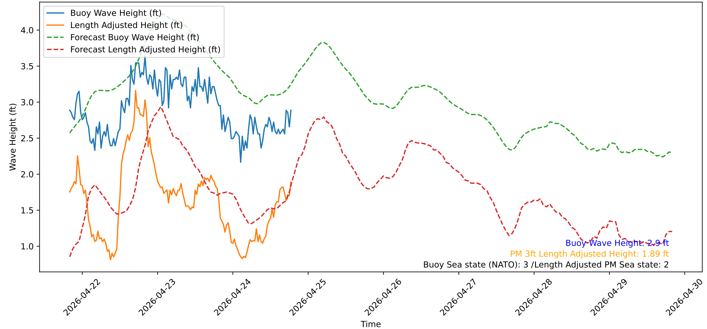
Wave Heights over Time for Red Beach at 2026-04-24 19:30:50
