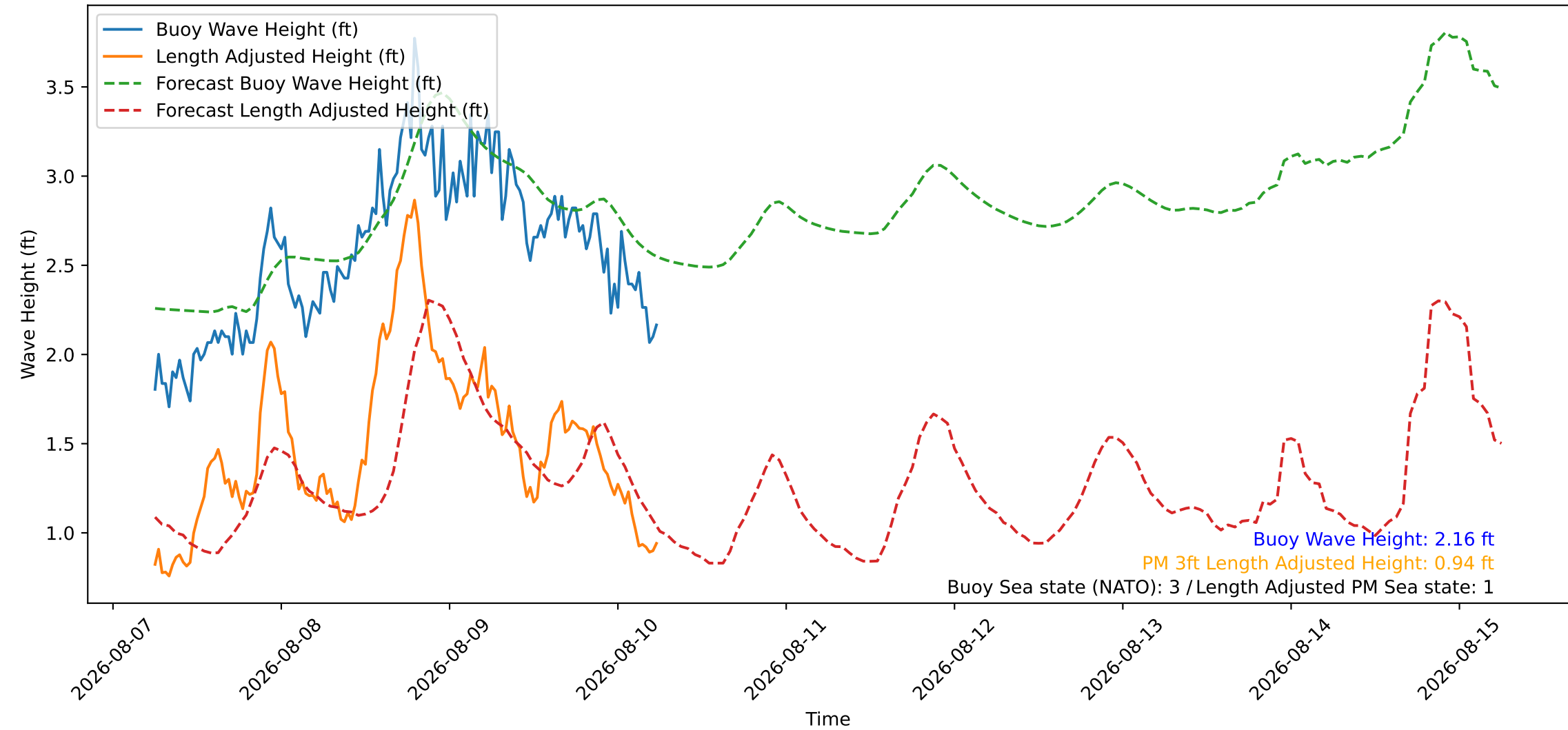
Wave Heights over Time for Green Beach at 2026-08-10 06:11:09
