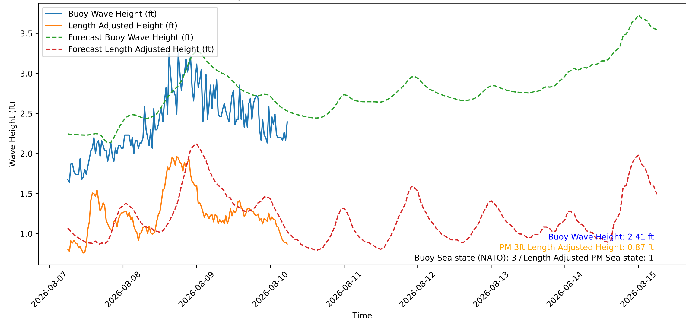
Wave Heights over Time for Oceanside Harbor at 2026-08-10 06:10:27
