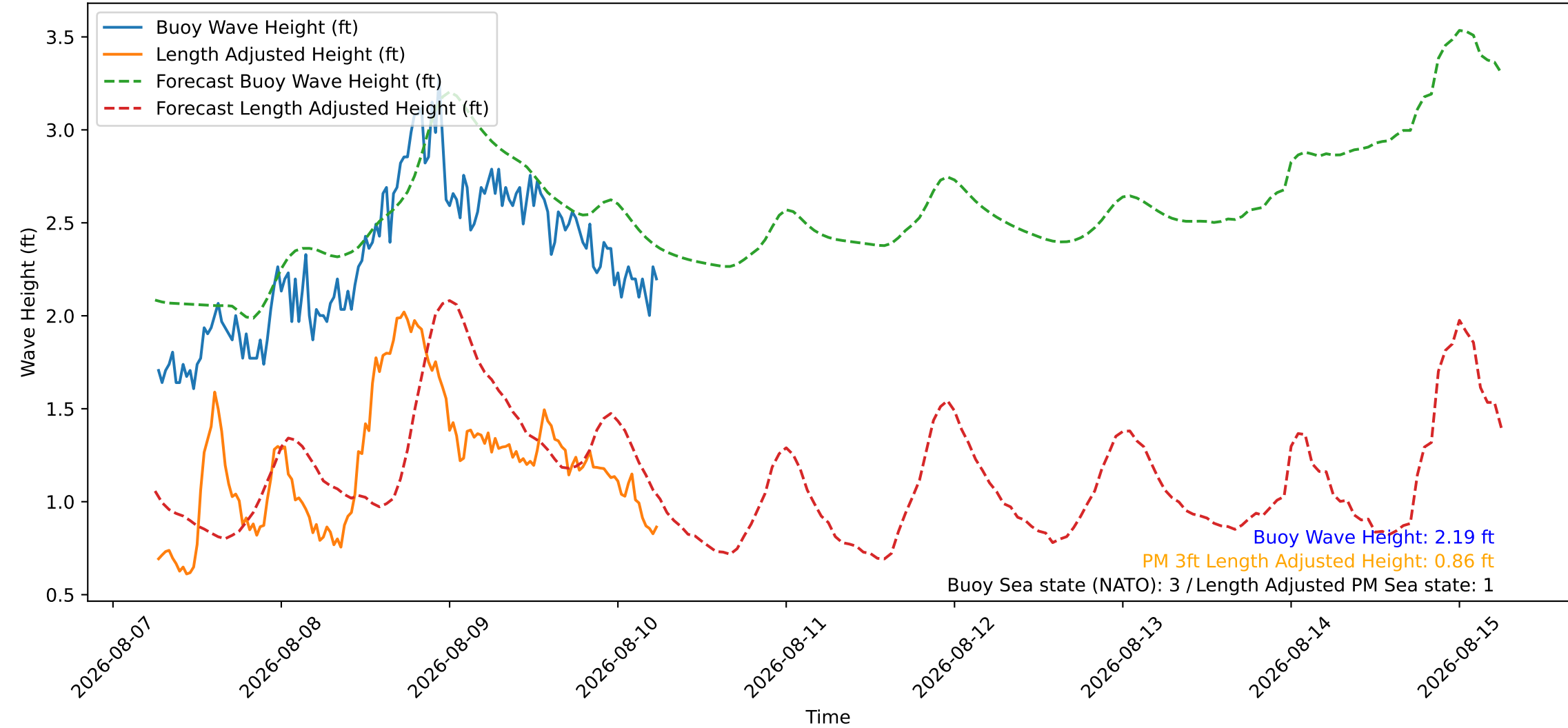
Wave Heights over Time for Red Beach at 2026-08-10 06:10:47
