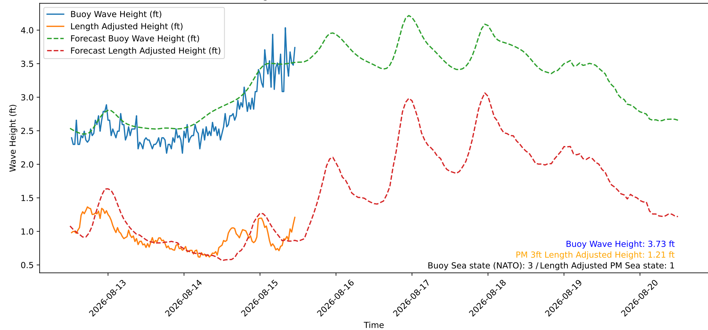
Wave Heights over Time for Red Beach at 2026-08-15 12:00:48
