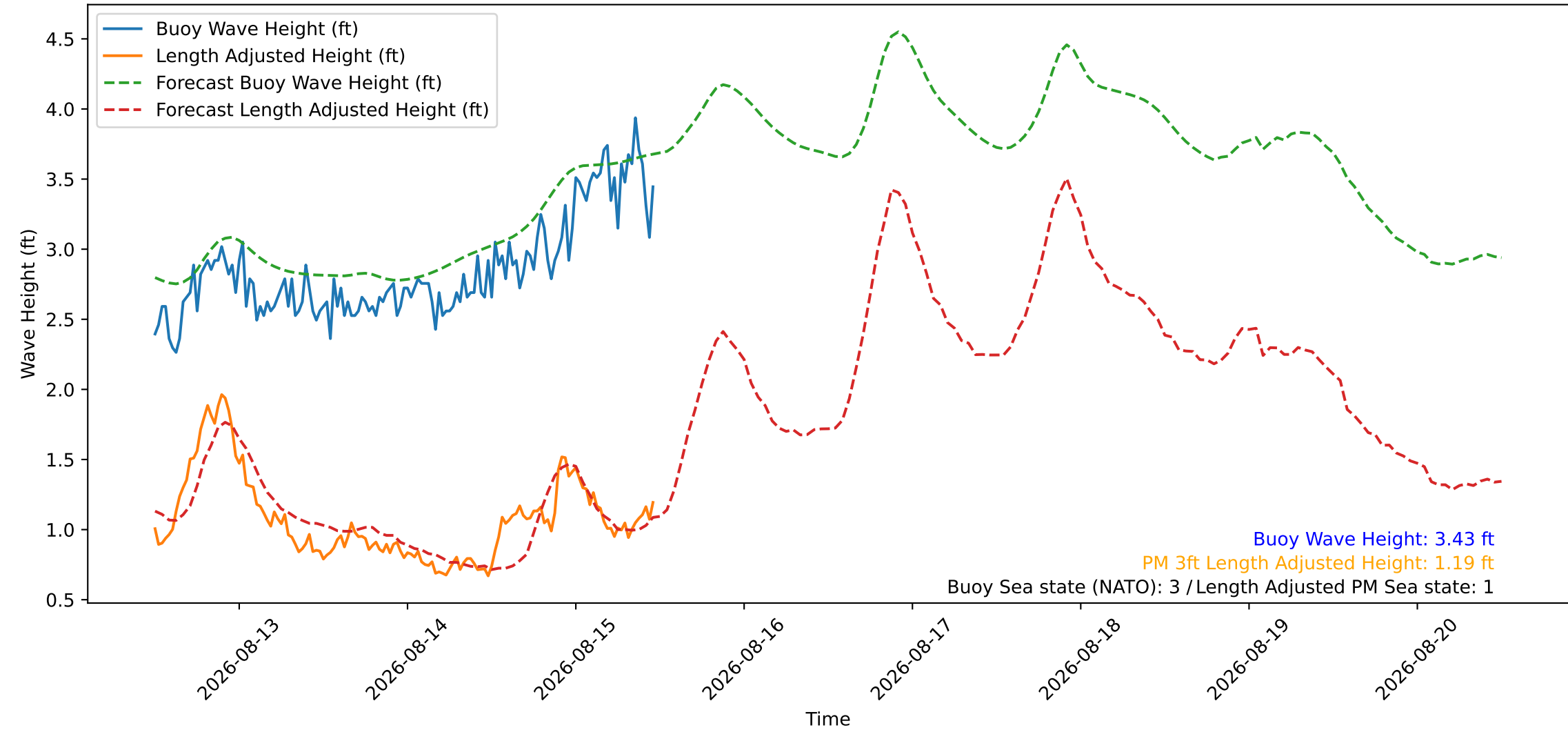
Wave Heights over Time for Green Beach at 2026-08-15 12:01:11
