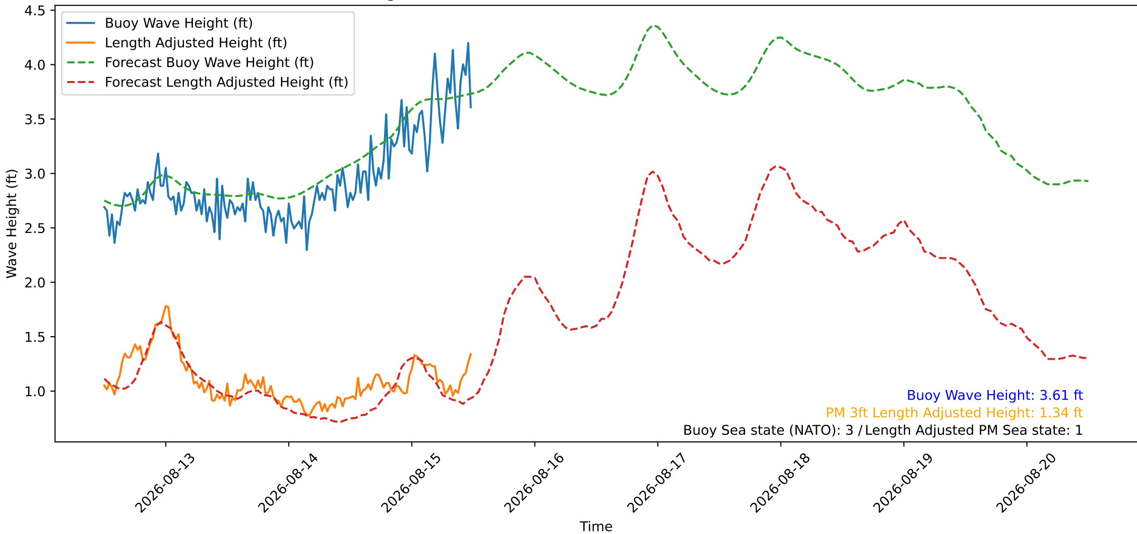
Wave Heights over Time for Oceanside Harbor at 2026-08-15 12:00:27
