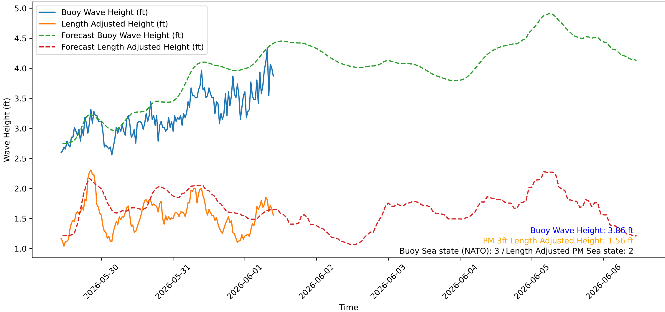
Wave Heights over Time for Green Beach at 2026-06-01 10:31:07
