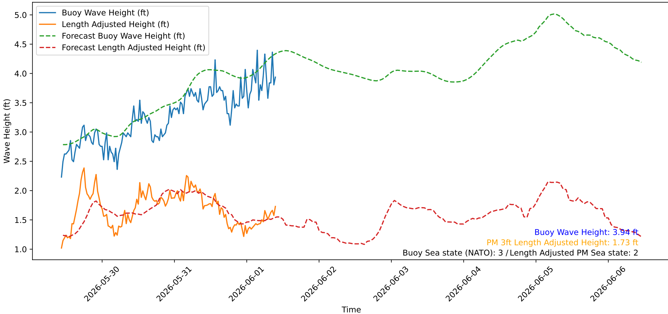
Wave Heights over Time for Oceanside Harbor at 2026-06-01 10:30:25
