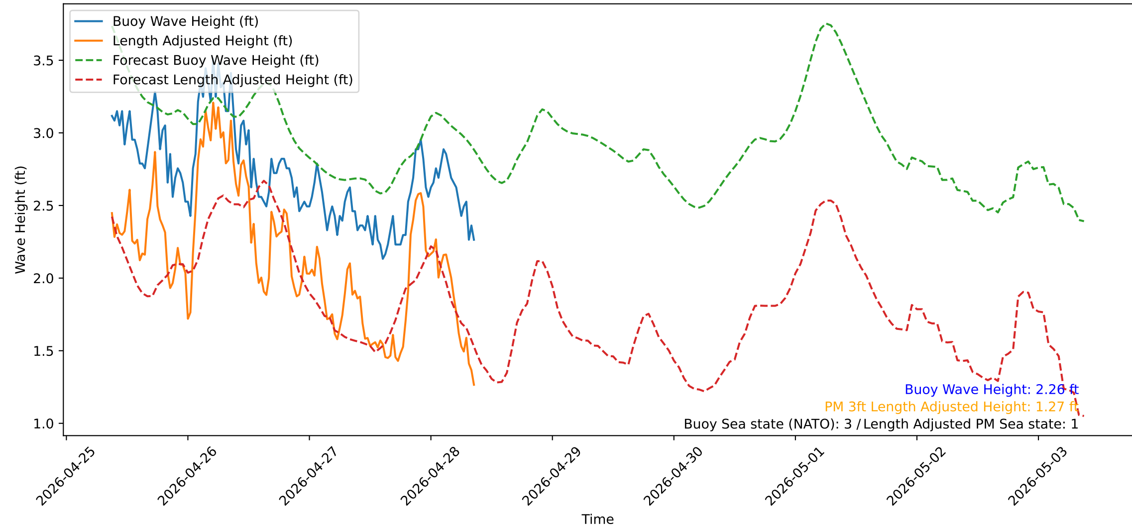
Wave Heights over Time for Green Beach at 2026-04-28 09:11:12
