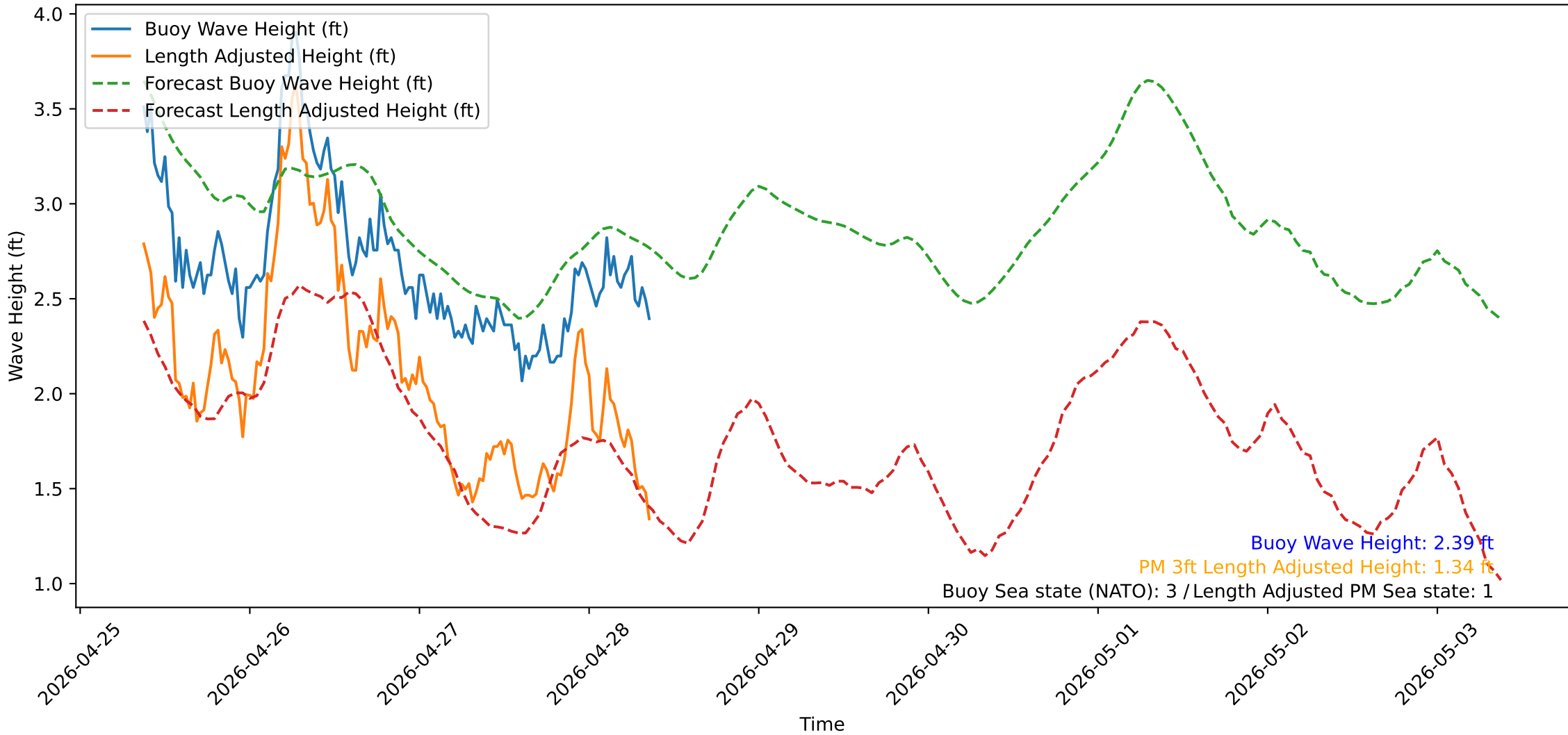
Wave Heights over Time for Oceanside Harbor at 2026-04-28 09:10:31
