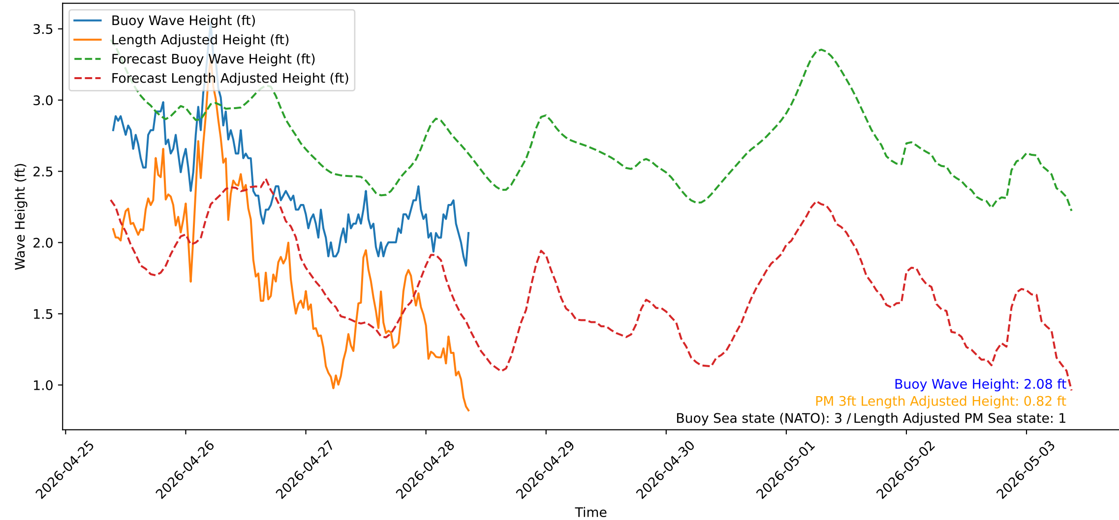
Wave Heights over Time for Red Beach at 2026-04-28 09:10:50
