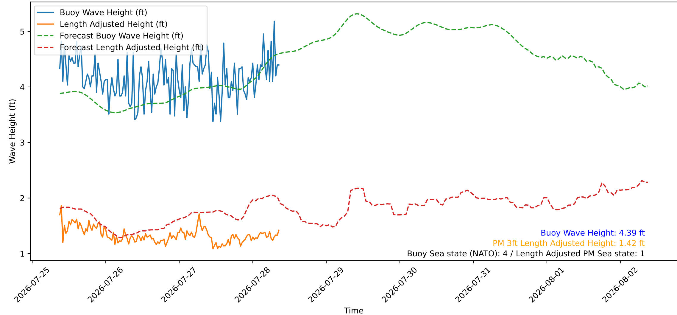
Wave Heights over Time for Green Beach at 2026-07-28 09:11:10
