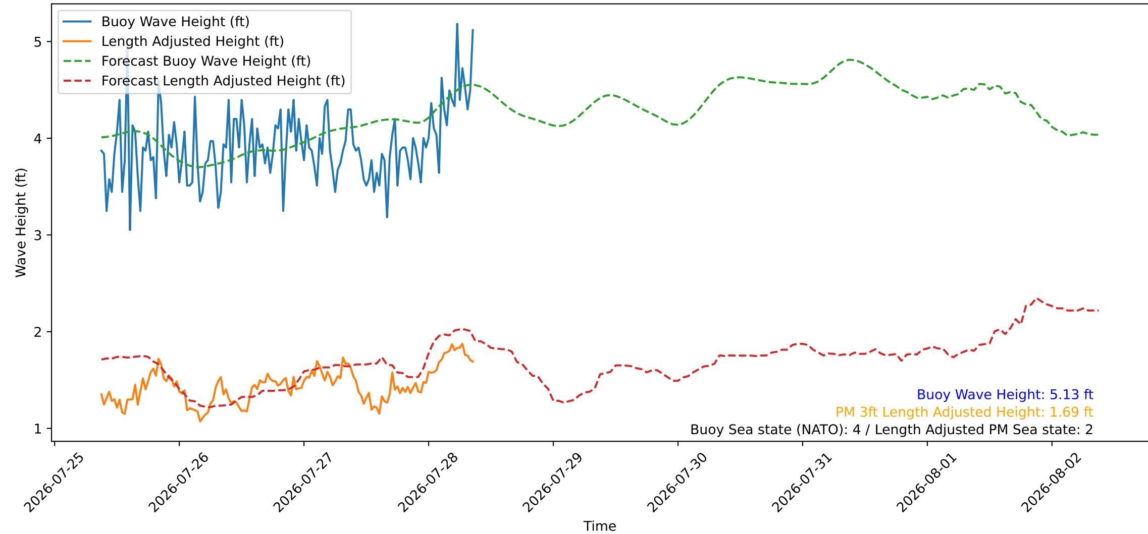
Wave Heights over Time for Oceanside Harbor at 2026-07-28 09:10:27
