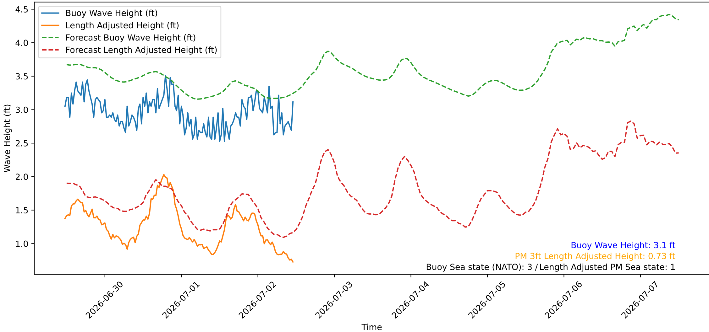
Wave Heights over Time for Green Beach at 2026-07-02 11:41:08
