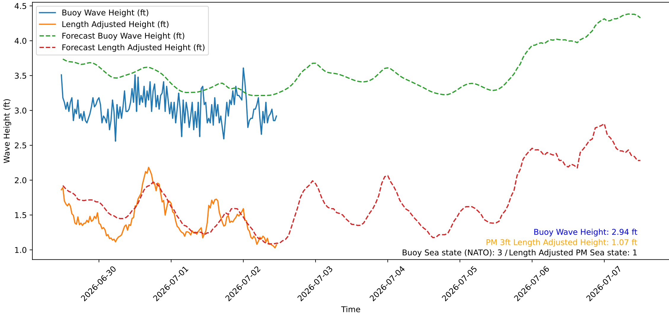
Wave Heights over Time for Oceanside Harbor at 2026-07-02 11:40:26
