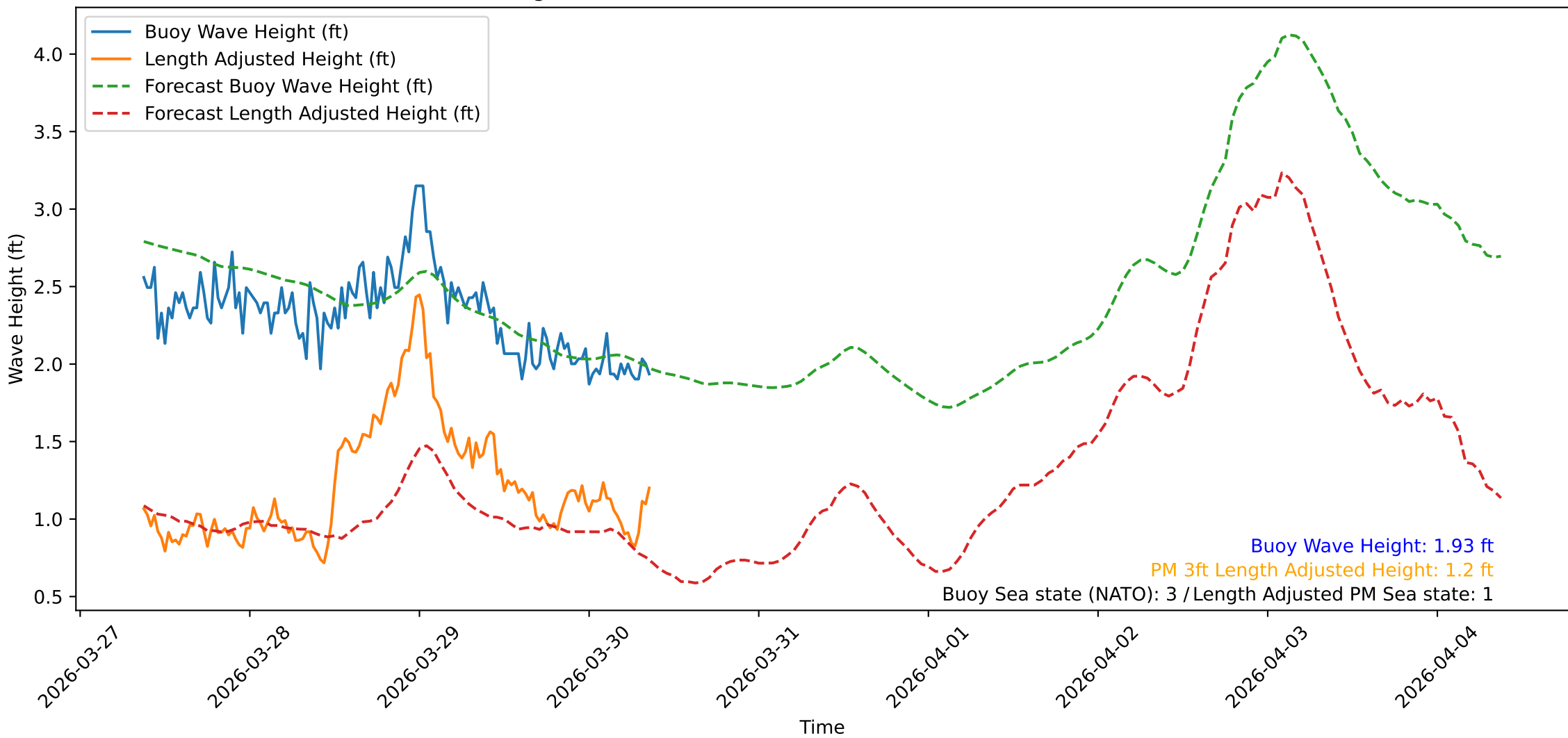
Wave Heights over Time for Oceanside Harbor at 2026-03-30 09:10:32
