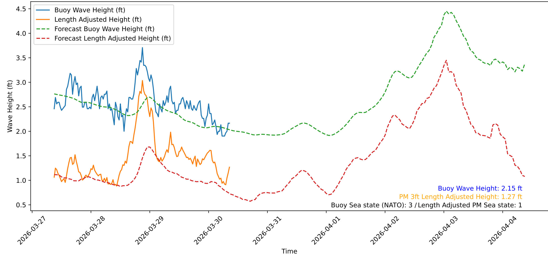
Wave Heights over Time for Green Beach at 2026-03-30 09:11:10
