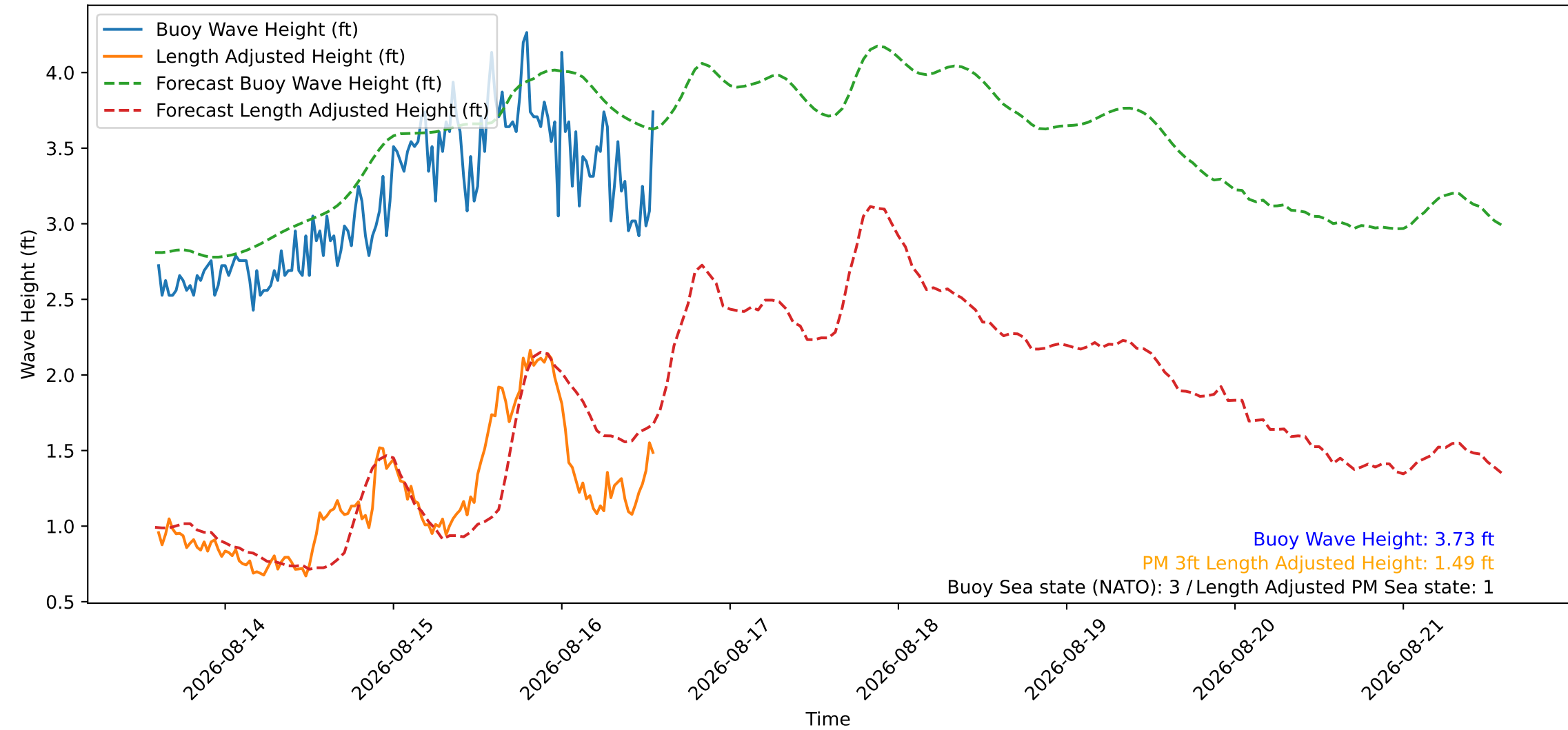
Wave Heights over Time for Green Beach at 2026-08-16 14:01:08
