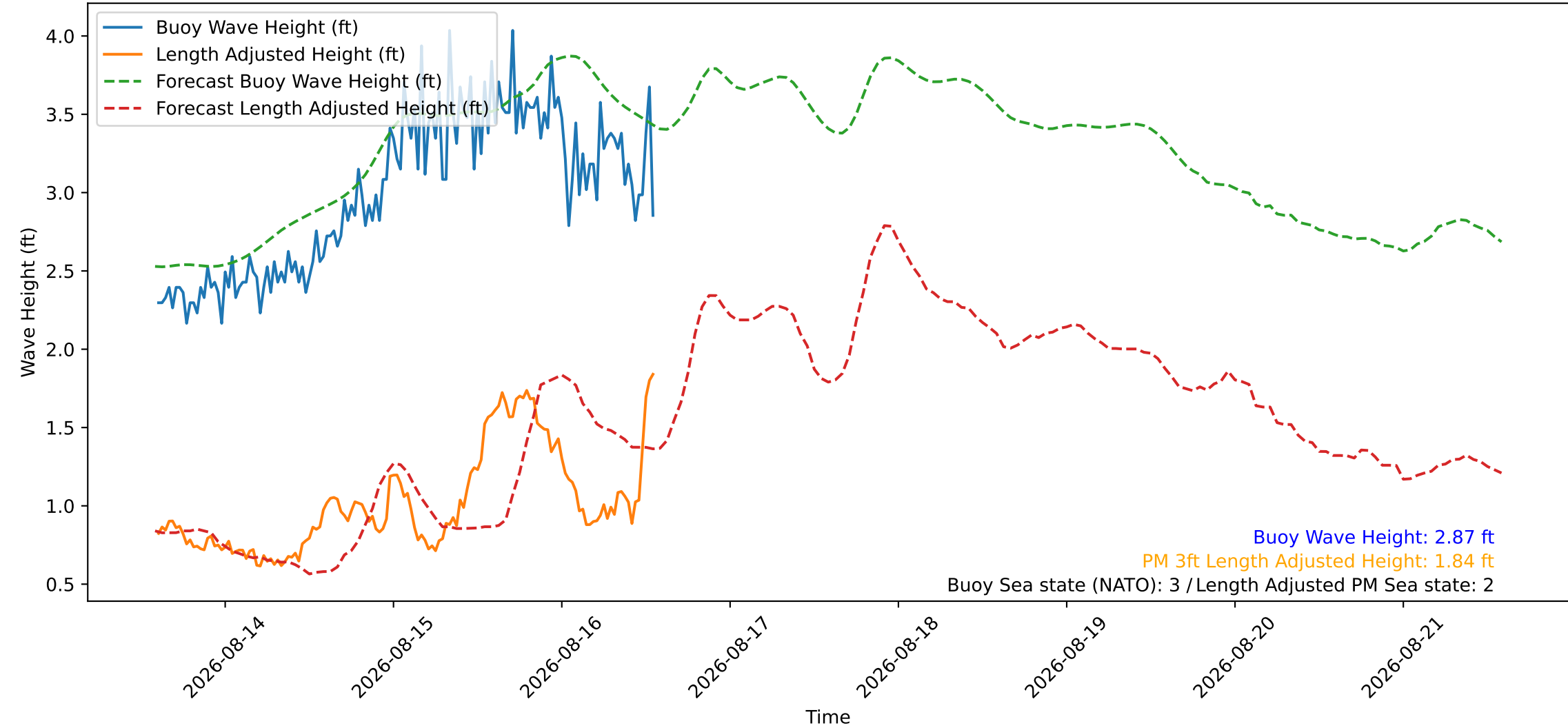
Wave Heights over Time for Red Beach at 2026-08-16 14:00:46
