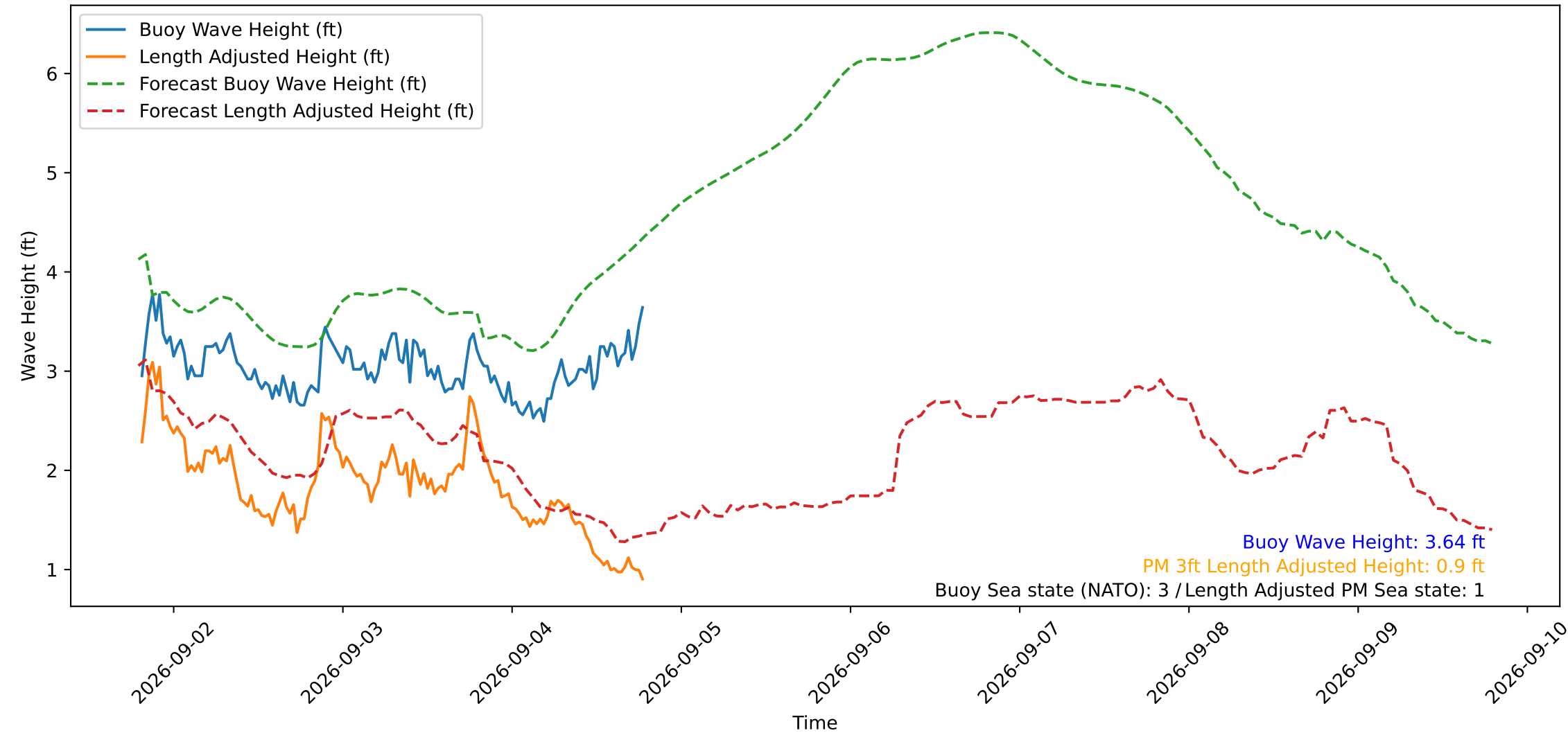
Wave Heights over Time for Green Beach at 2026-09-04 19:11:13
