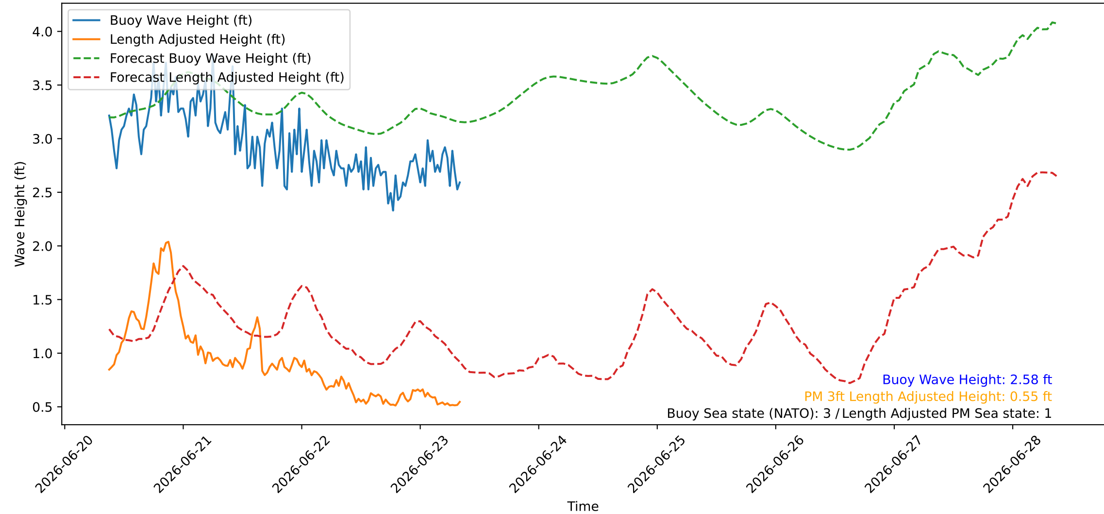
Wave Heights over Time for Red Beach at 2026-06-23 08:50:48
