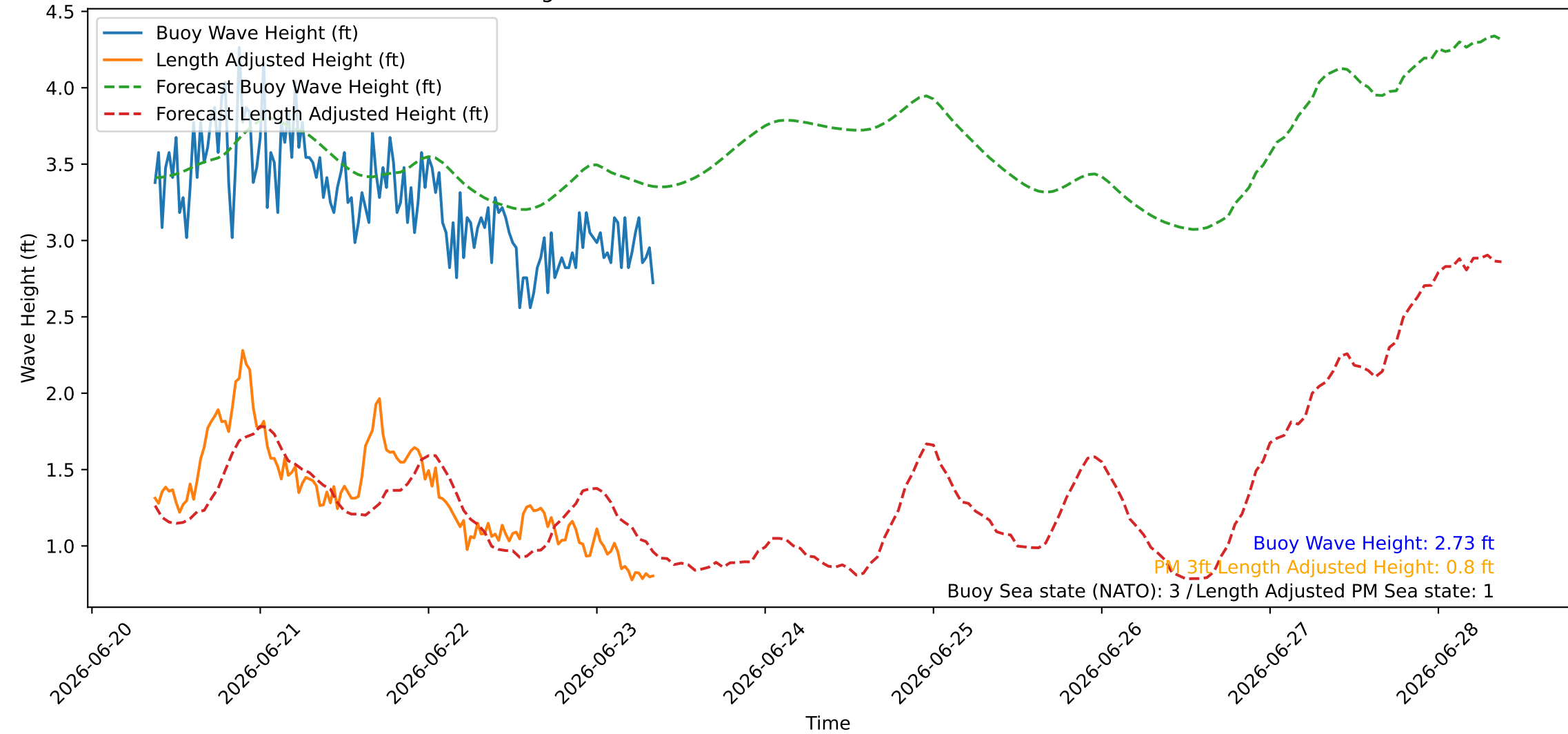
Wave Heights over Time for Oceanside Harbor at 2026-06-23 08:50:27
