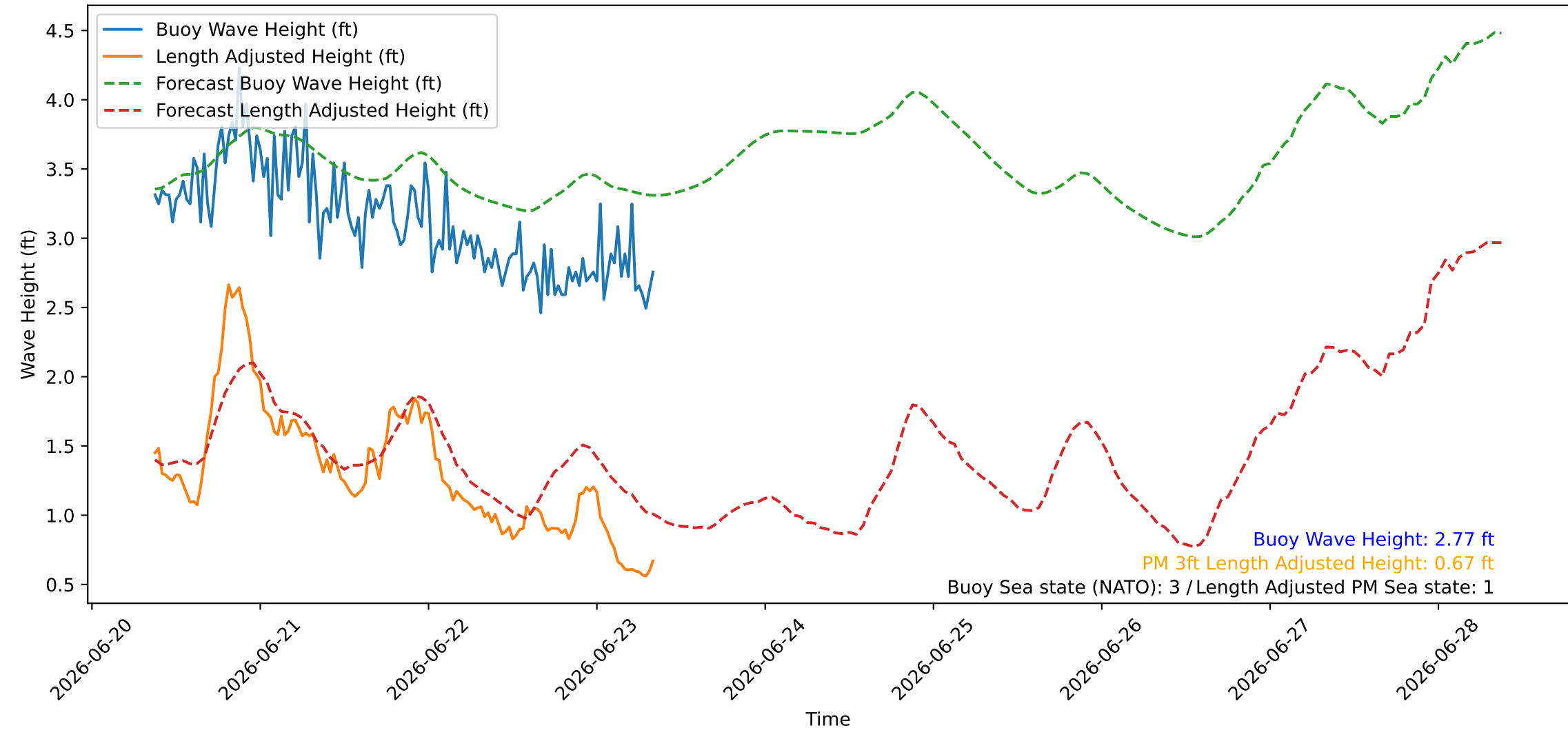
Wave Heights over Time for Green Beach at 2026-06-23 08:51:10
