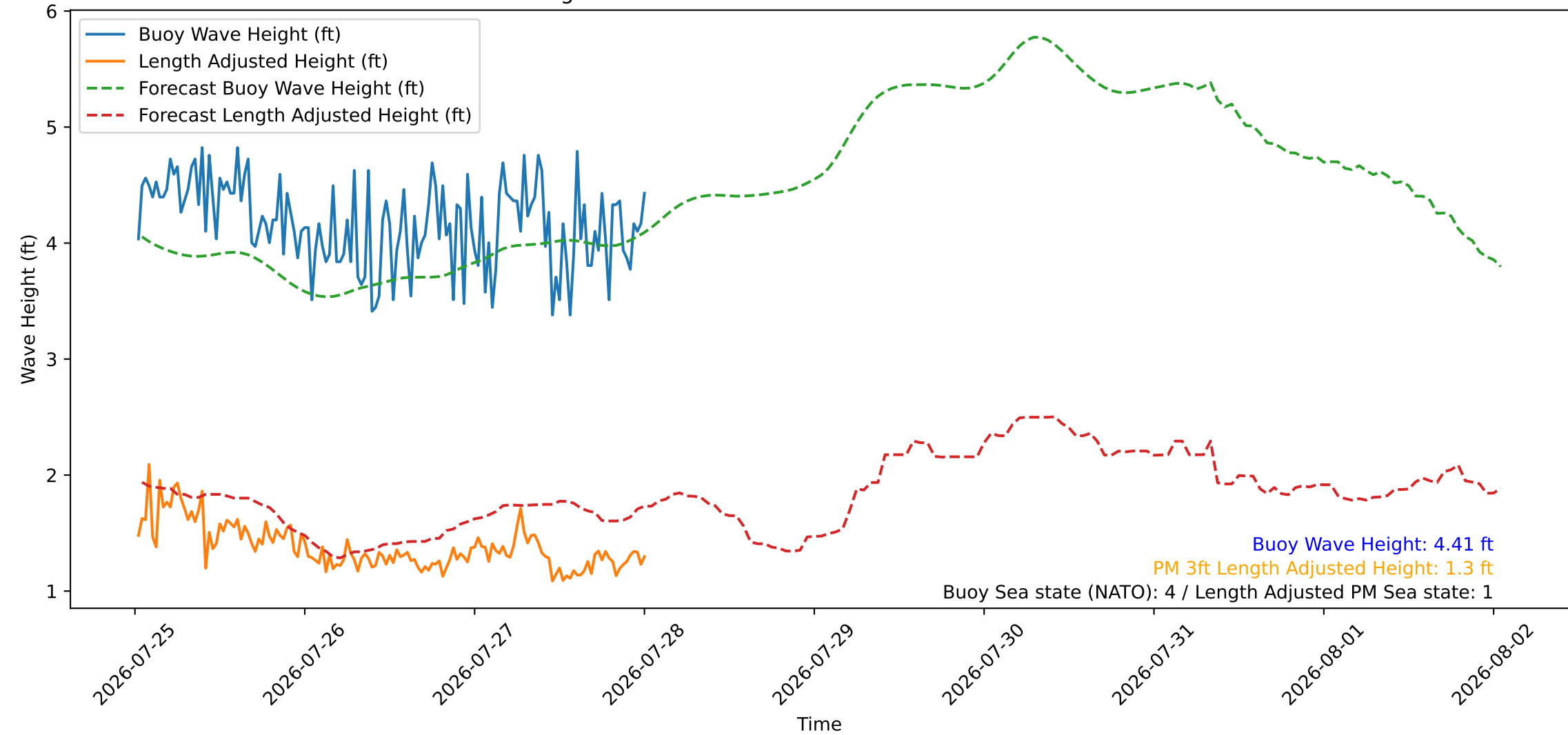
Wave Heights over Time for Green Beach at 2026-07-28 00:41:09
