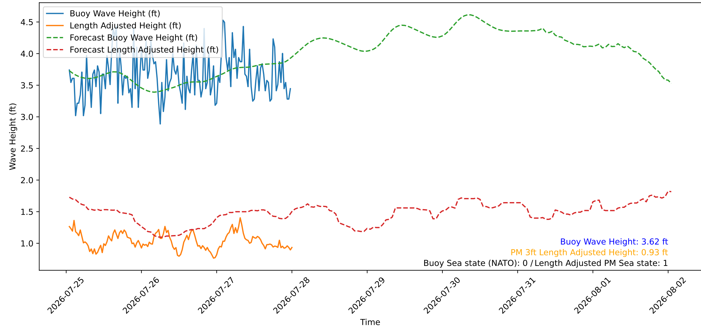
Wave Heights over Time for Red Beach at 2026-07-28 00:40:47
