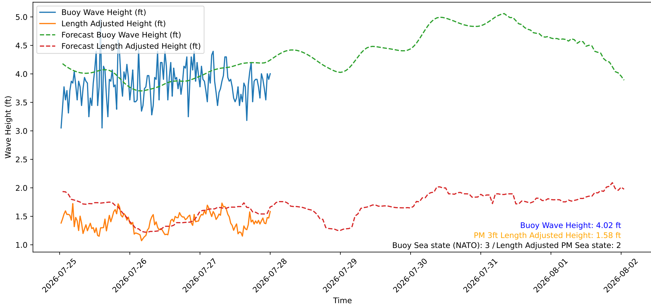
Wave Heights over Time for Oceanside Harbor at 2026-07-28 00:40:26
