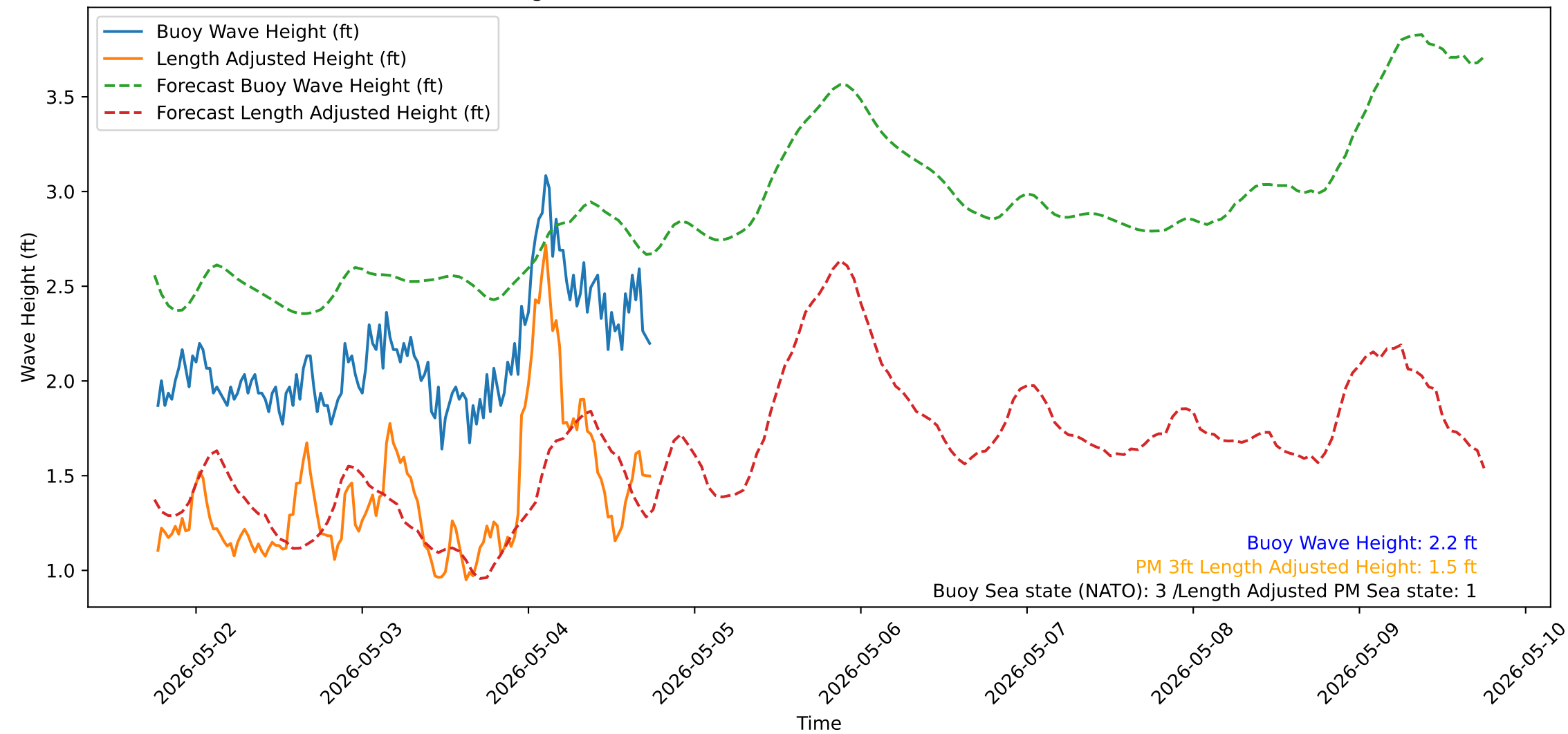
Wave Heights over Time for Oceanside Harbor at 2026-05-04 18:20:31
