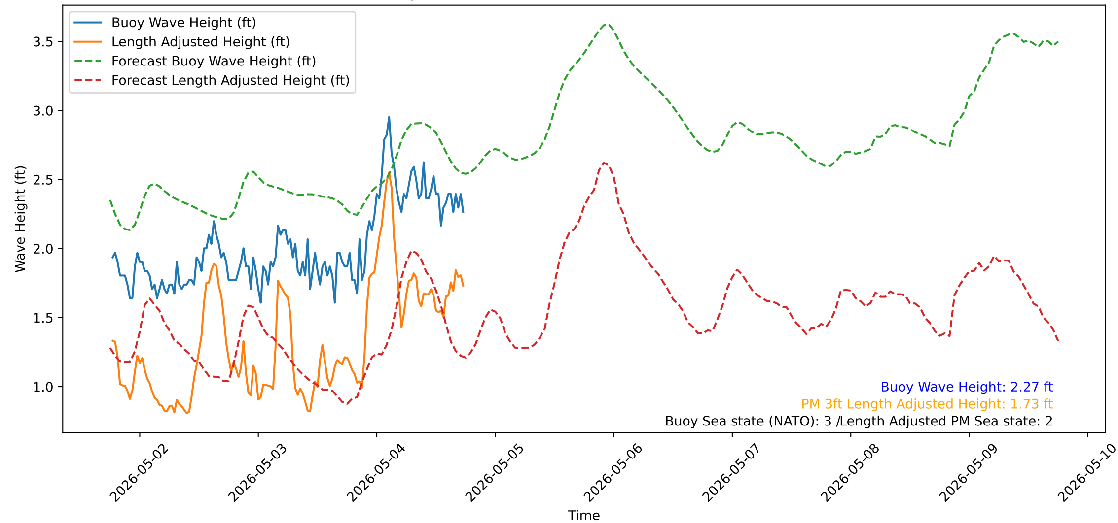
Wave Heights over Time for Red Beach at 2026-05-04 18:20:51
