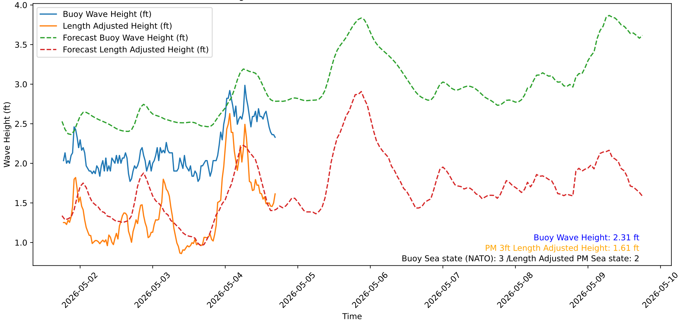
Wave Heights over Time for Green Beach at 2026-05-04 18:21:14
