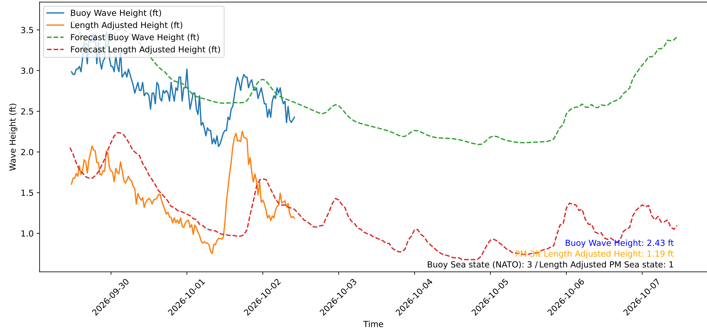
Wave Heights over Time for Red Beach at 2026-10-02 11:00:49
