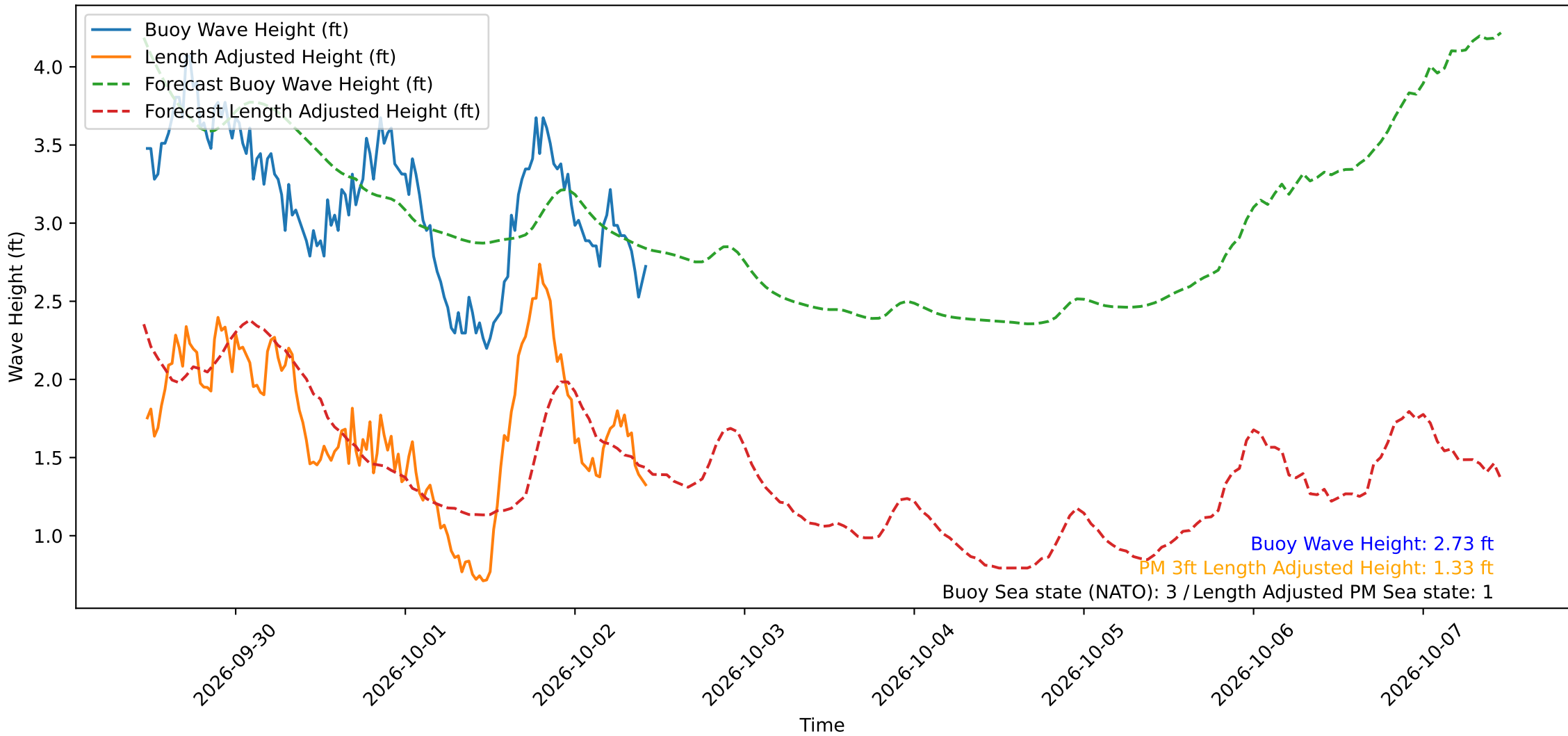
Wave Heights over Time for Green Beach at 2026-10-02 11:01:12
