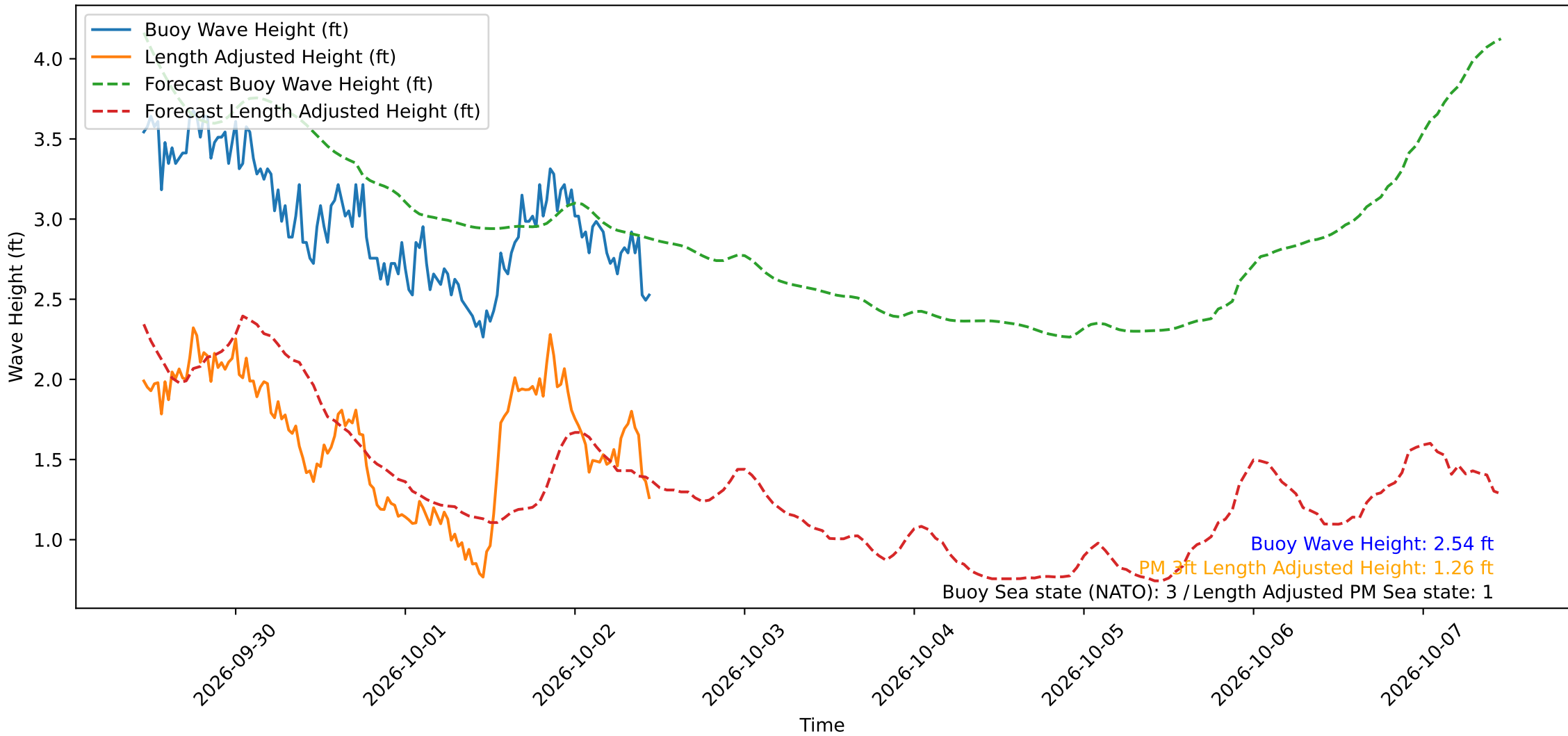
Wave Heights over Time for Oceanside Harbor at 2026-10-02 11:00:30
