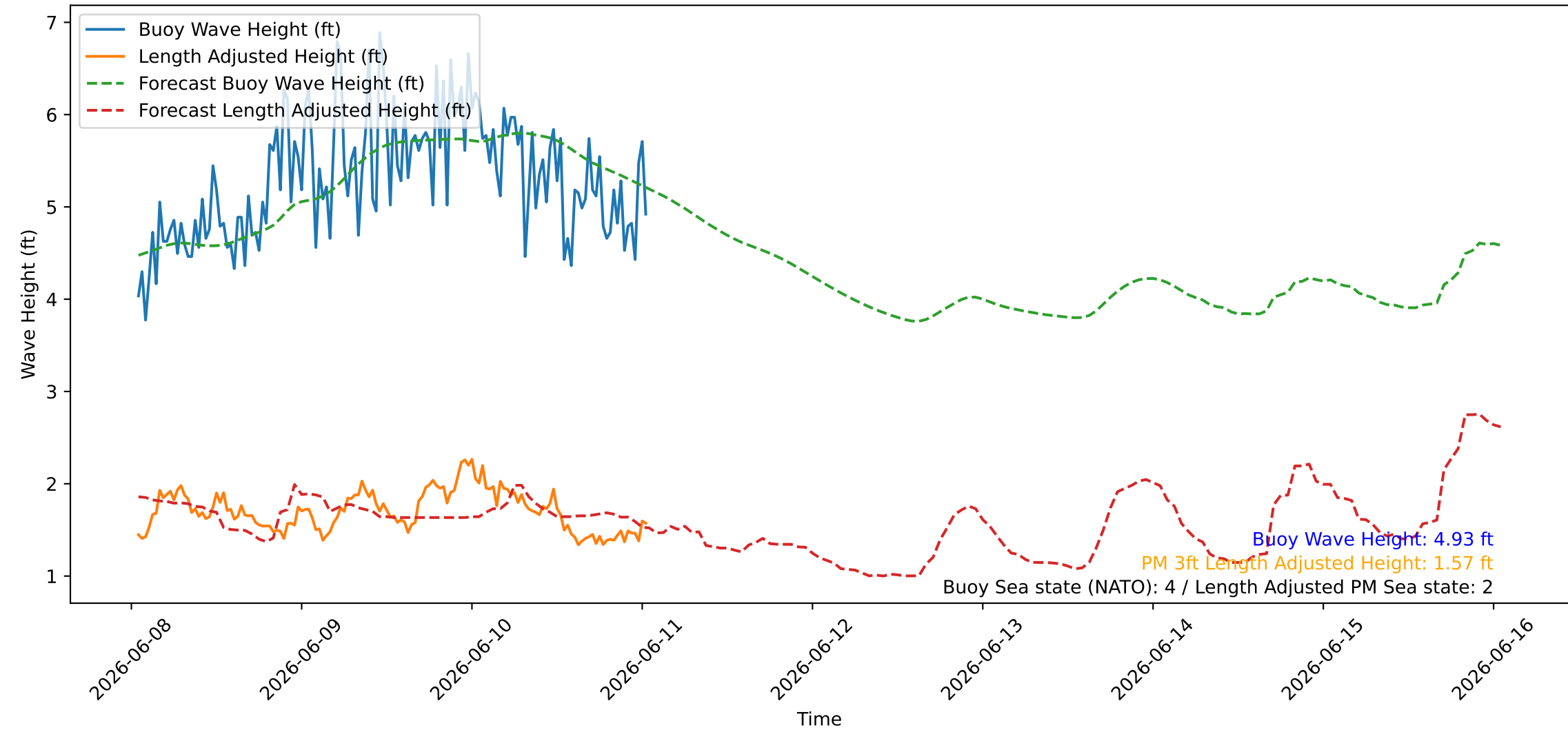
Wave Heights over Time for Green Beach at 2026-06-11 01:11:10
