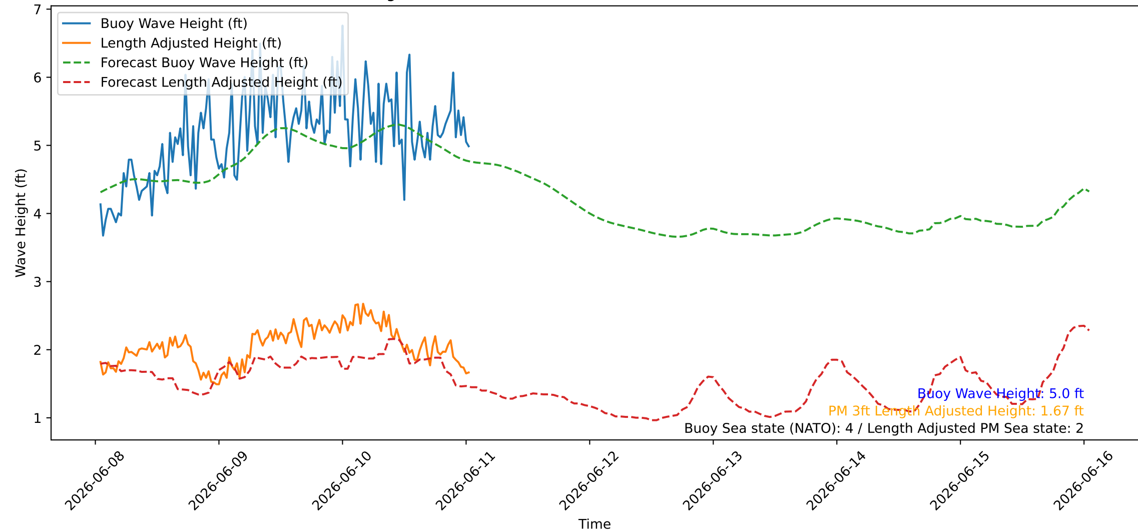
Wave Heights over Time for Oceanside Harbor at 2026-06-11 01:10:26
