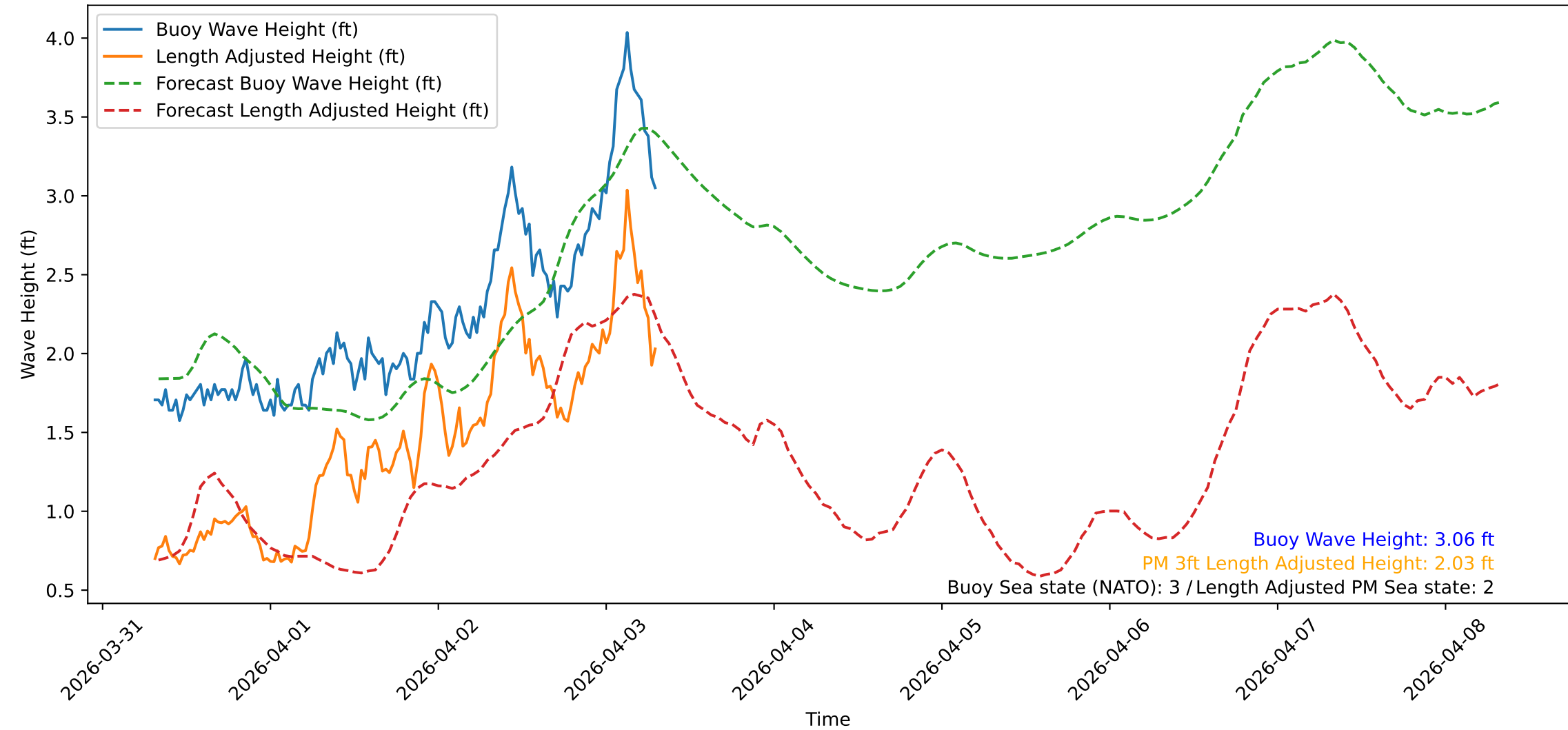
Wave Heights over Time for Oceanside Harbor at 2026-04-03 07:40:31
