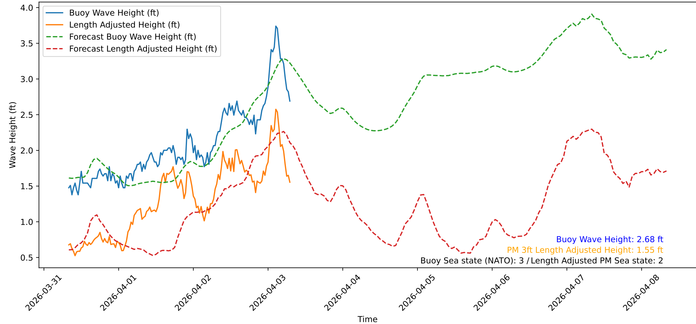
Wave Heights over Time for Red Beach at 2026-04-03 07:40:48
