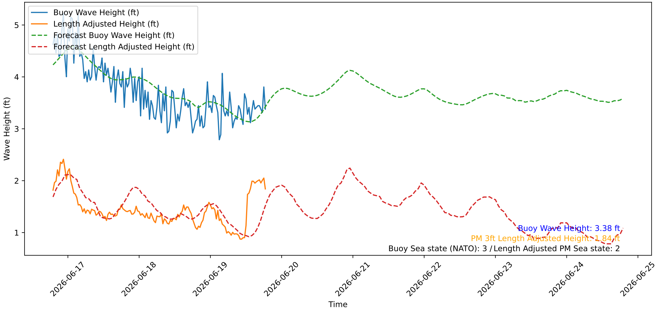
Wave Heights over Time for Oceanside Harbor at 2026-06-19 19:00:26
