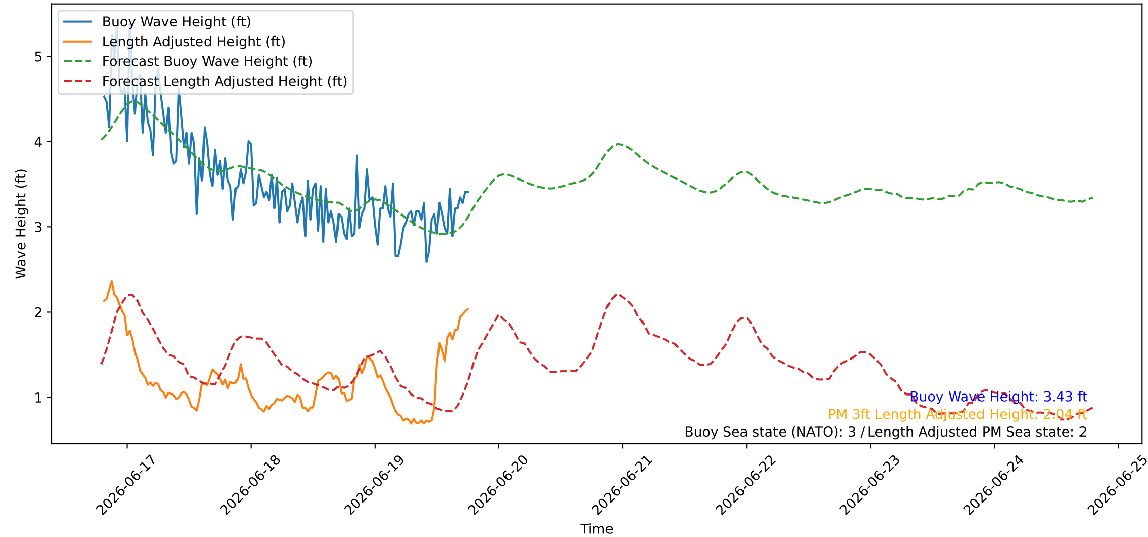
Wave Heights over Time for Red Beach at 2026-06-19 19:00:45
