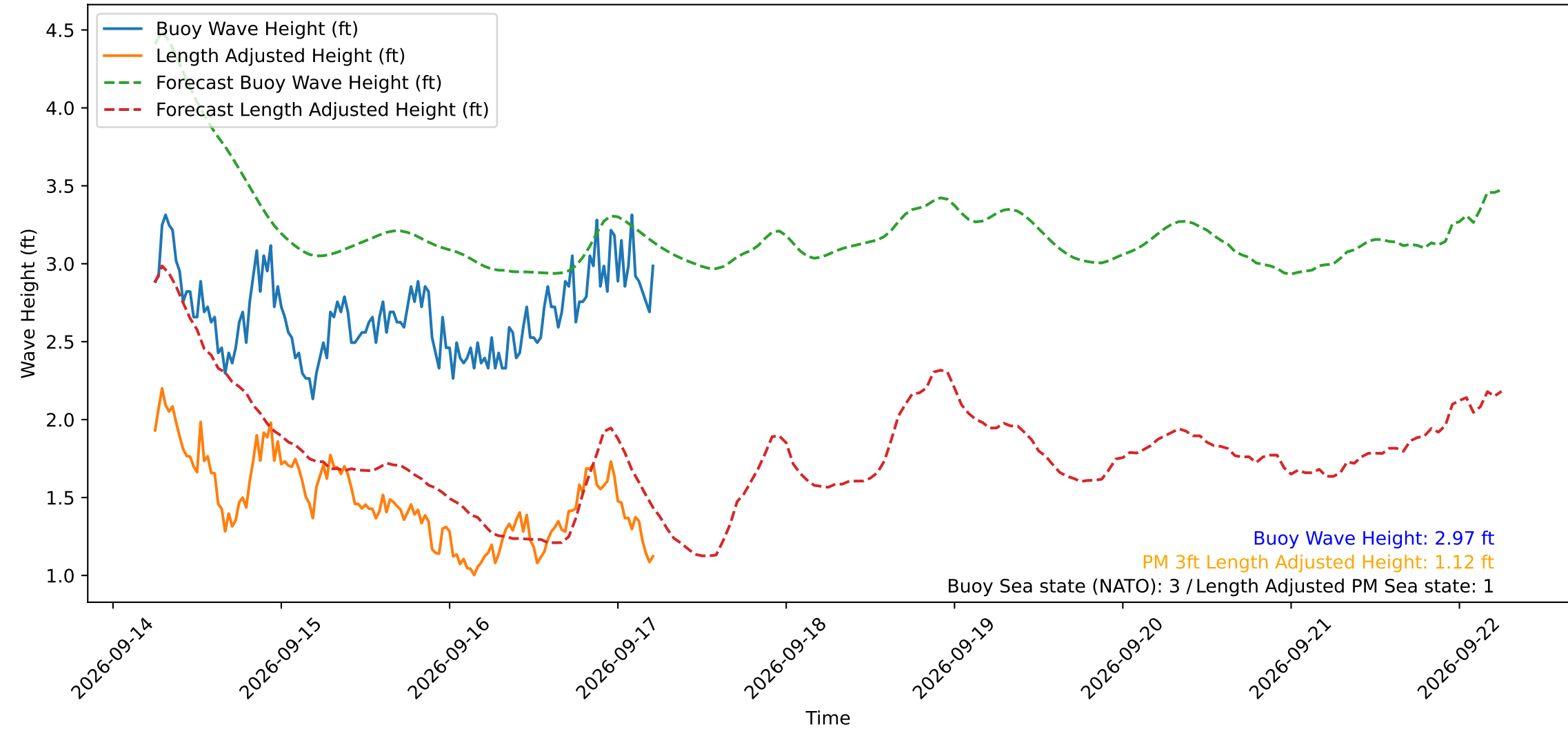
Wave Heights over Time for Green Beach at 2026-09-17 05:51:13
