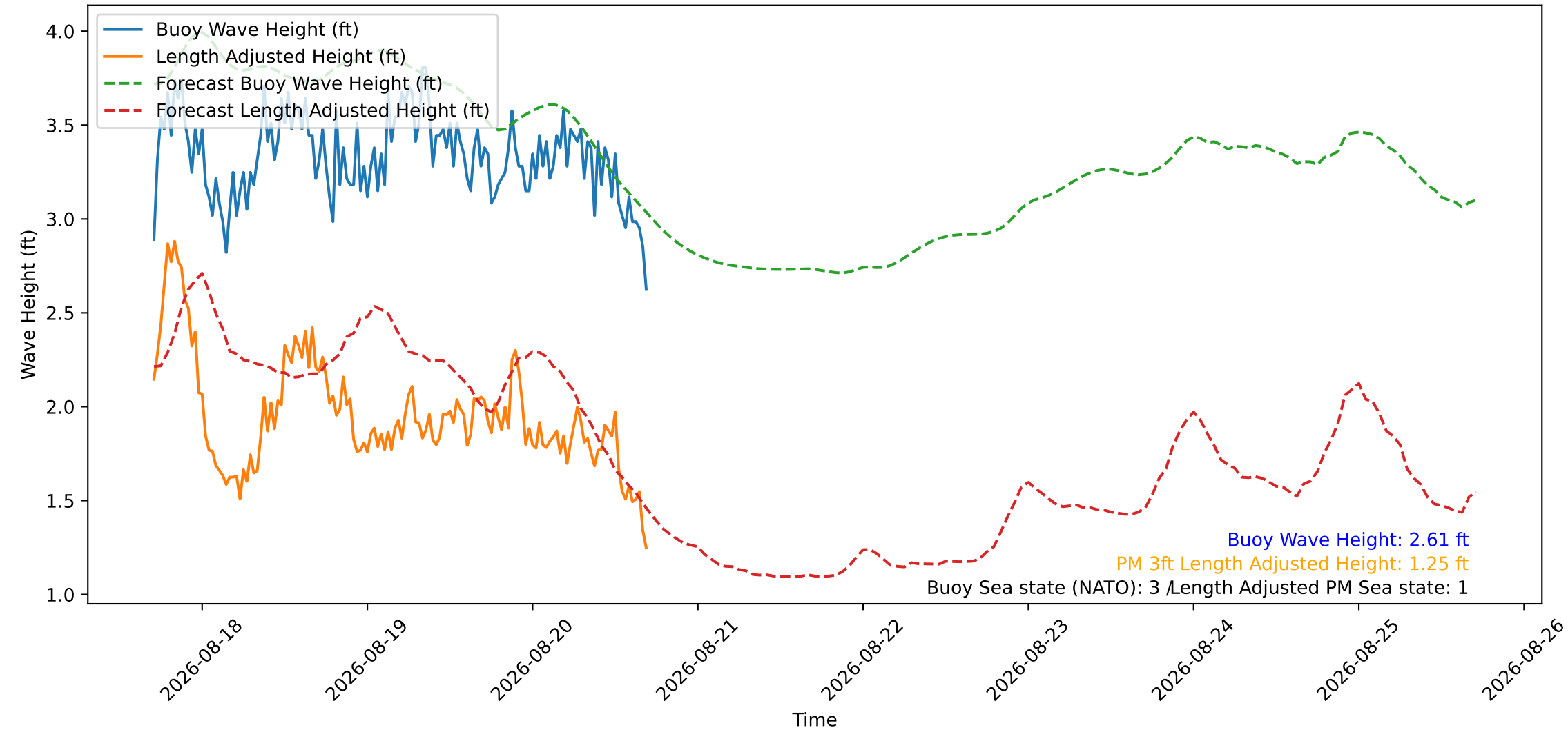
Wave Heights over Time for Oceanside Harbor at 2026-08-20 17:10:26
