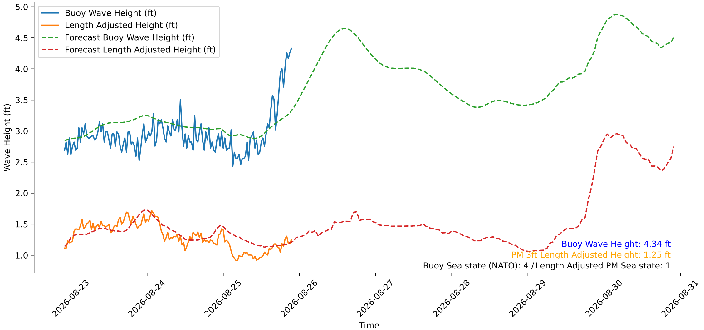
Wave Heights over Time for Oceanside Harbor at 2026-08-25 22:10:29
