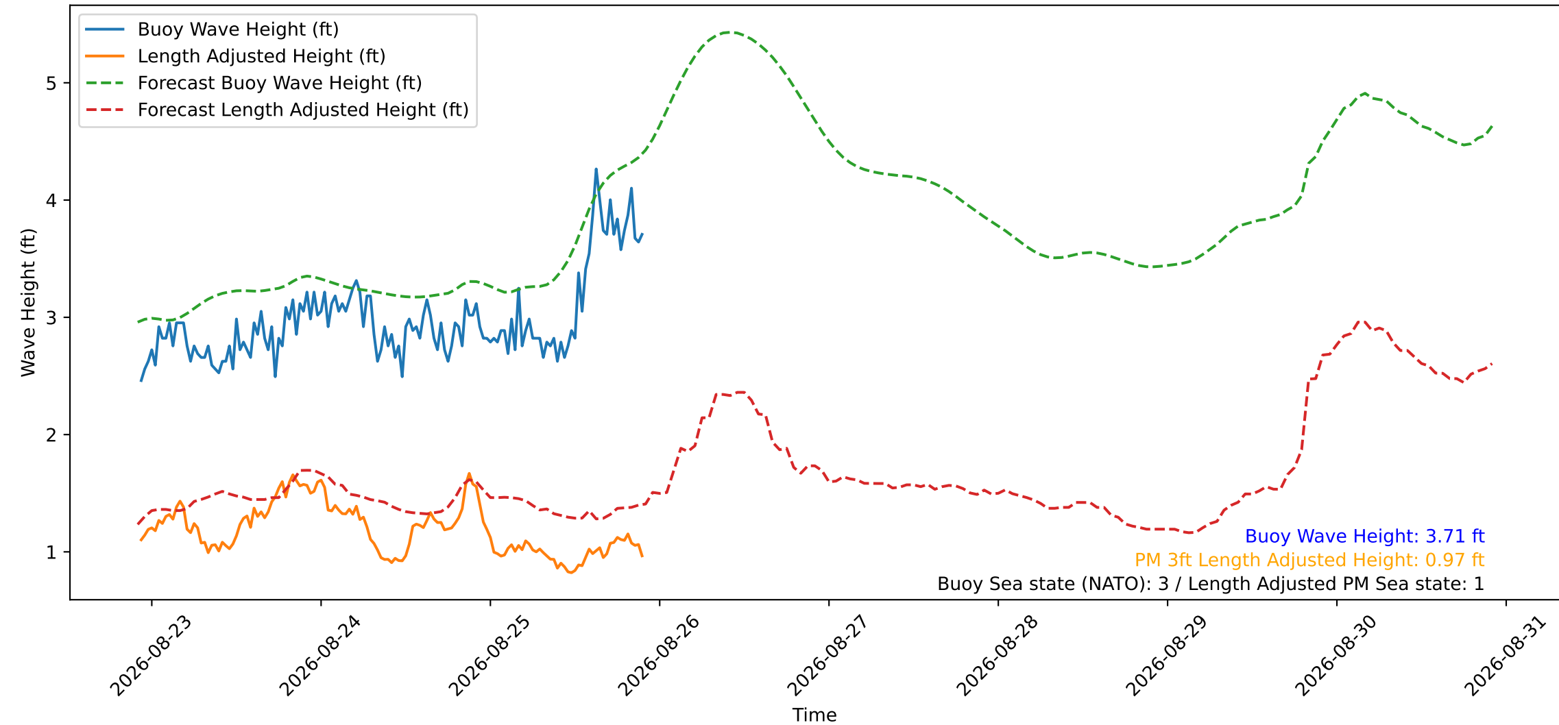
Wave Heights over Time for Green Beach at 2026-08-25 22:11:11
