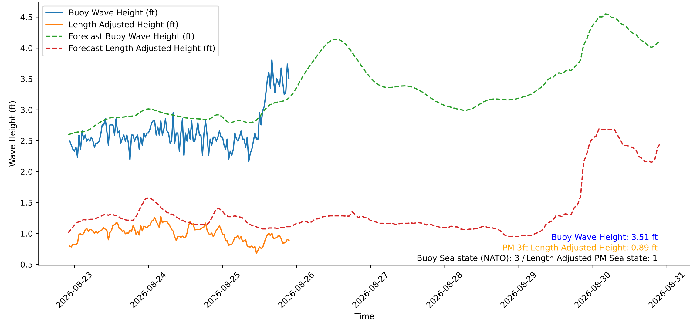
Wave Heights over Time for Red Beach at 2026-08-25 22:10:49
