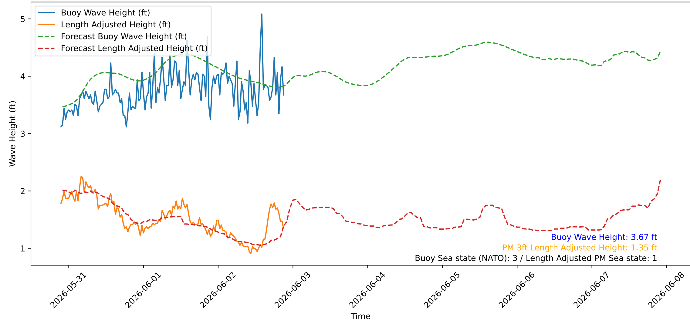
Wave Heights over Time for Oceanside Harbor at 2026-06-02 21:30:26
