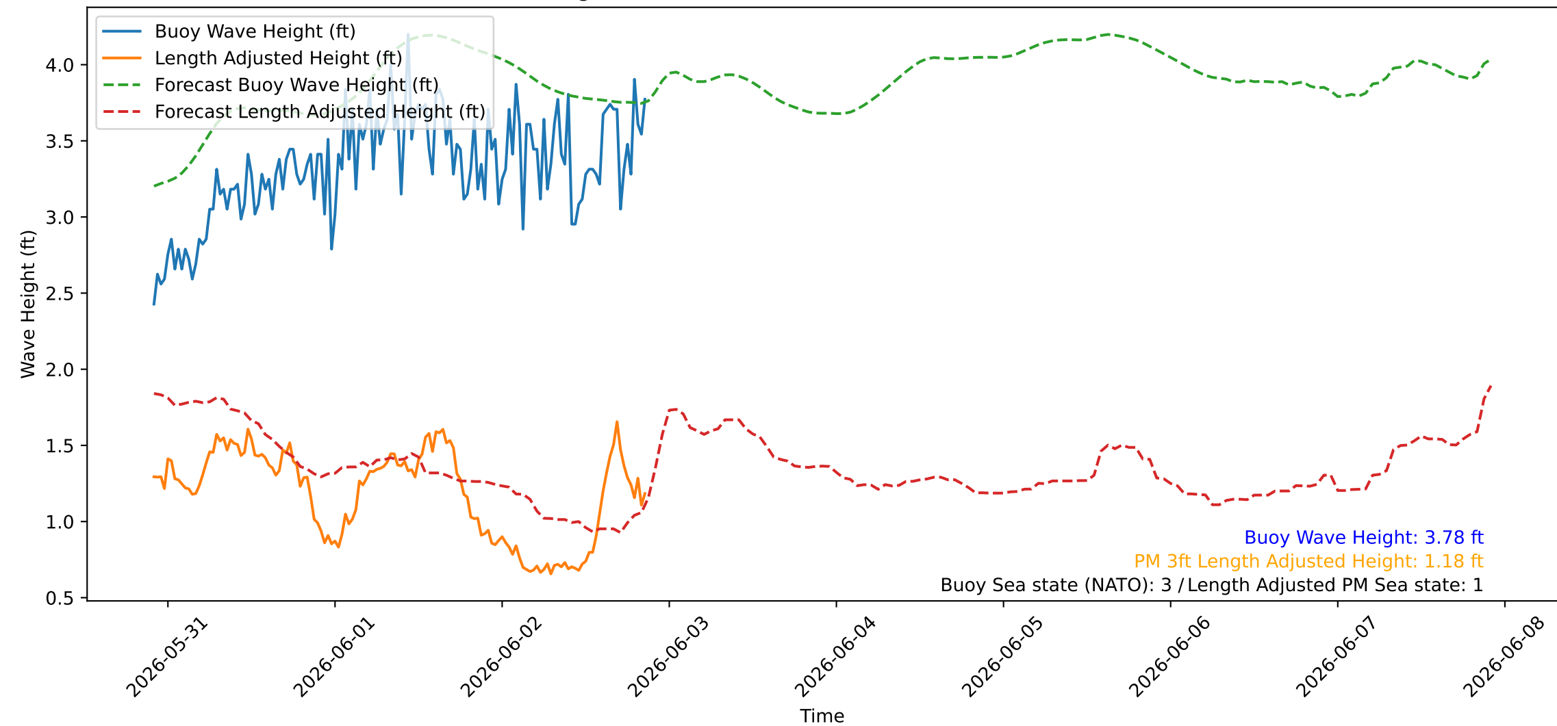
Wave Heights over Time for Red Beach at 2026-06-02 21:30:45
