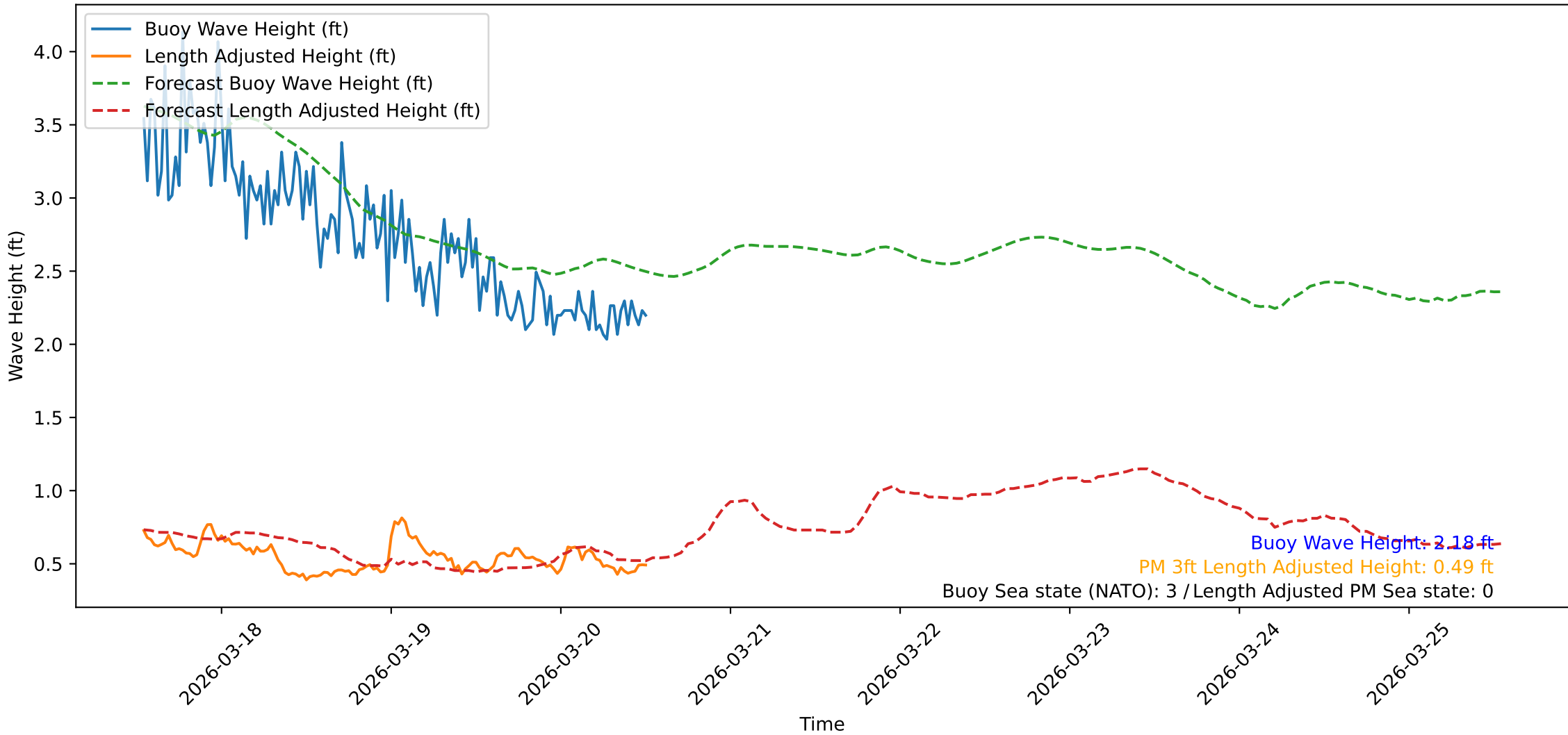
Wave Heights over Time for Green Beach at 2026-03-20 12:51:11
