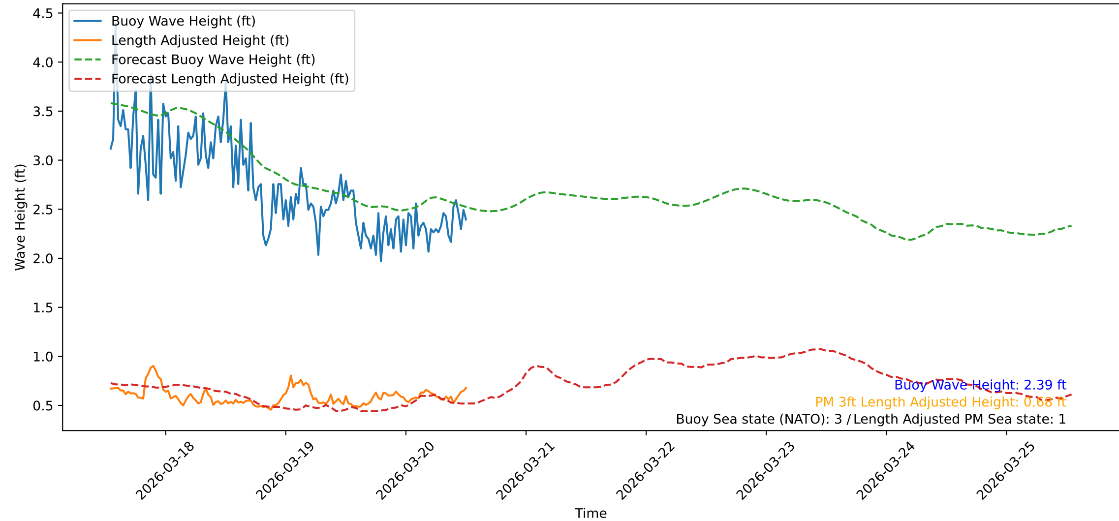
Wave Heights over Time for Oceanside Harbor at 2026-03-20 12:50:32
