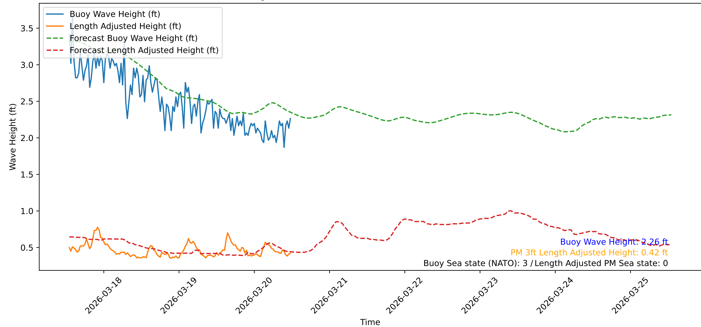
Wave Heights over Time for Red Beach at 2026-03-20 12:50:48
