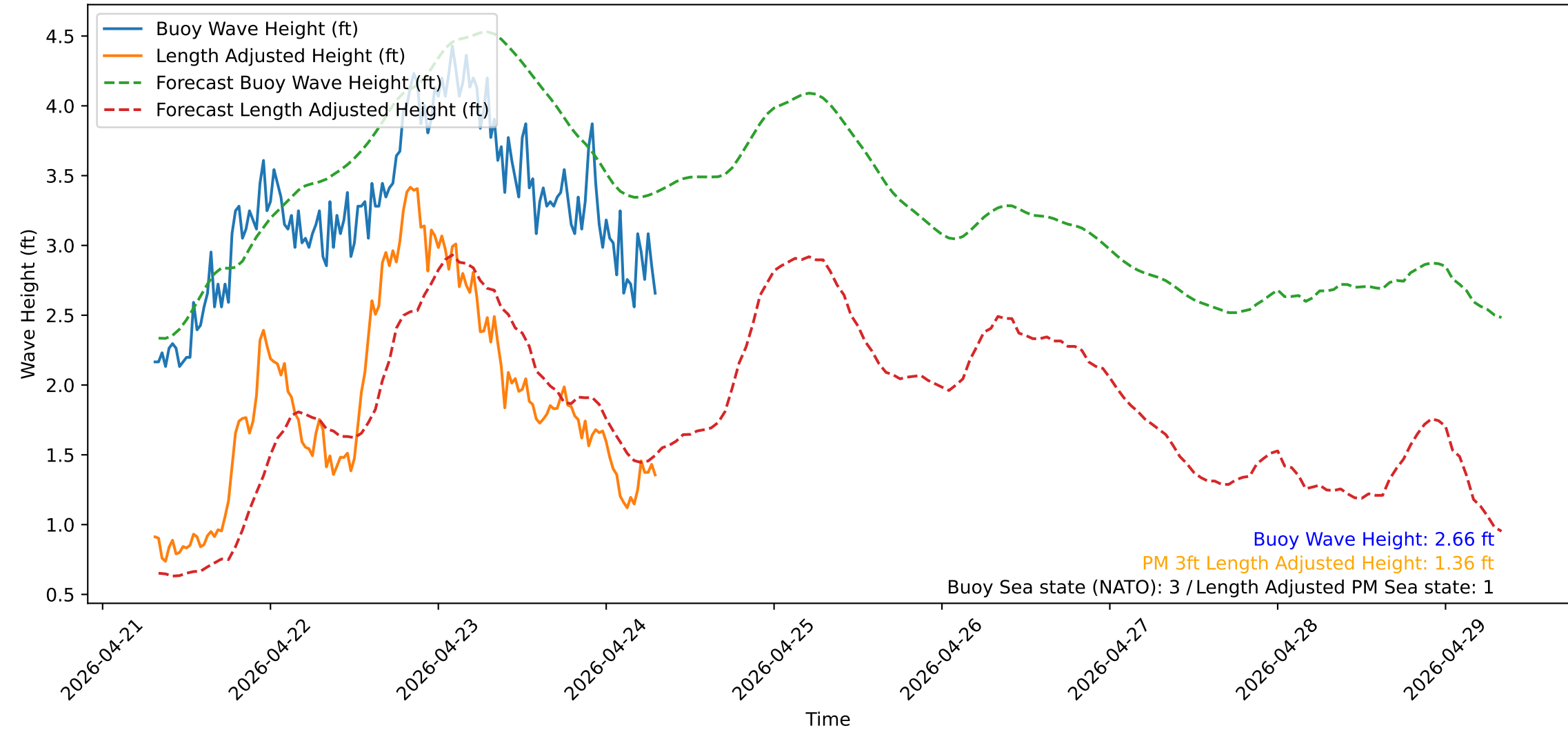
Wave Heights over Time for Oceanside Harbor at 2026-04-24 07:40:32
