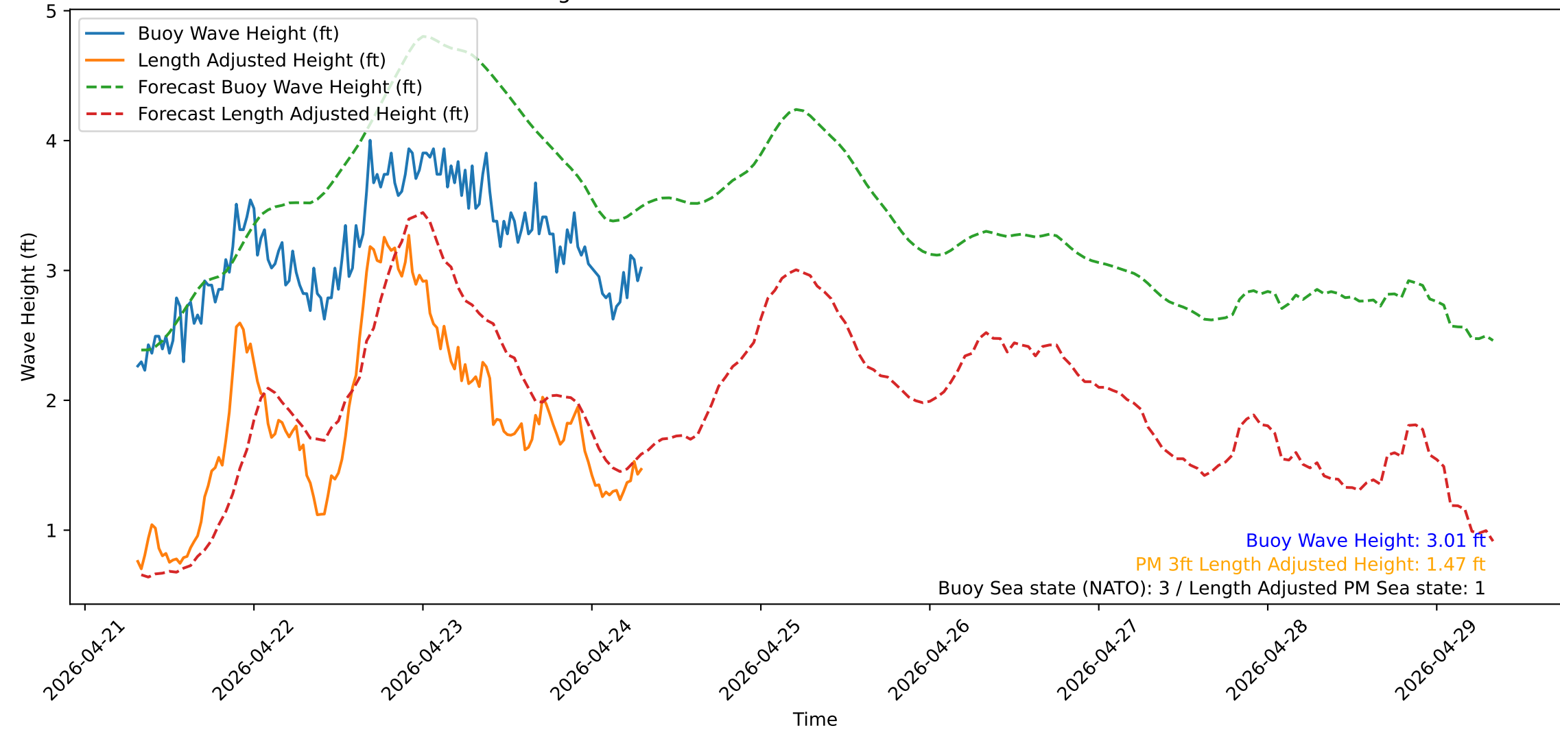
Wave Heights over Time for Green Beach at 2026-04-24 07:41:13
