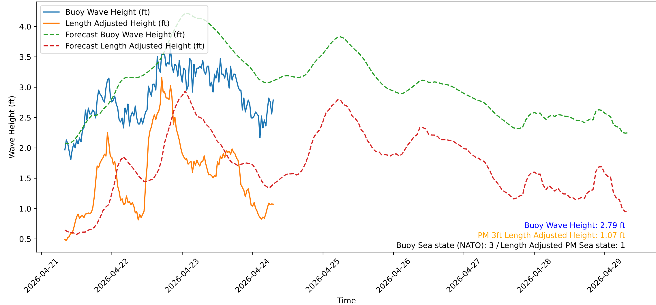
Wave Heights over Time for Red Beach at 2026-04-24 07:40:51
