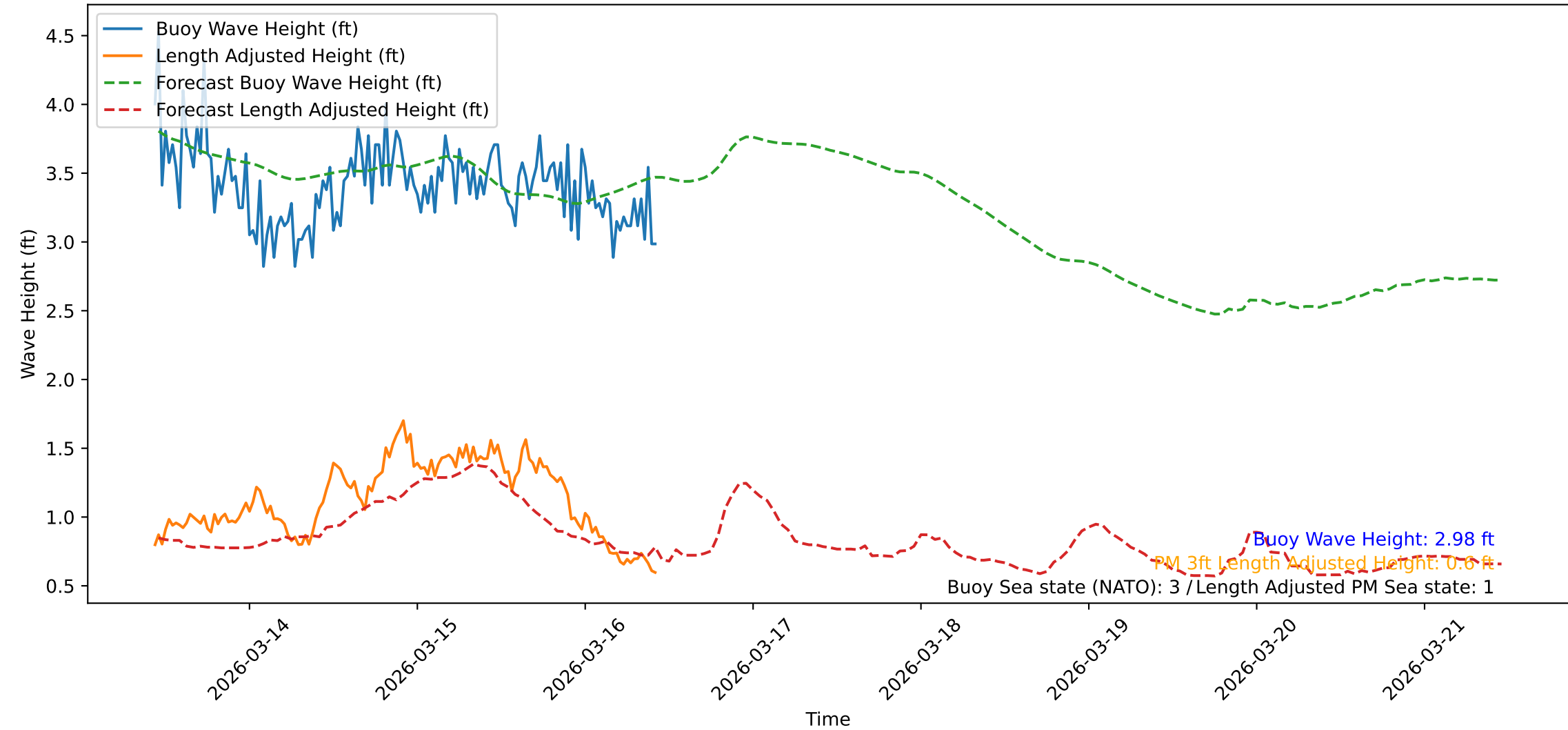
Wave Heights over Time for Green Beach at 2026-03-16 10:41:45
