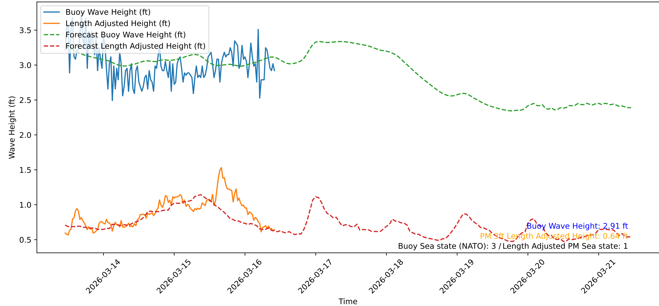
Wave Heights over Time for Red Beach at 2026-03-16 10:41:11
