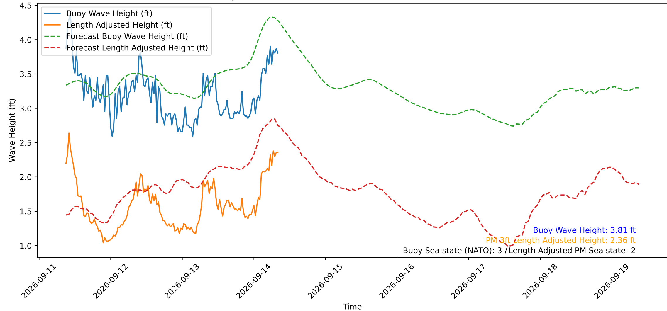
Wave Heights over Time for Oceanside Harbor at 2026-09-14 09:00:30
