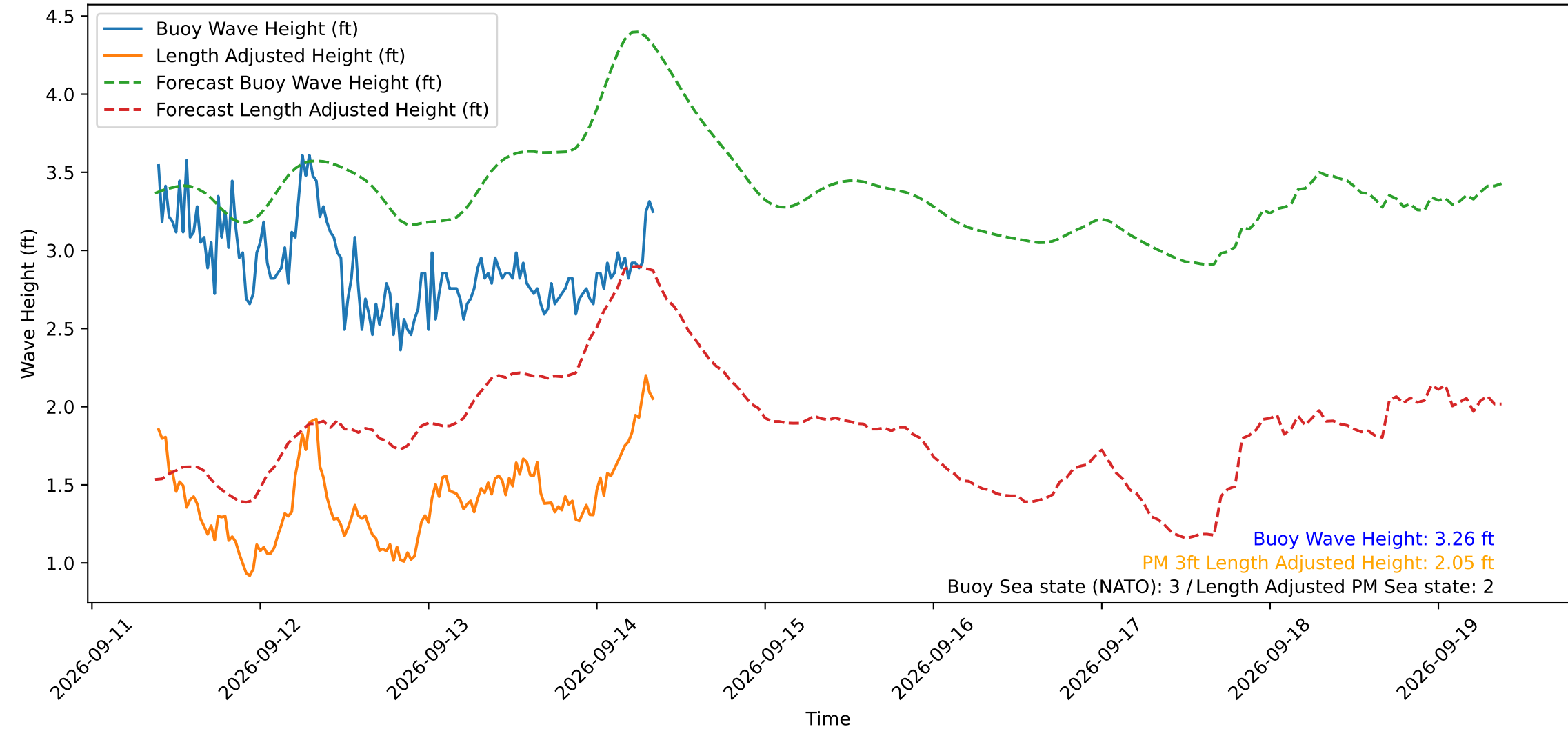
Wave Heights over Time for Green Beach at 2026-09-14 09:01:12
