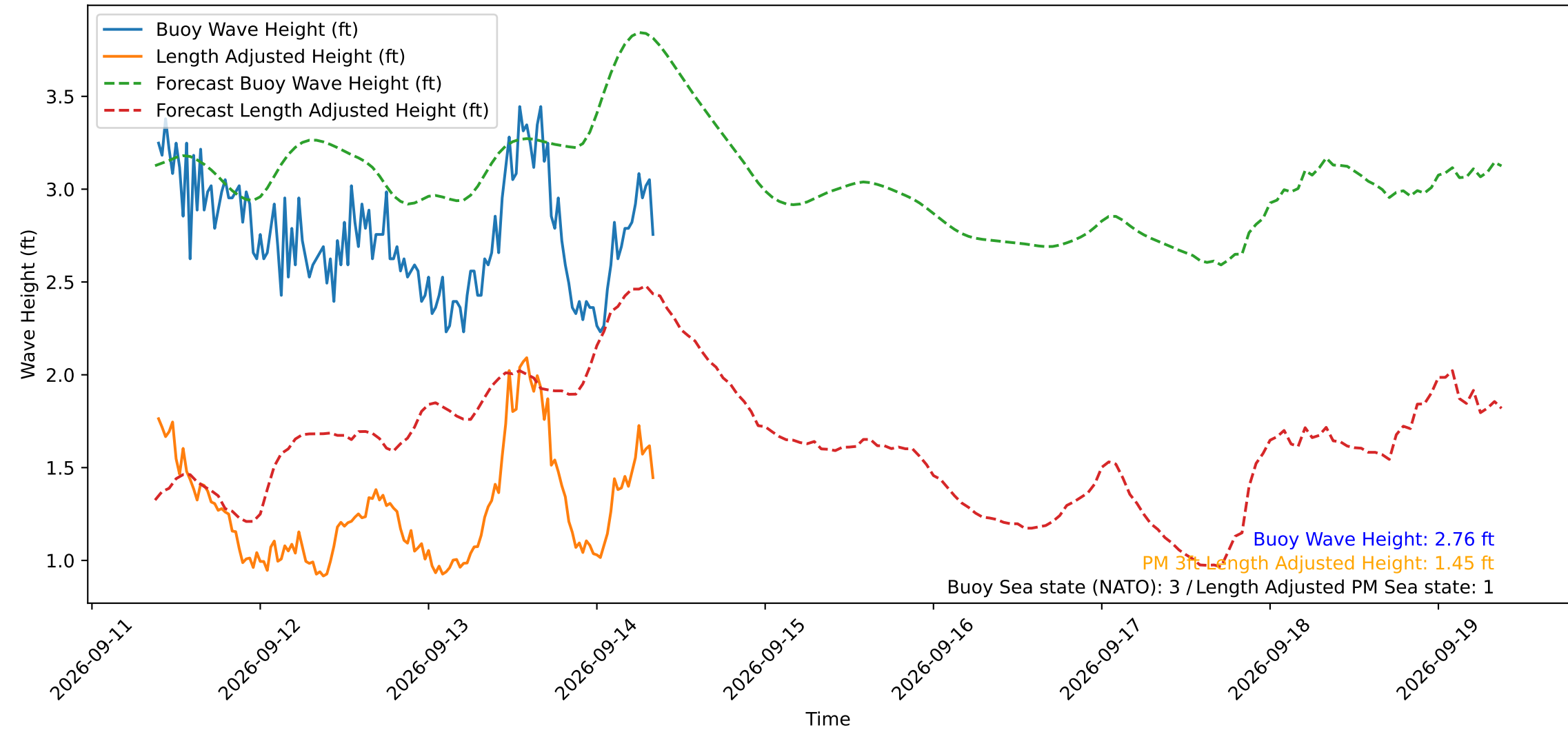
Wave Heights over Time for Red Beach at 2026-09-14 09:00:49
