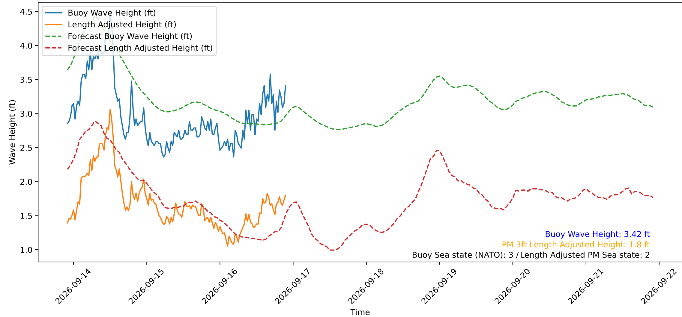
Wave Heights over Time for Oceanside Harbor at 2026-09-16 22:10:29
