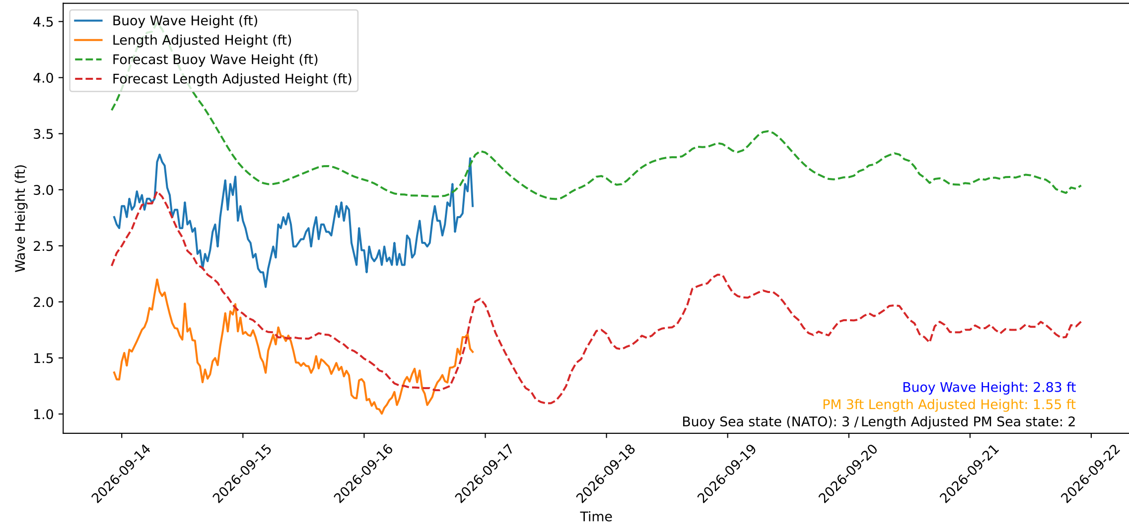
Wave Heights over Time for Green Beach at 2026-09-16 22:11:12
