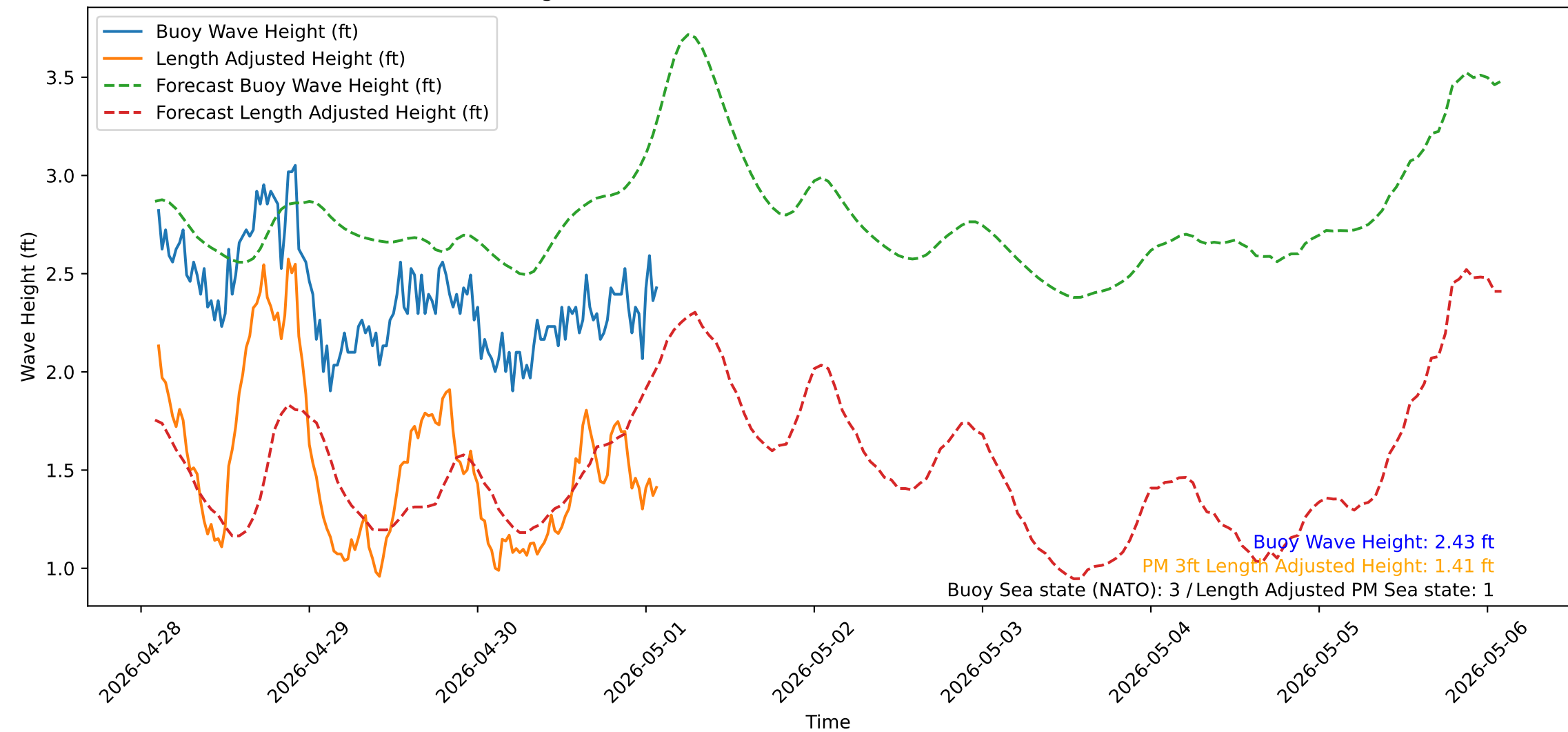
Wave Heights over Time for Oceanside Harbor at 2026-05-01 02:20:30
