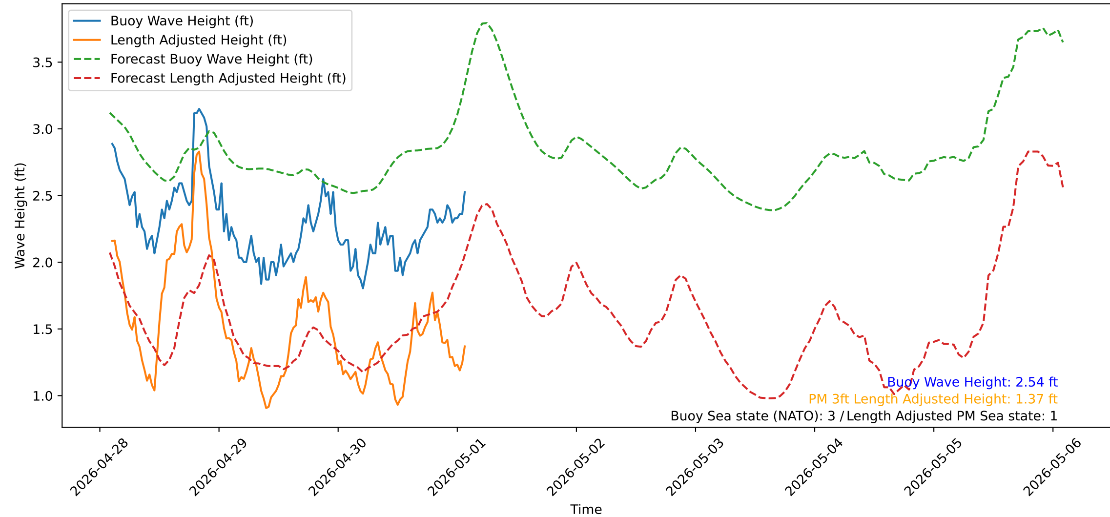
Wave Heights over Time for Green Beach at 2026-05-01 02:21:13
