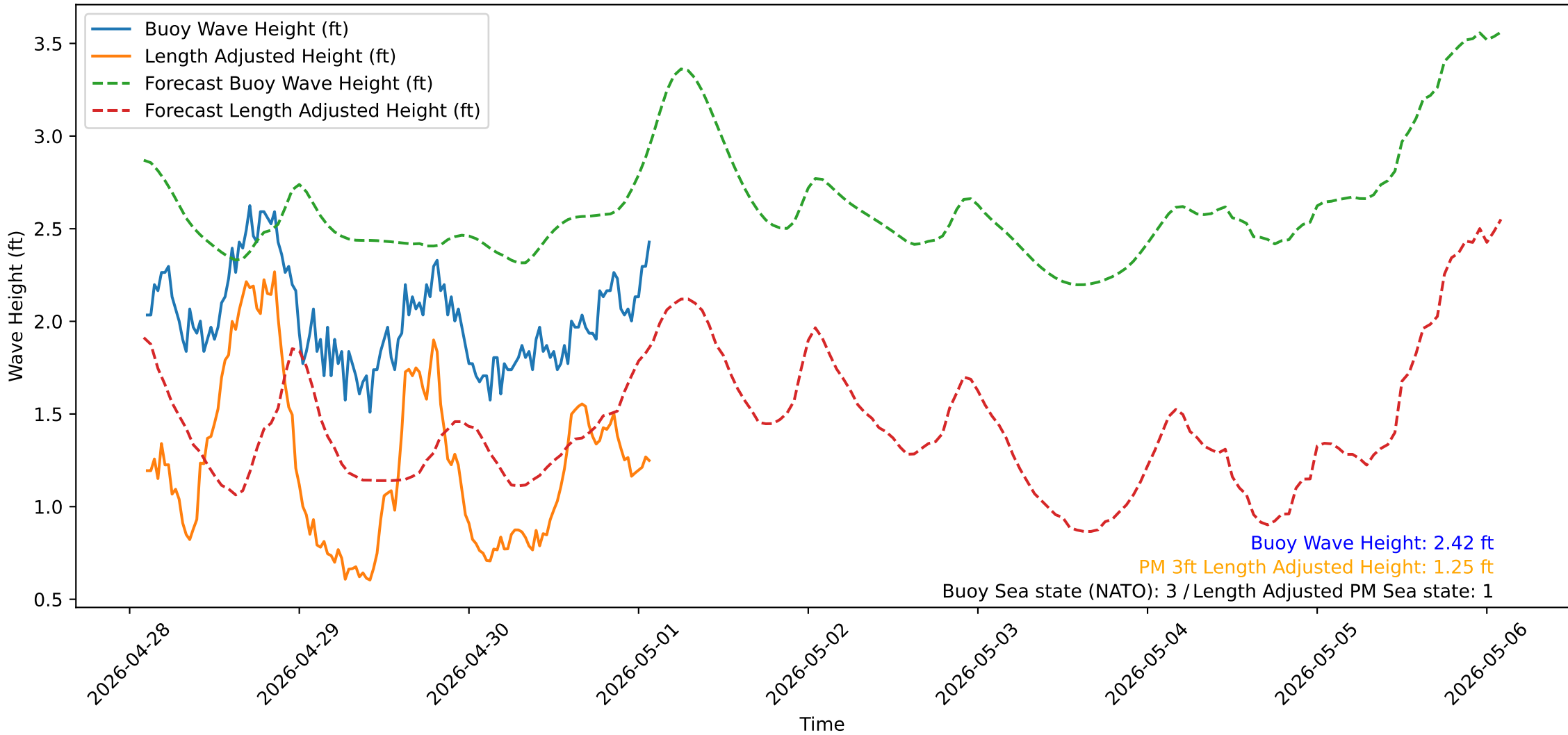
Wave Heights over Time for Red Beach at 2026-05-01 02:20:51
