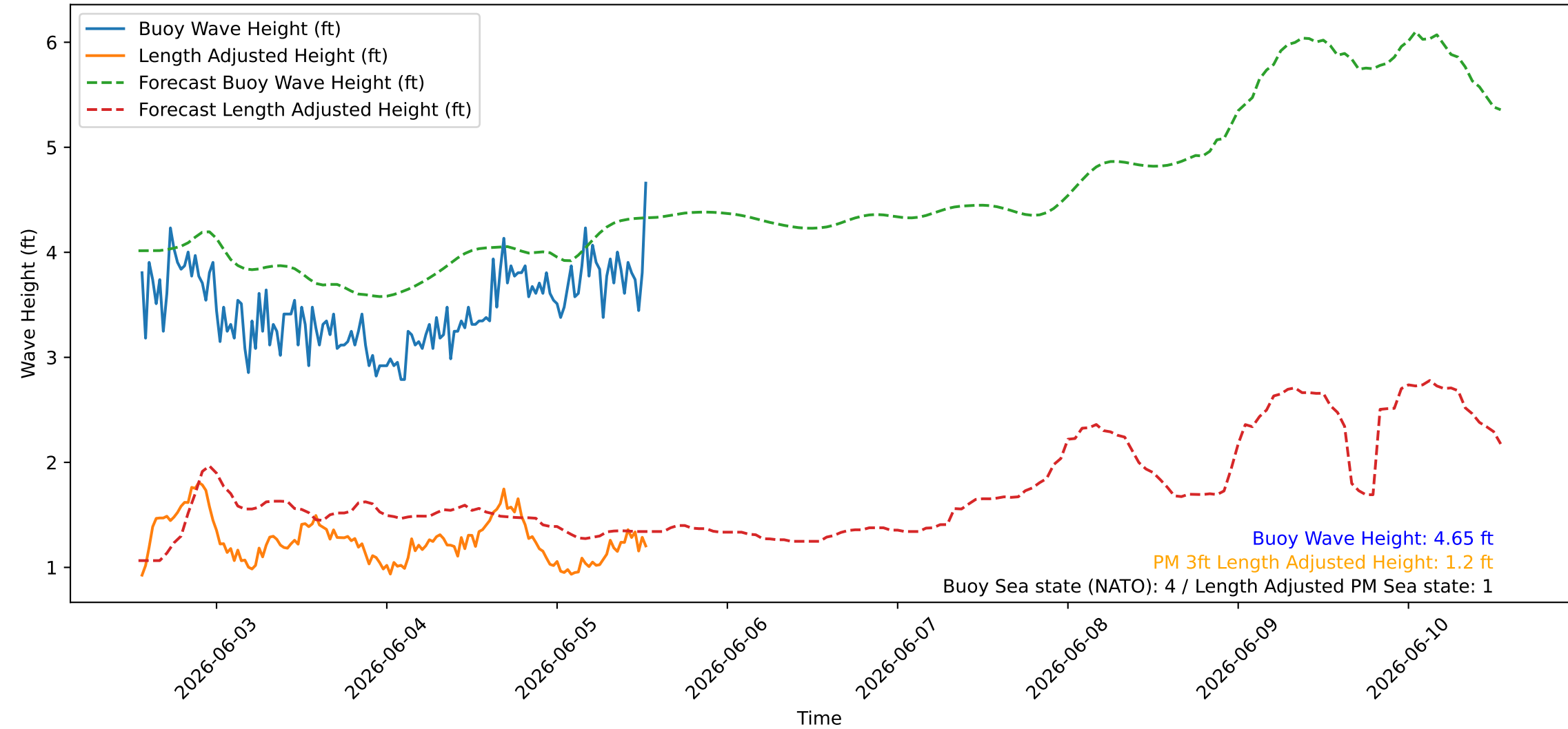
Wave Heights over Time for Green Beach at 2026-06-05 13:21:09
