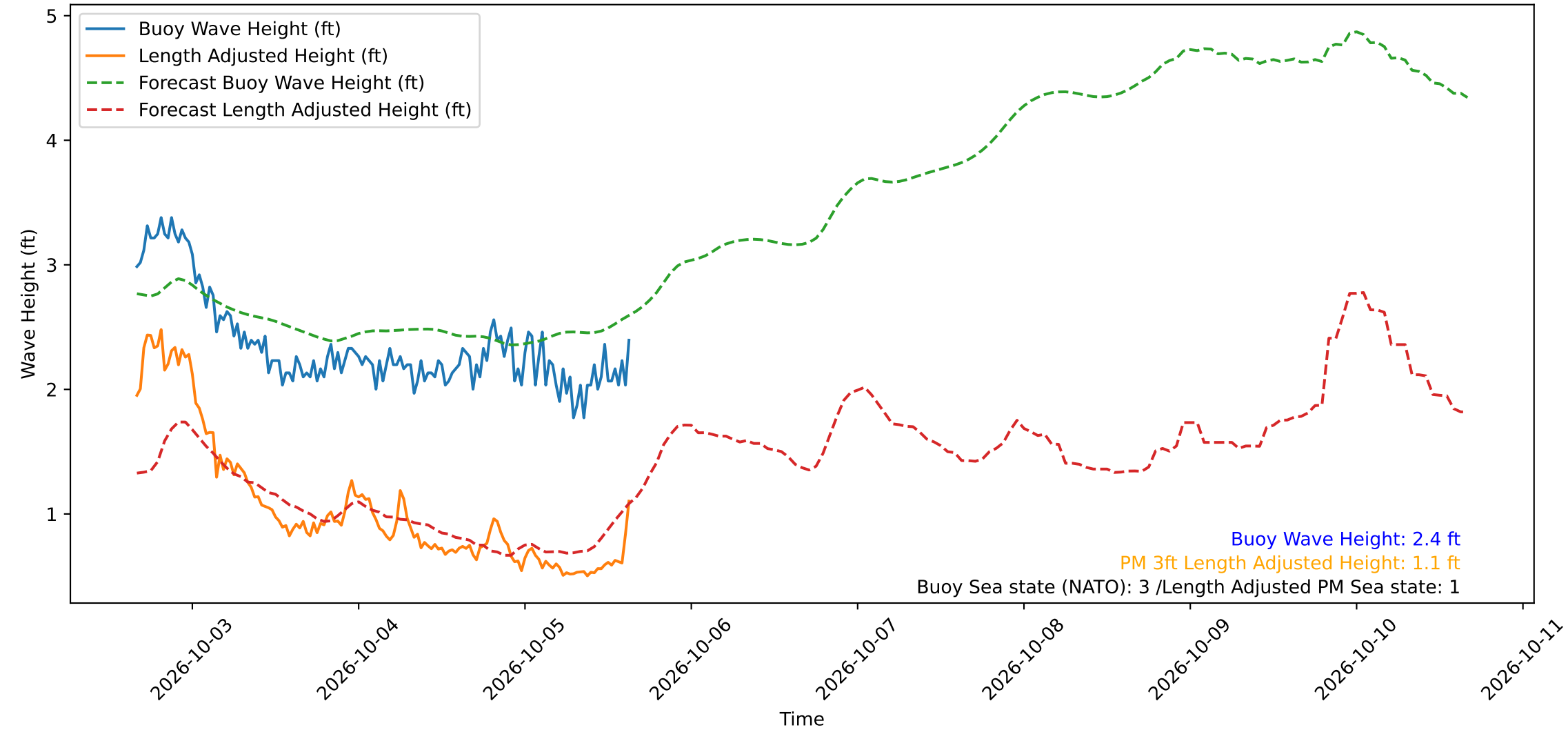
Wave Heights over Time for Green Beach at 2026-10-05 15:41:11
