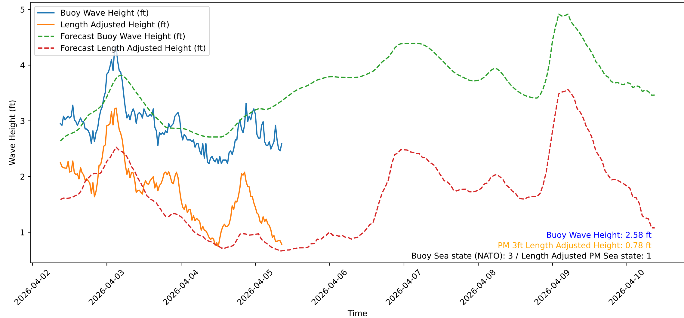
Wave Heights over Time for Green Beach at 2026-04-05 09:11:11
