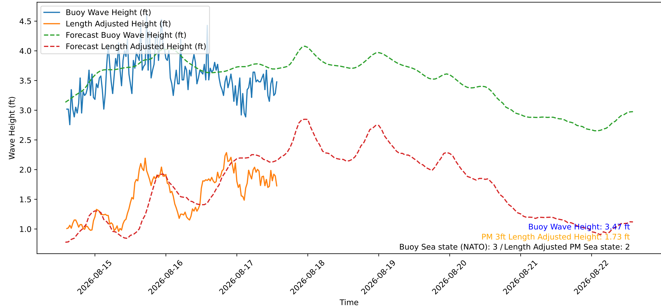
Wave Heights over Time for Oceanside Harbor at 2026-08-17 14:20:26
