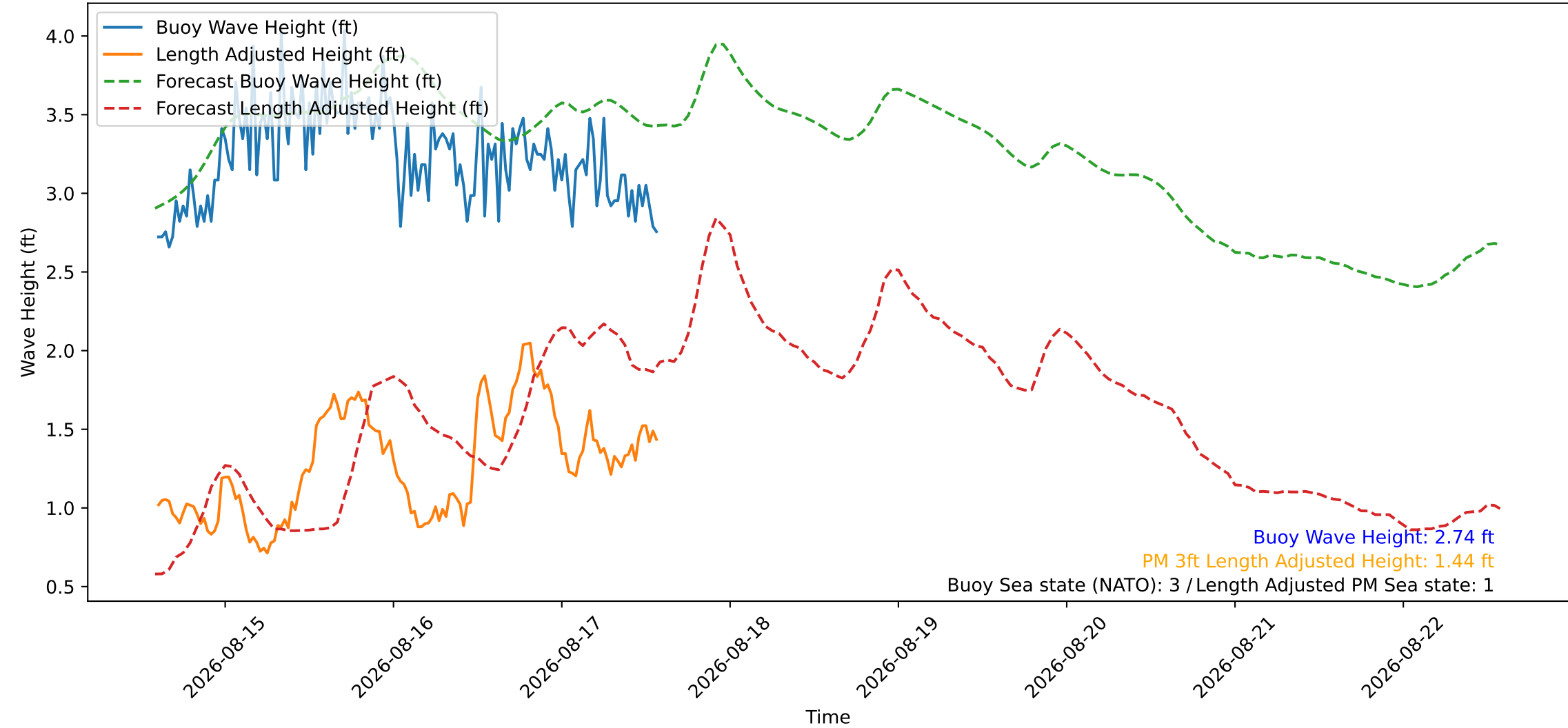
Wave Heights over Time for Red Beach at 2026-08-17 14:20:47
