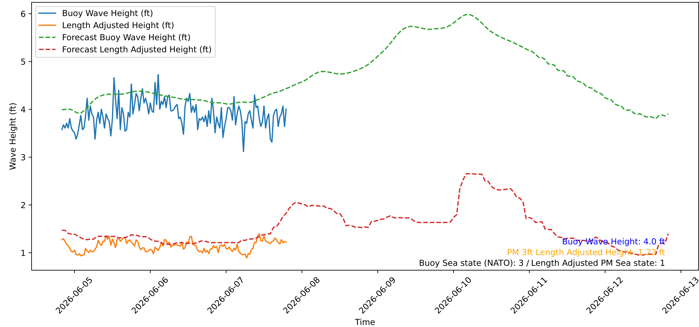
Wave Heights over Time for Green Beach at 2026-06-07 19:51:09
