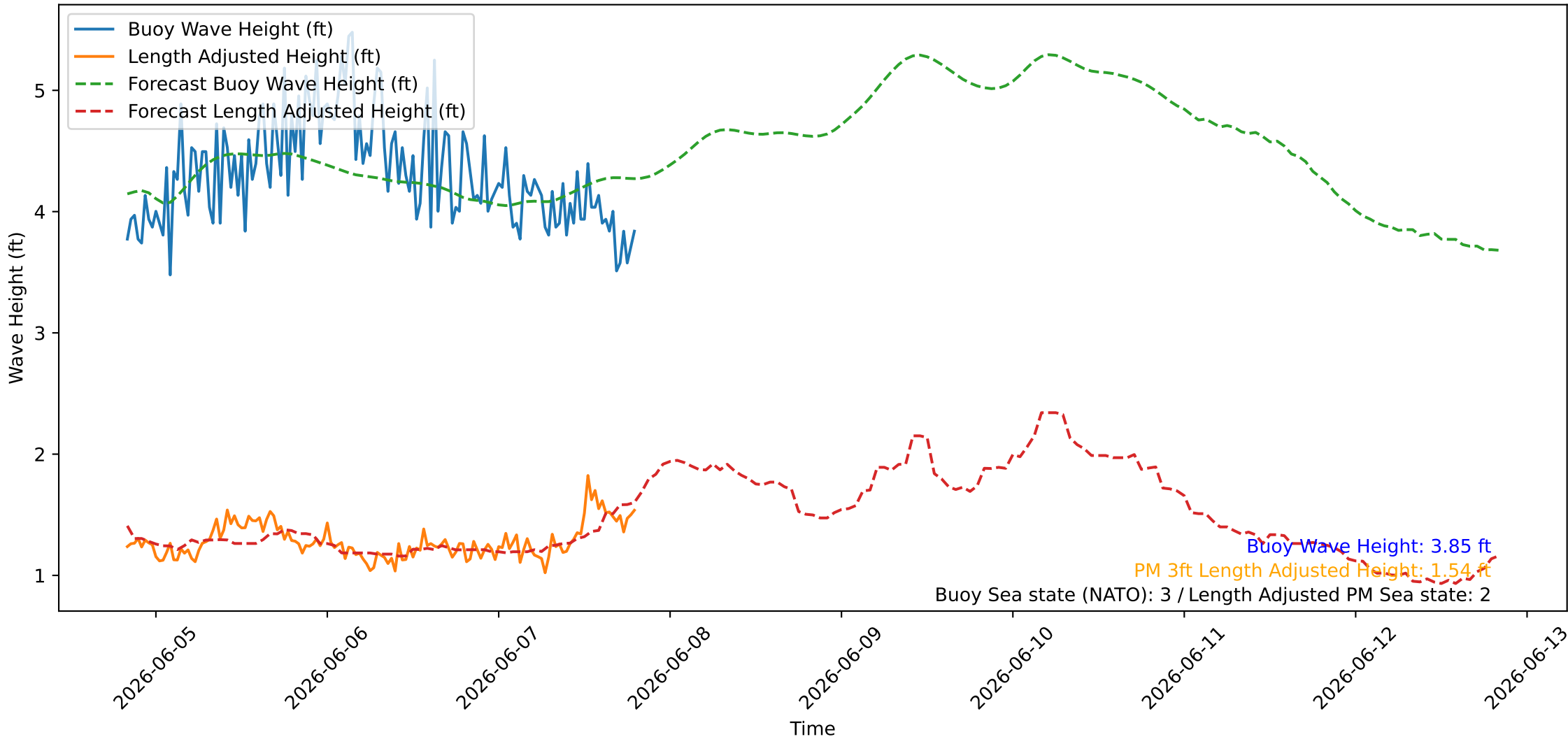
Wave Heights over Time for Oceanside Harbor at 2026-06-07 19:50:25
