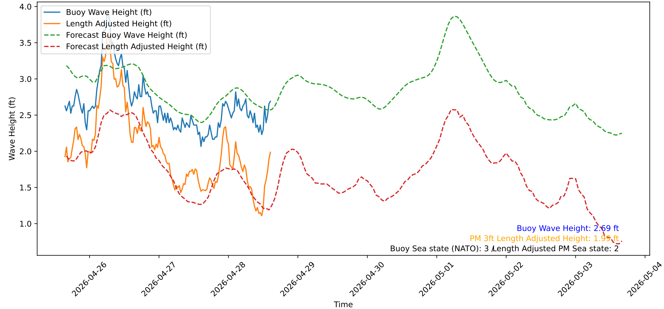
Wave Heights over Time for Oceanside Harbor at 2026-04-28 15:30:32
