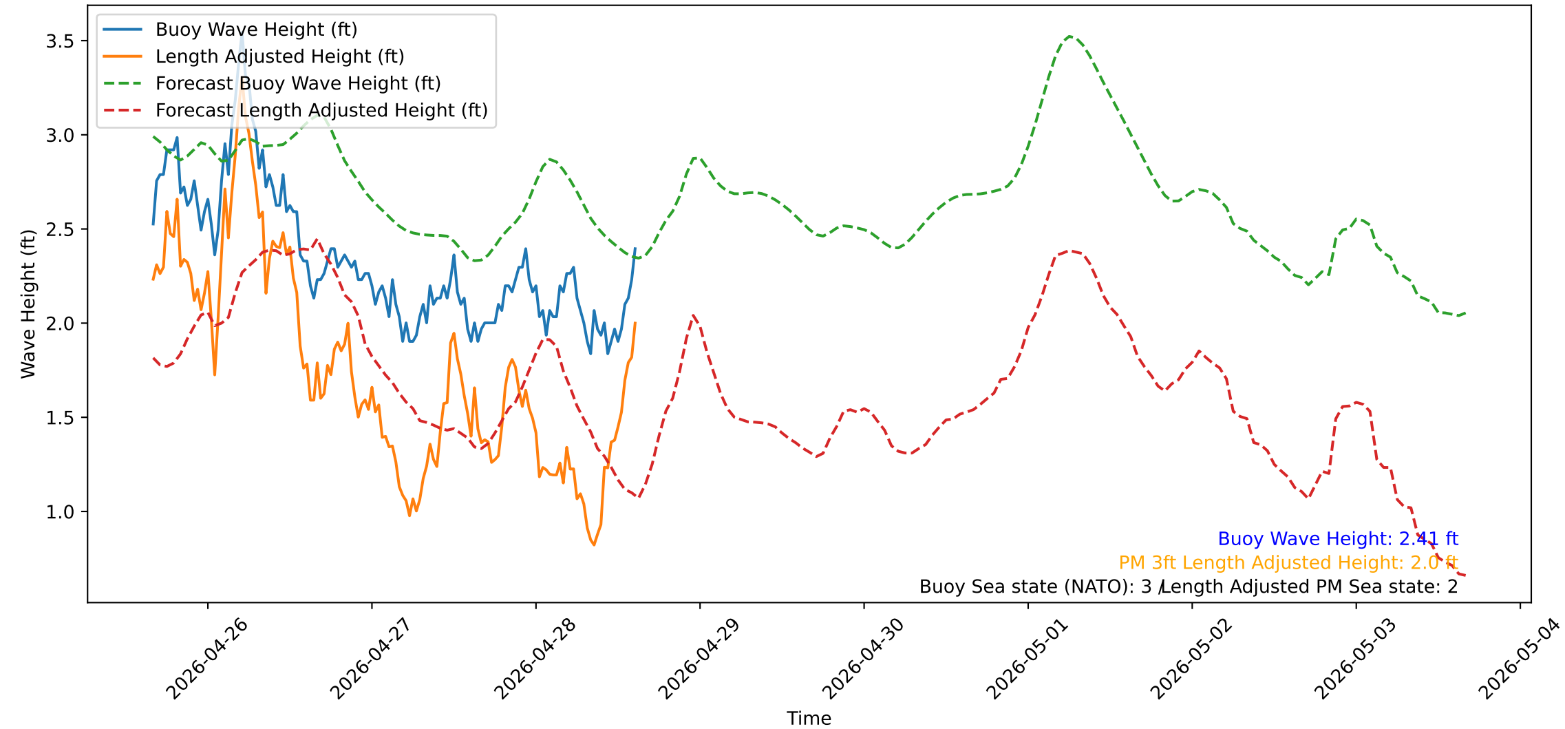
Wave Heights over Time for Red Beach at 2026-04-28 15:30:51
