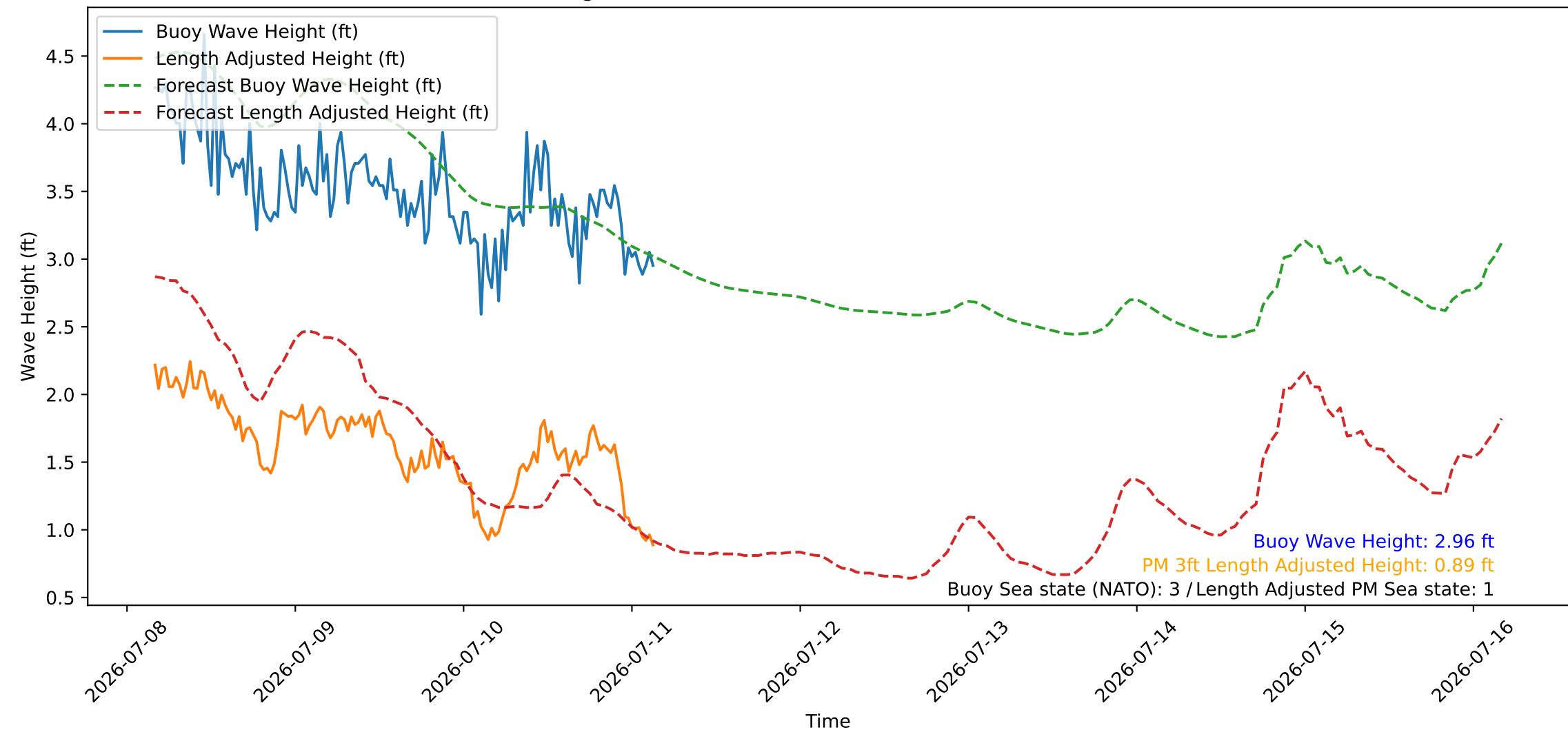
Wave Heights over Time for Red Beach at 2026-07-11 03:50:46
