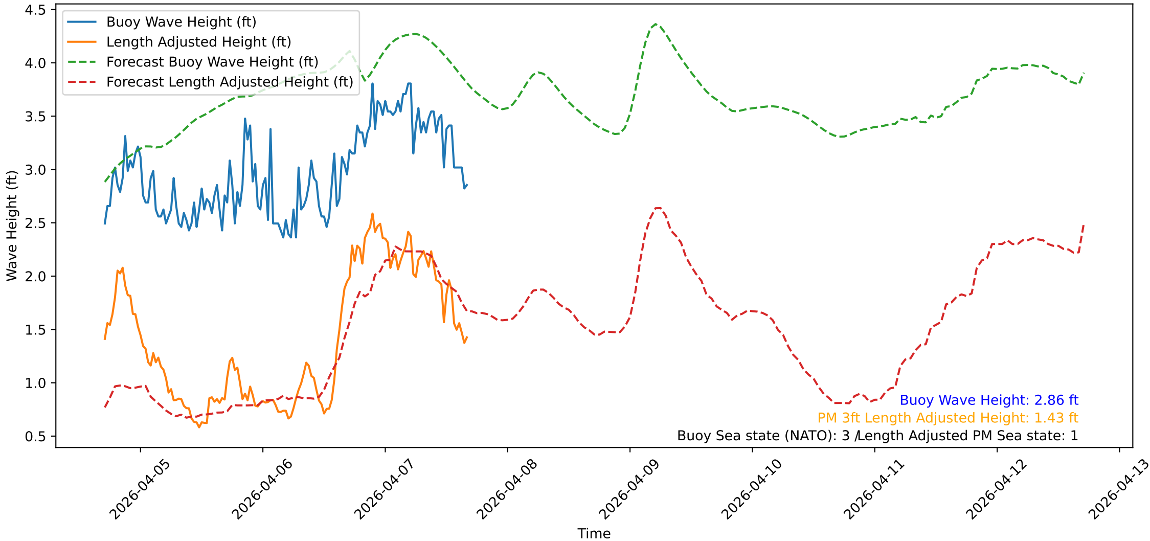
Wave Heights over Time for Green Beach at 2026-04-07 17:01:10
