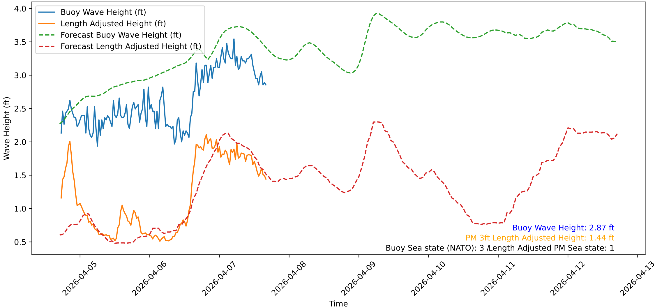
Wave Heights over Time for Red Beach at 2026-04-07 17:00:48
