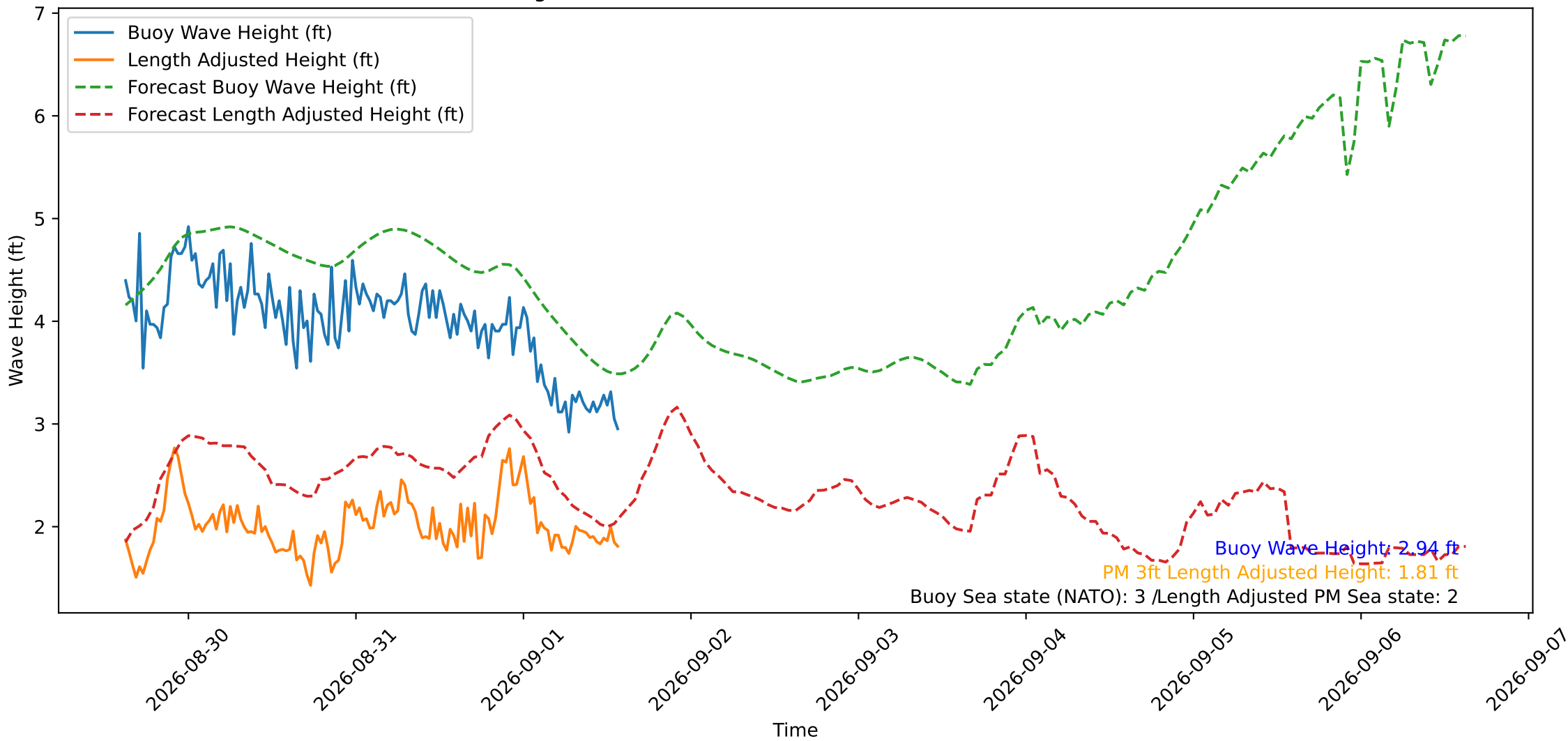
Wave Heights over Time for Green Beach at 2026-09-01 14:31:13
