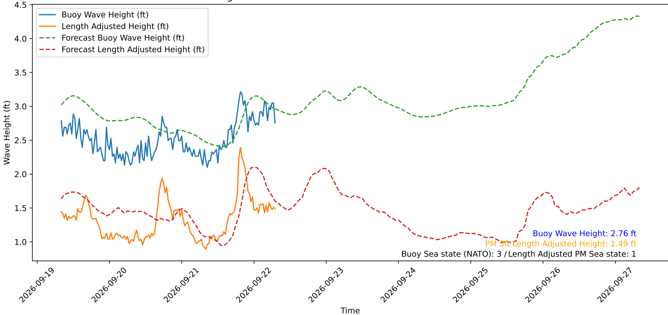
Wave Heights over Time for Oceanside Harbor at 2026-09-22 07:50:29
