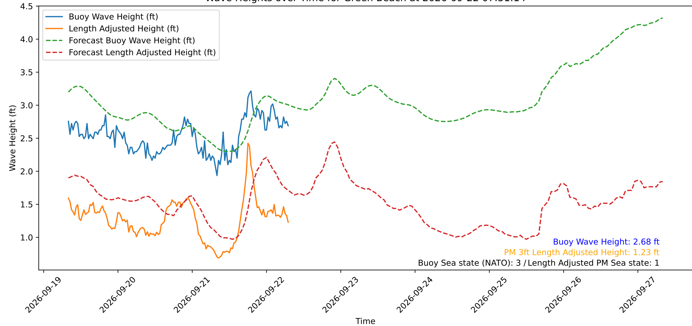
Wave Heights over Time for Green Beach at 2026-09-22 07:51:14
