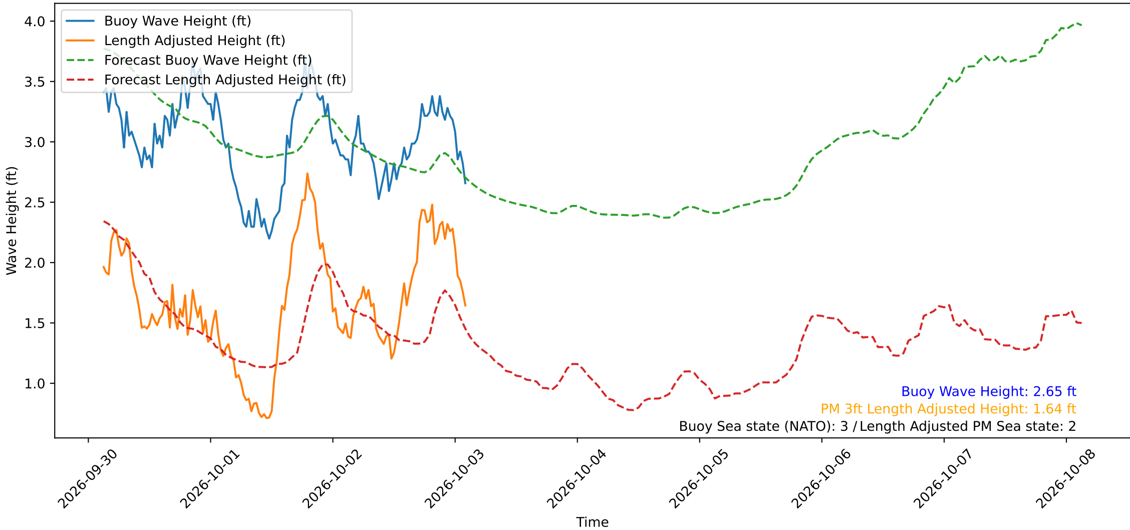
Wave Heights over Time for Green Beach at 2026-10-03 02:51:15
