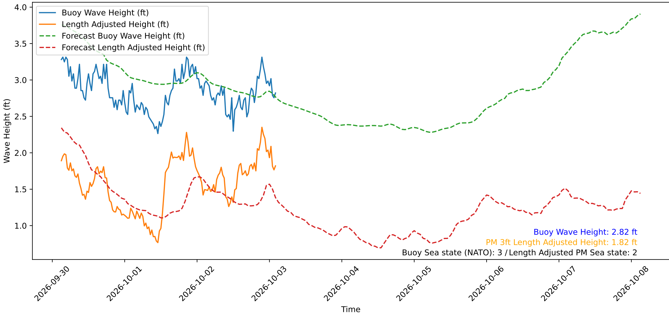
Wave Heights over Time for Oceanside Harbor at 2026-10-03 02:50:30
