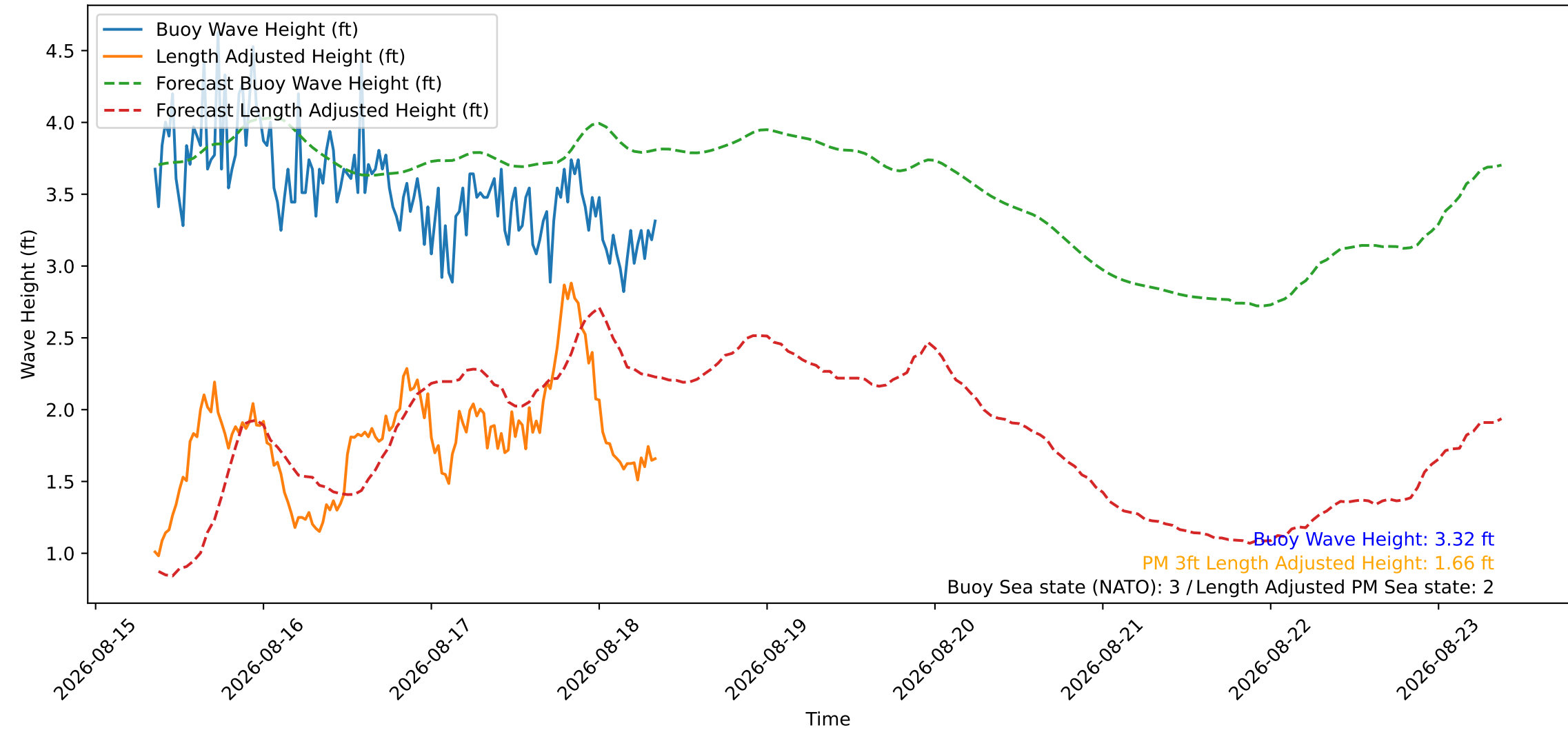
Wave Heights over Time for Oceanside Harbor at 2026-08-18 08:40:26
