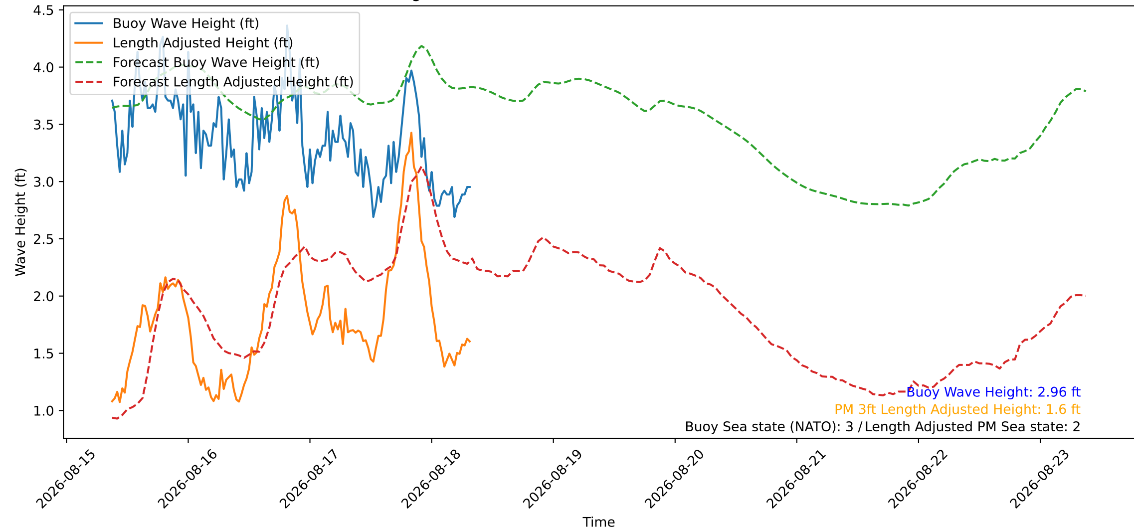
Wave Heights over Time for Green Beach at 2026-08-18 08:41:09
