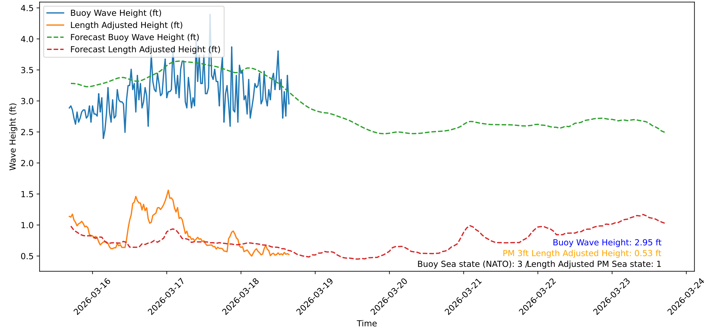
Wave Heights over Time for Oceanside Harbor at 2026-03-18 16:30:31
