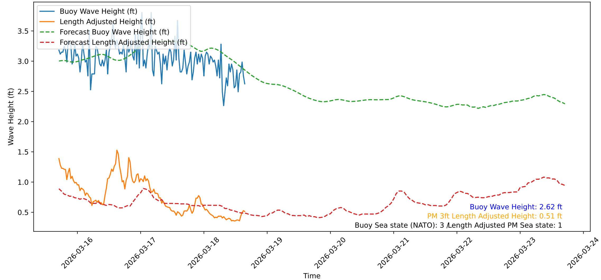
Wave Heights over Time for Red Beach at 2026-03-18 16:30:47
