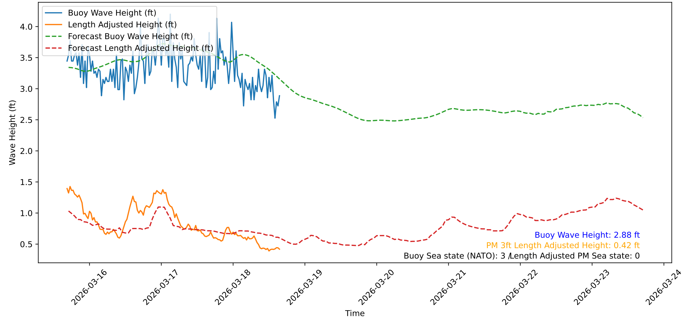
Wave Heights over Time for Green Beach at 2026-03-18 16:31:10
