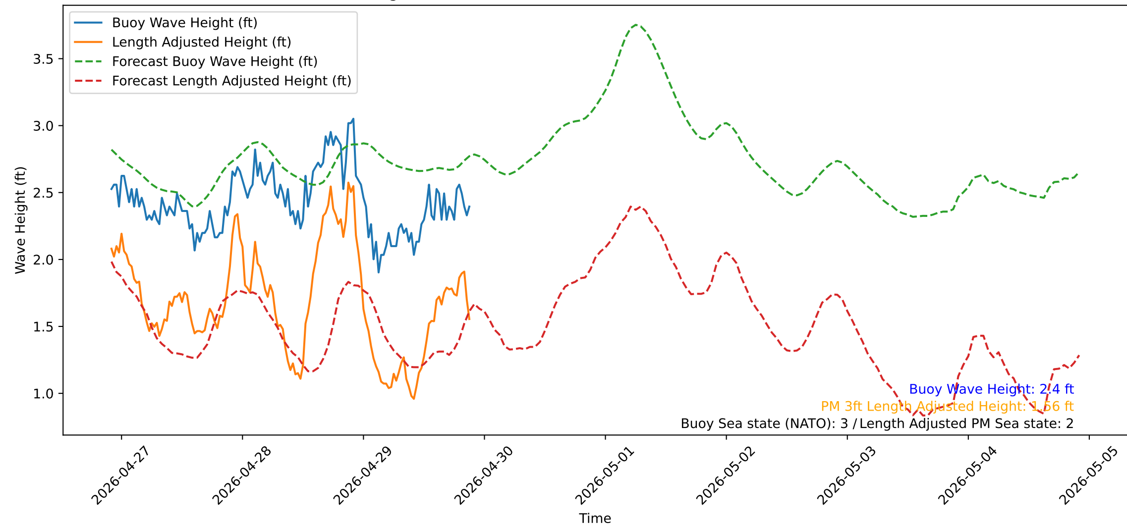
Wave Heights over Time for Oceanside Harbor at 2026-04-29 21:50:32
