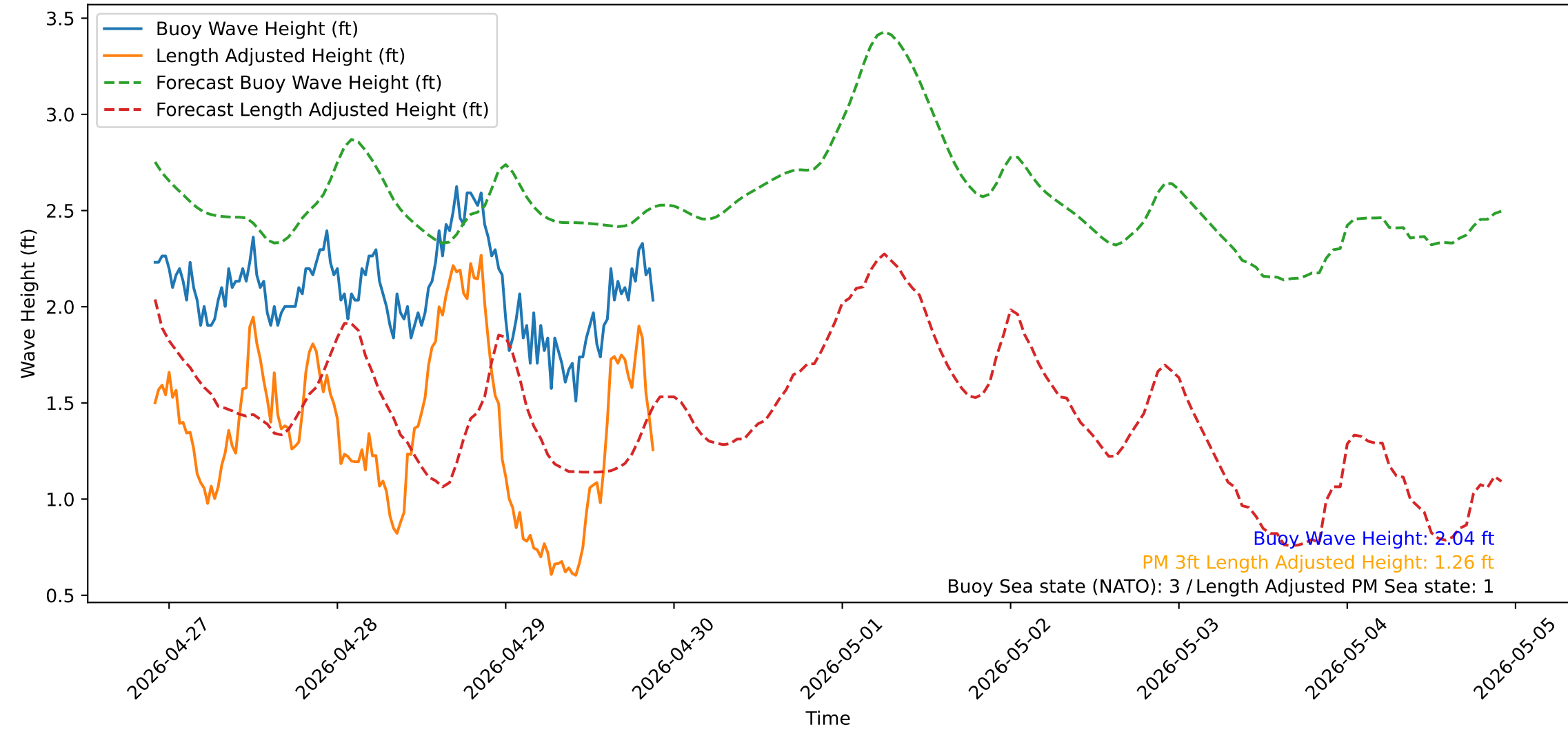
Wave Heights over Time for Red Beach at 2026-04-29 21:50:52
