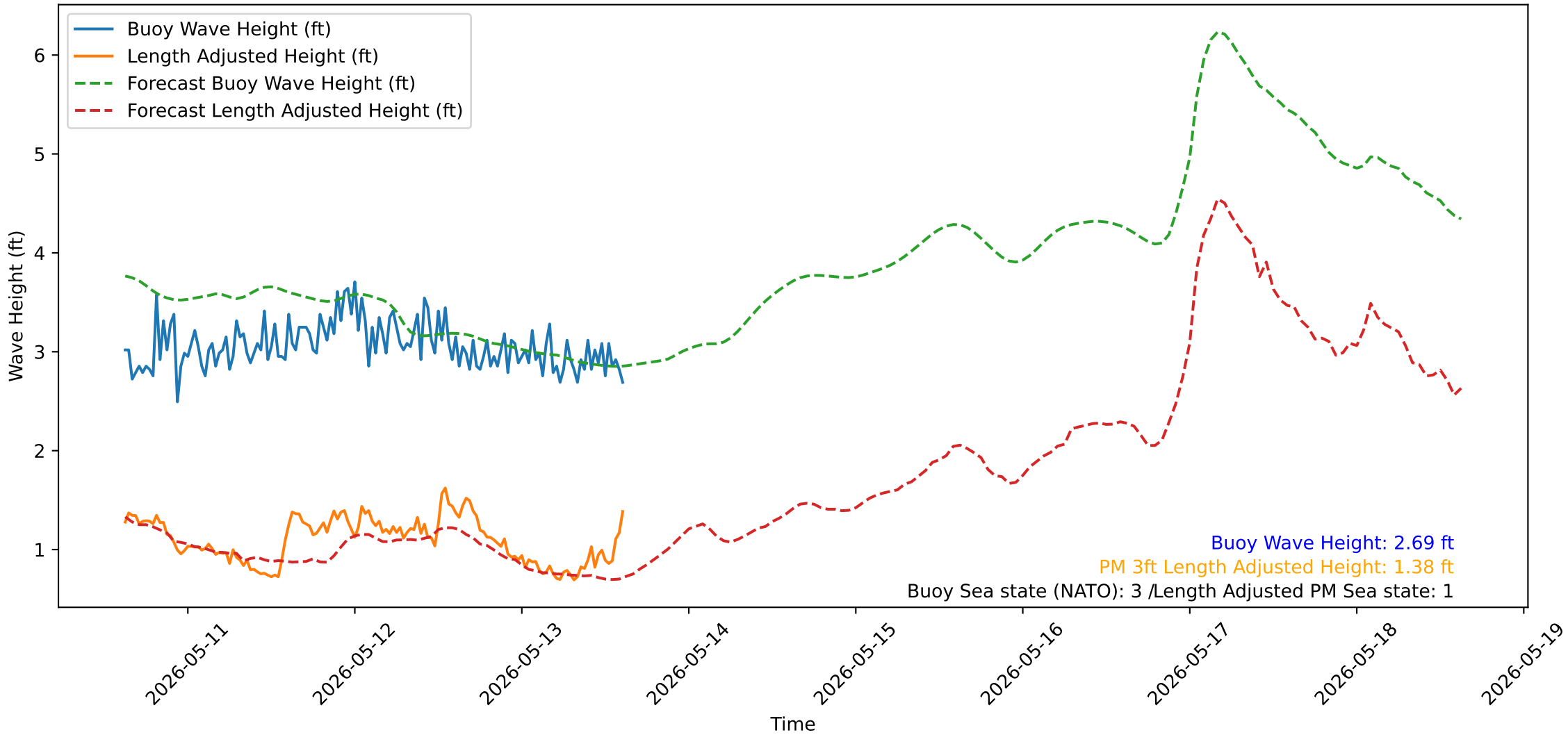
Wave Heights over Time for Oceanside Harbor at 2026-05-13 15:00:32
