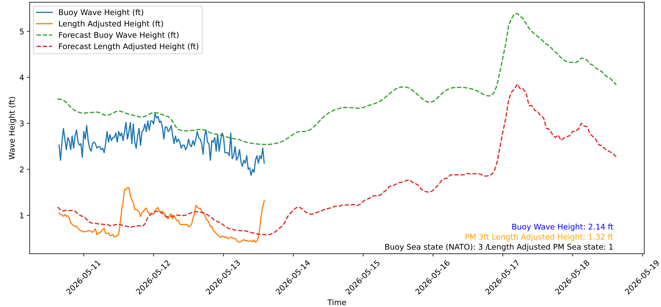
Wave Heights over Time for Red Beach at 2026-05-13 15:00:51
