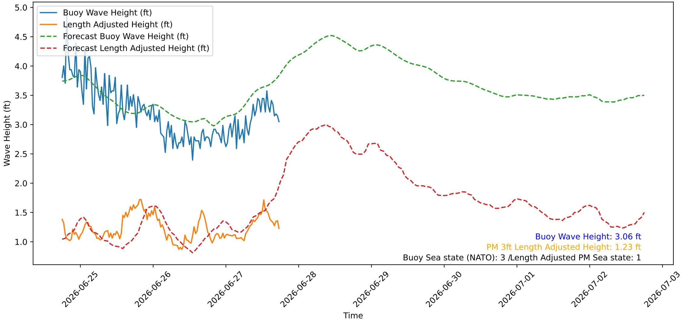
Wave Heights over Time for Oceanside Harbor at 2026-06-27 18:10:26
