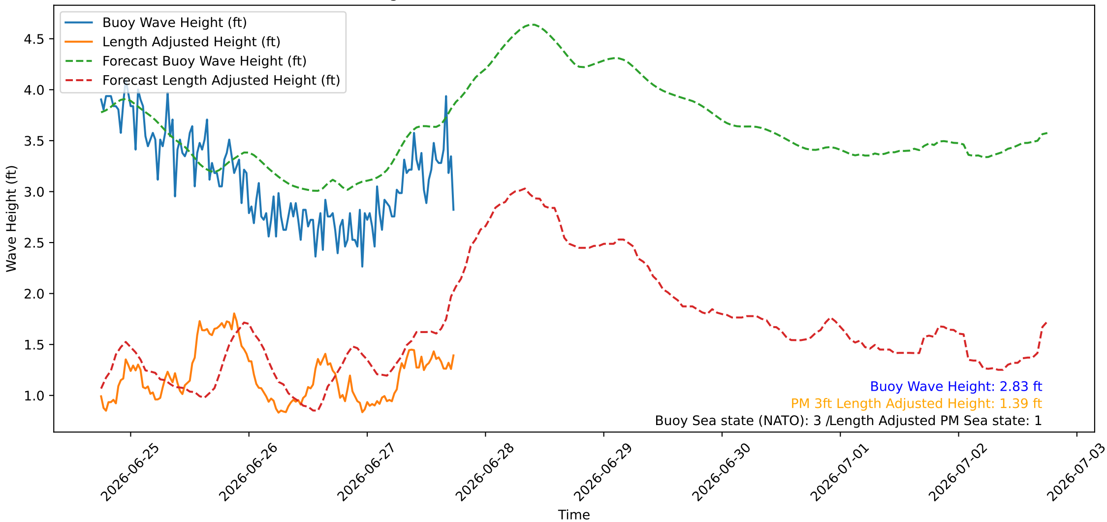
Wave Heights over Time for Green Beach at 2026-06-27 18:11:07
