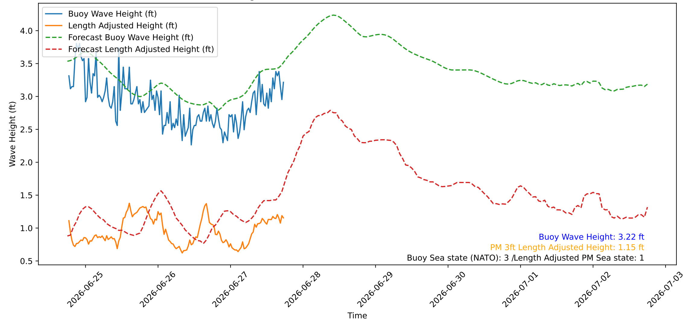
Wave Heights over Time for Red Beach at 2026-06-27 18:10:45
