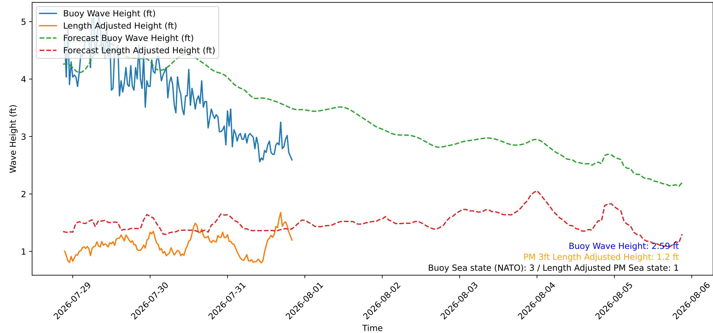
Wave Heights over Time for Red Beach at 2026-07-31 21:00:46
