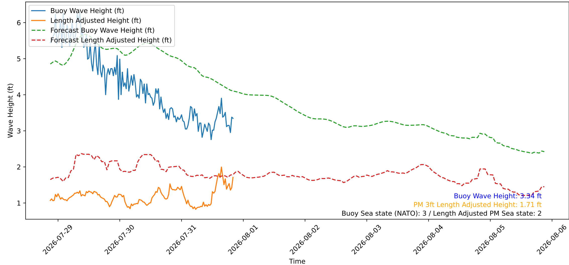
Wave Heights over Time for Green Beach at 2026-07-31 21:01:09
