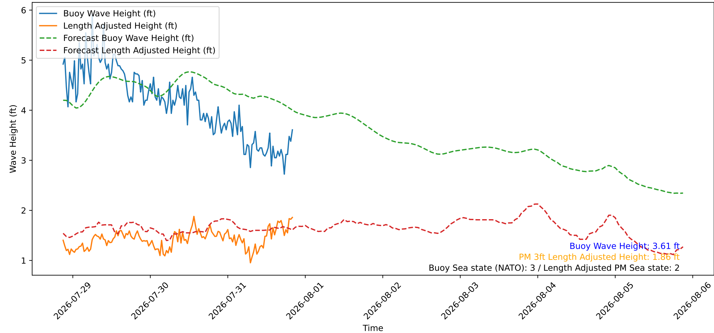
Wave Heights over Time for Oceanside Harbor at 2026-07-31 21:00:26
