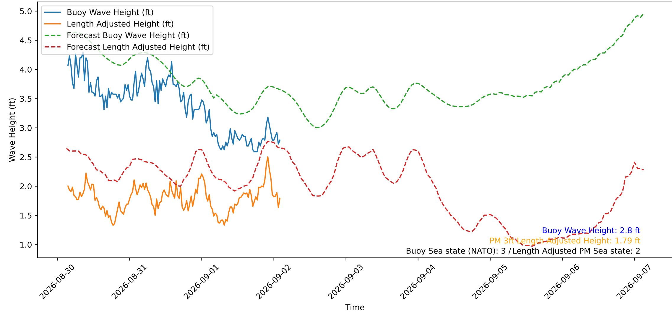
Wave Heights over Time for Red Beach at 2026-09-02 03:00:50
