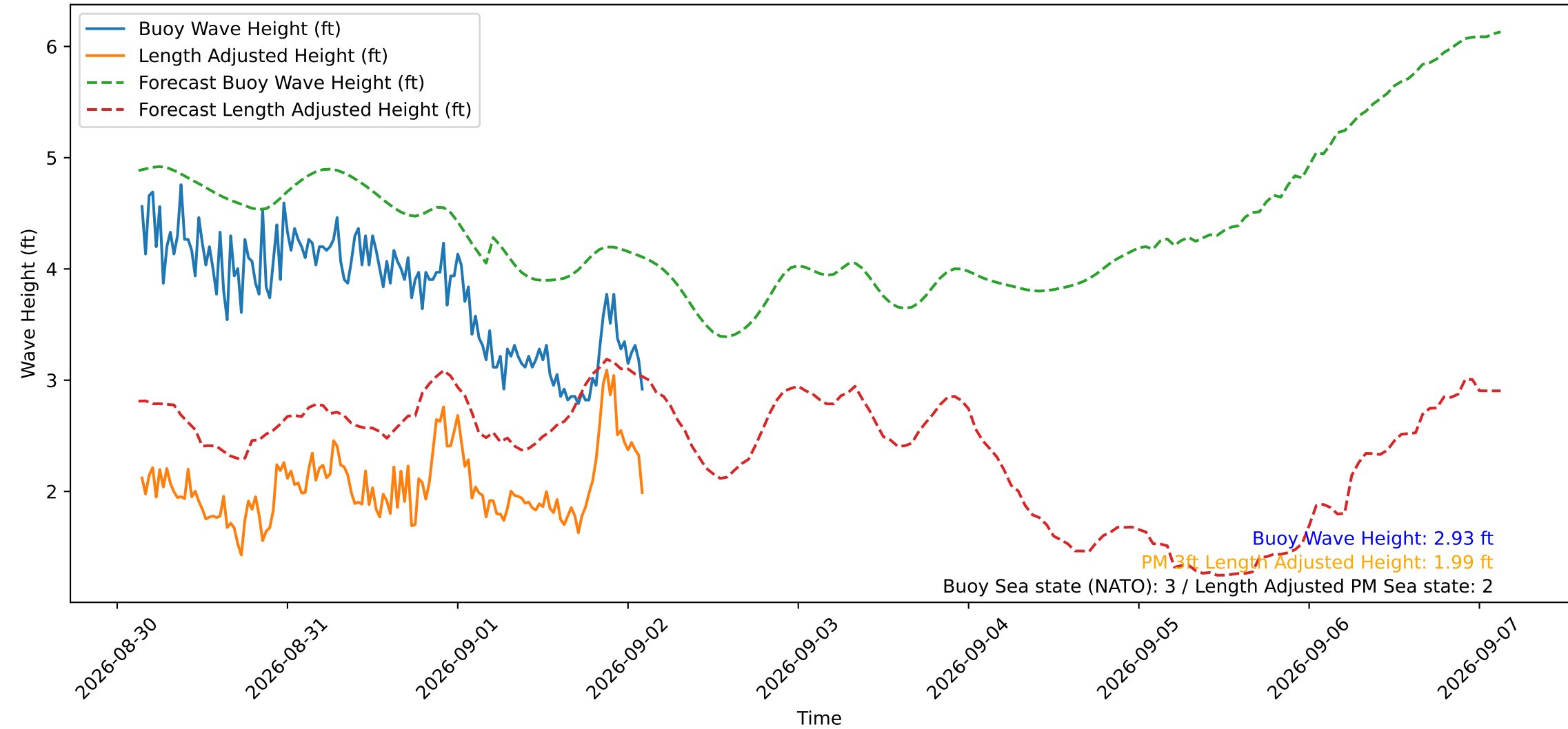
Wave Heights over Time for Green Beach at 2026-09-02 03:01:13
