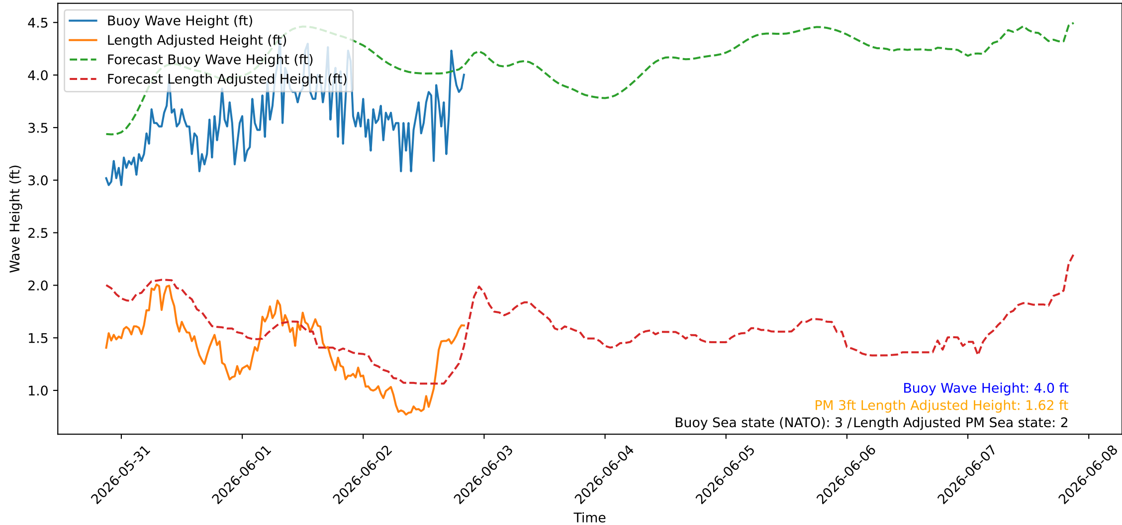
Wave Heights over Time for Green Beach at 2026-06-02 20:51:09
