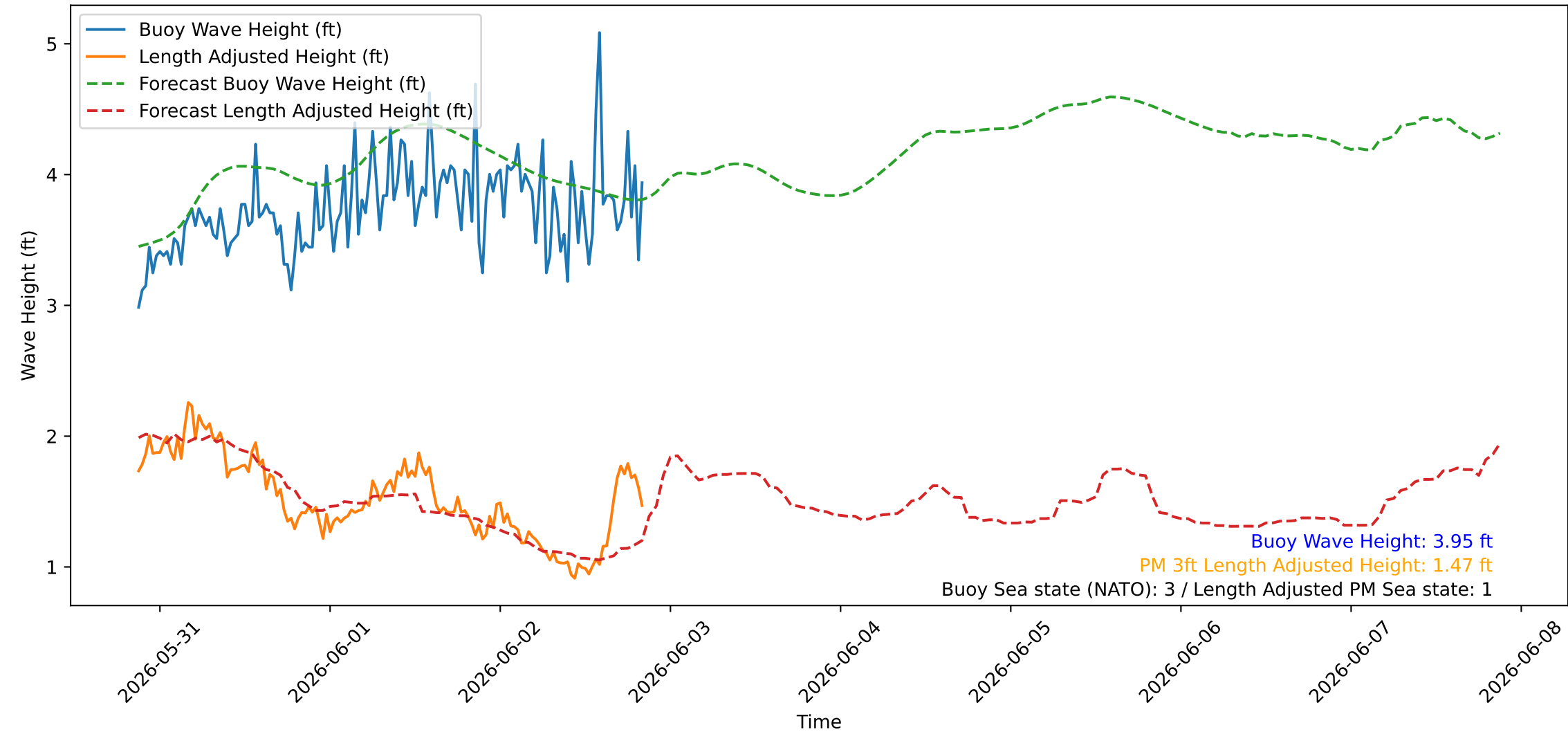
Wave Heights over Time for Oceanside Harbor at 2026-06-02 20:50:25
