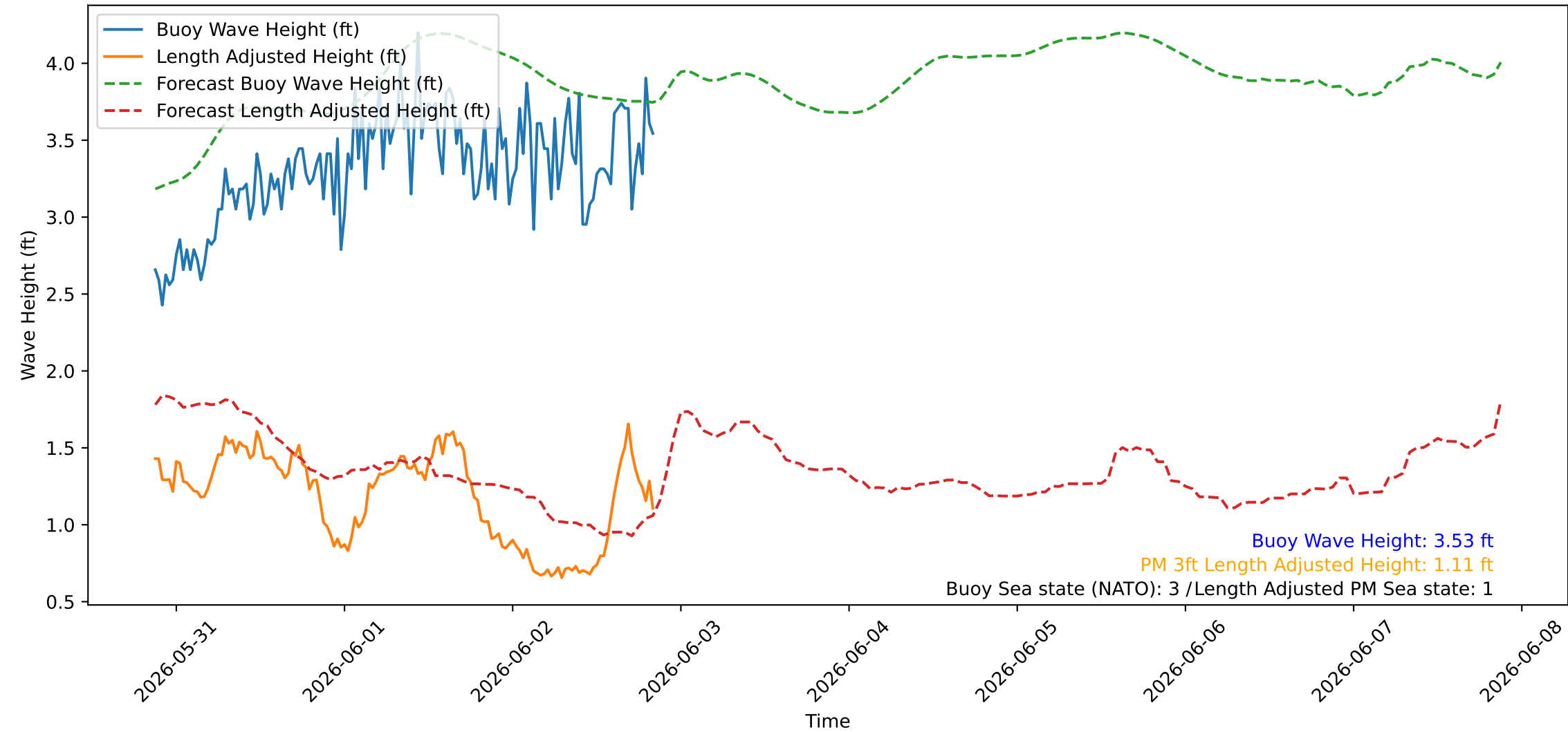
Wave Heights over Time for Red Beach at 2026-06-02 20:50:46
